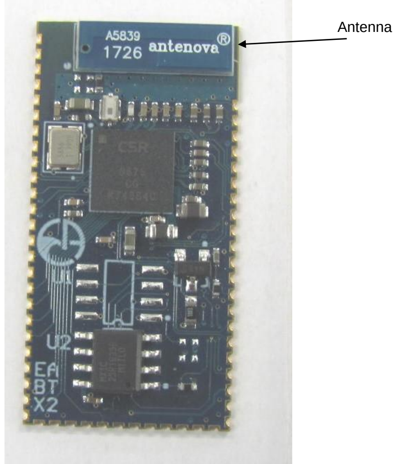
Photograph of PC Board: Component Side
