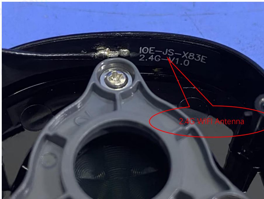
Photo 29 Internal of Antenna
