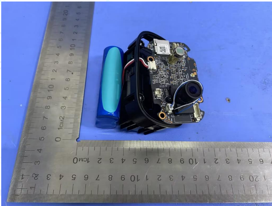
Photo 31 Internal of EUT
