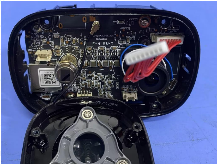
Photo 27 Internal of EUT
