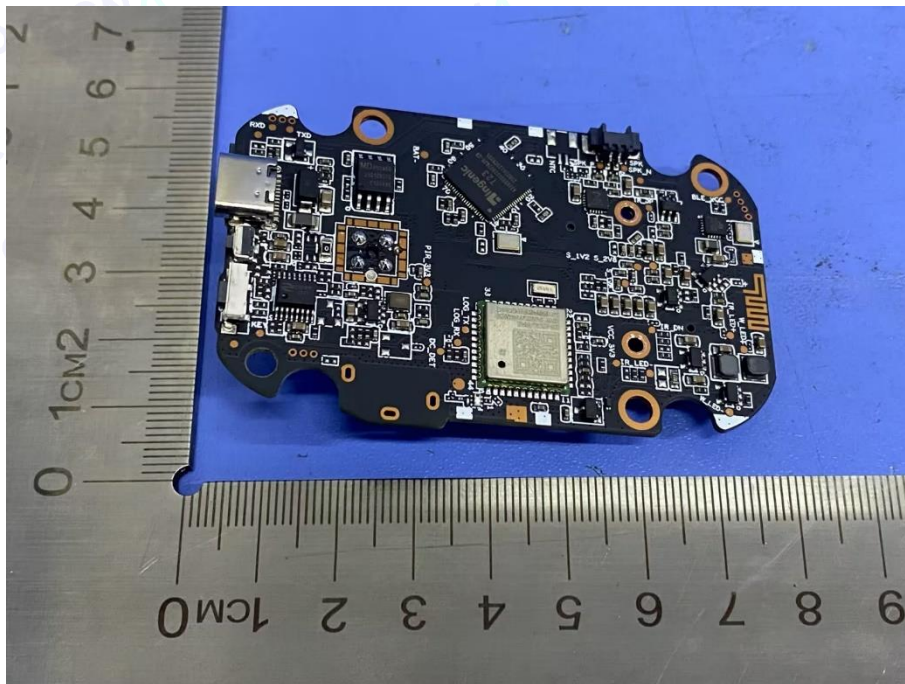
Photo 37 Appearance of PCB
