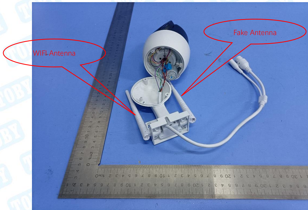
Photo 7 Internal of EUT
