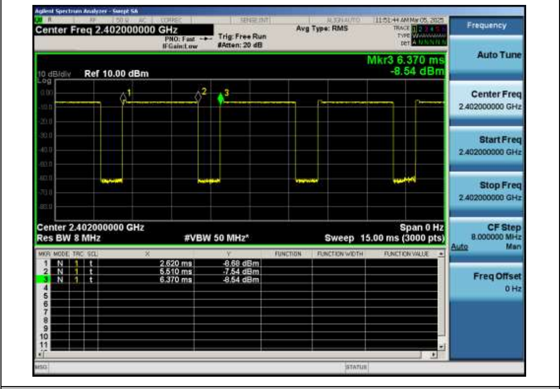
EDR-π /4-DQPSK-Ant1-2402
