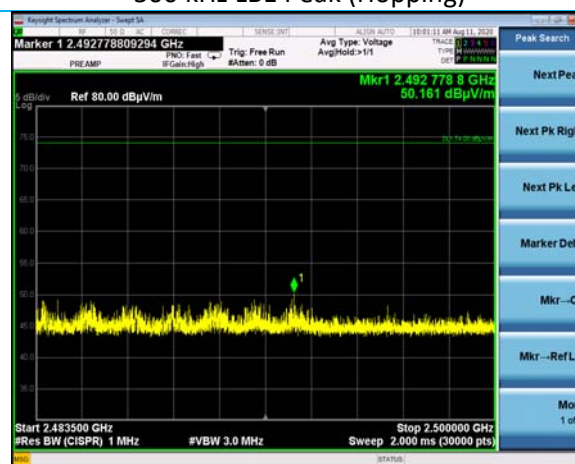
500 kHz UBE Peak (Hopping)
