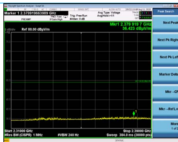
500 kHz LBE Average (Hopping)
