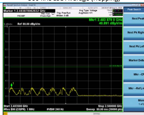
500 kHz UBE Average (Hopping)
