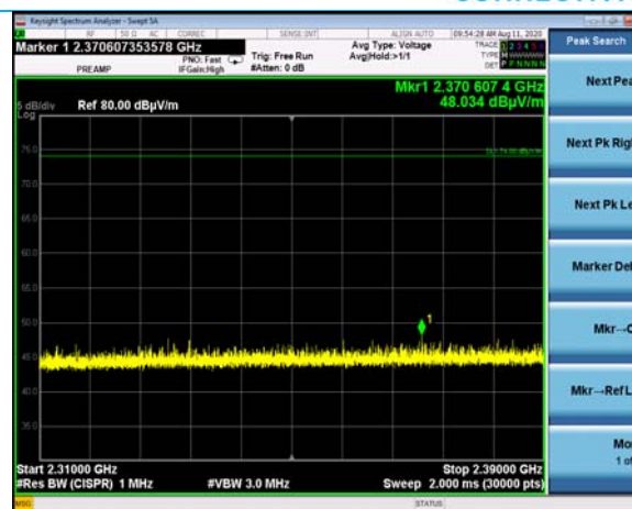
500 kHz LBE Peak (Hopping)
