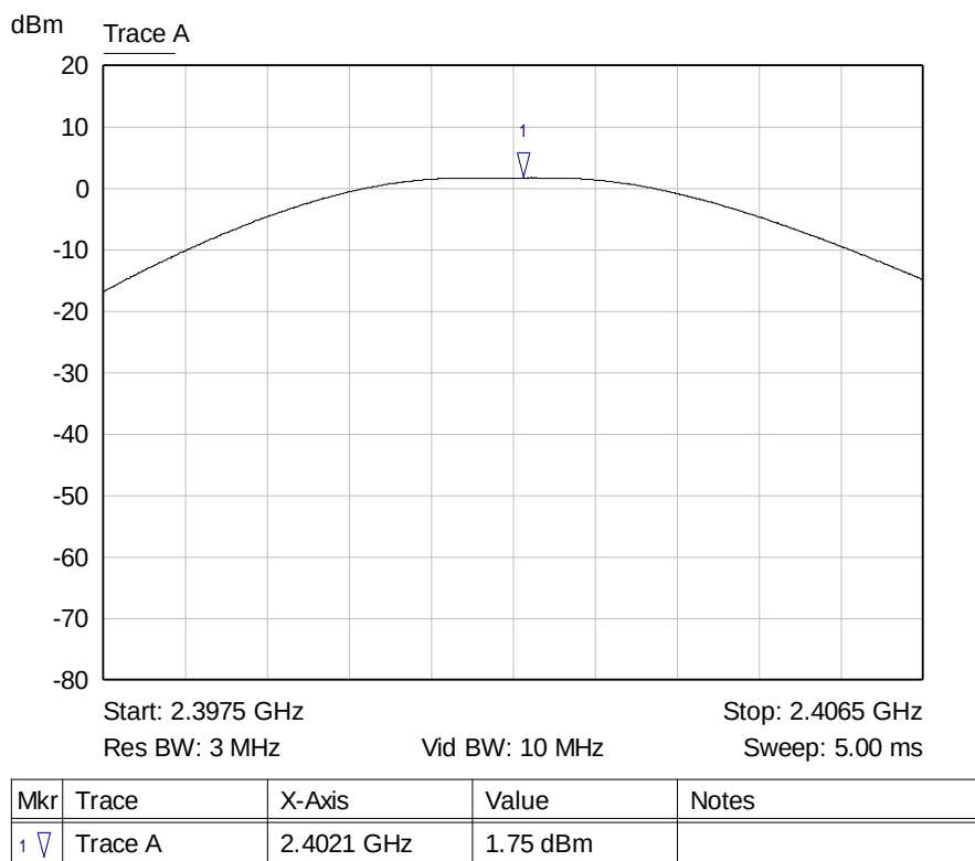
Graph 4: Lowest Channel Output Power Plot
