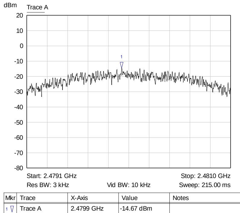
Graph 13: Highest Channel Output 3 kHz PSD Plot
