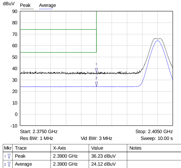
Graph 9: Radiated Lower Band Edge Plot
