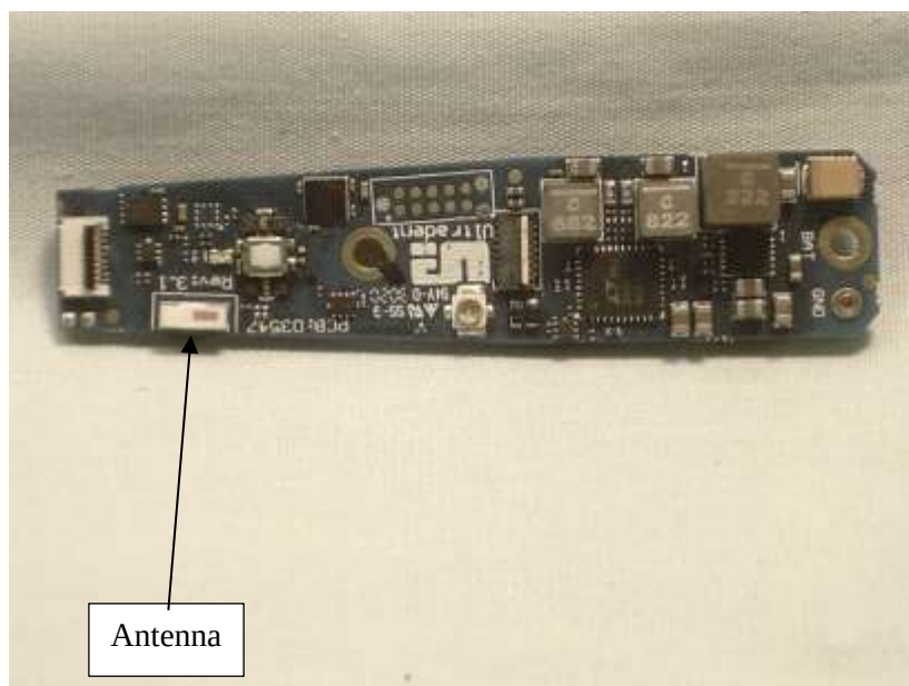
Photograph 19: Top Side of the PCB
