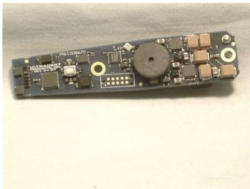
Photograph 20: Bottom Side of the PCB
