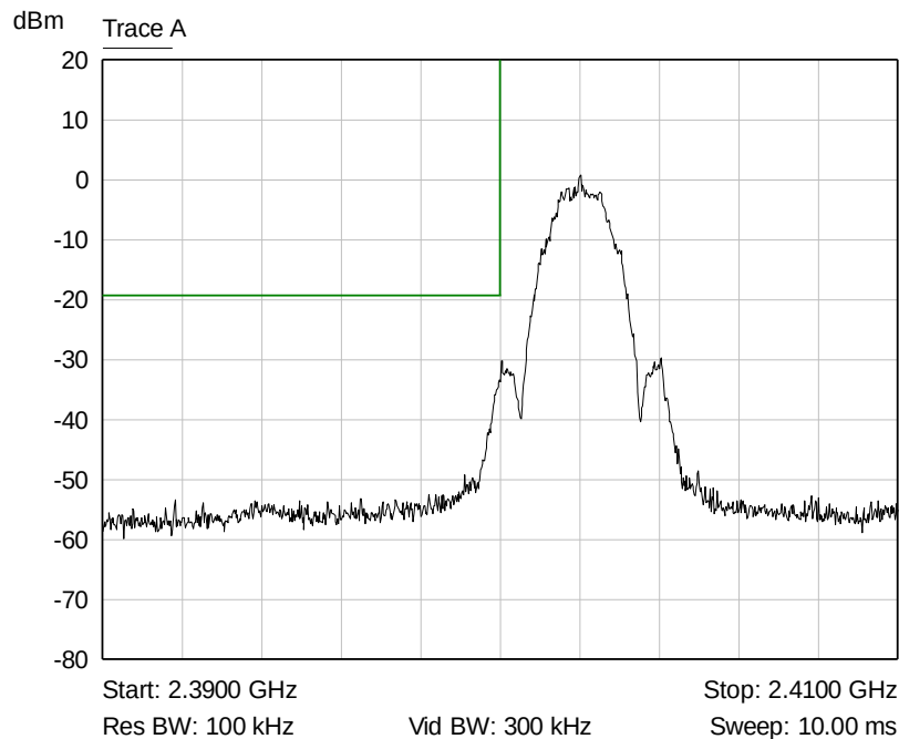
Graph 7: Lower Band Edge Plot
