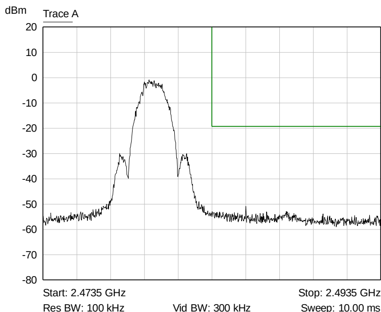
Graph 8: Upper Band Edge Plot
