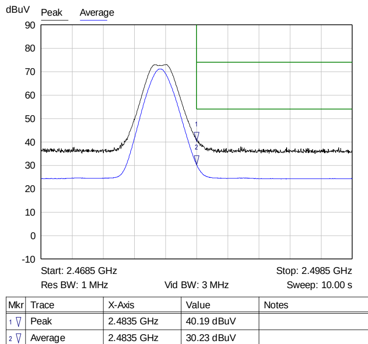
Graph 10: Radiated Upper Band Edge Plot
