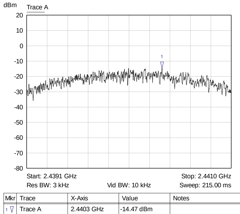
Graph 12: Middle Channel 3 kHz PSD Plot
