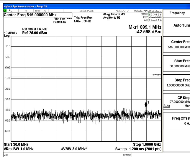
Band4-15MHz-QPSK-20325-1RB#0-Range4:1000~10000MHz
