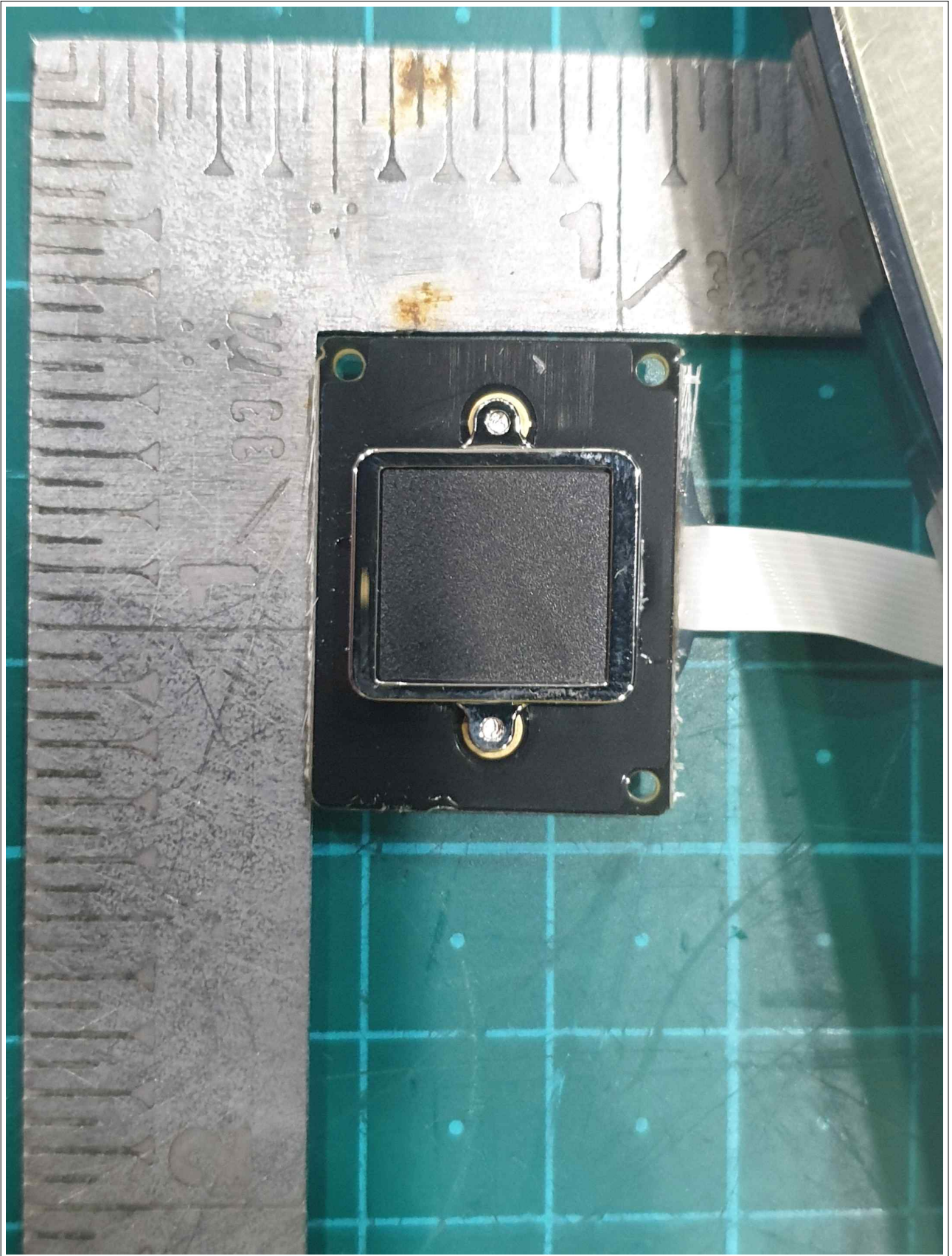
View of PCB 3 (Bottom)
