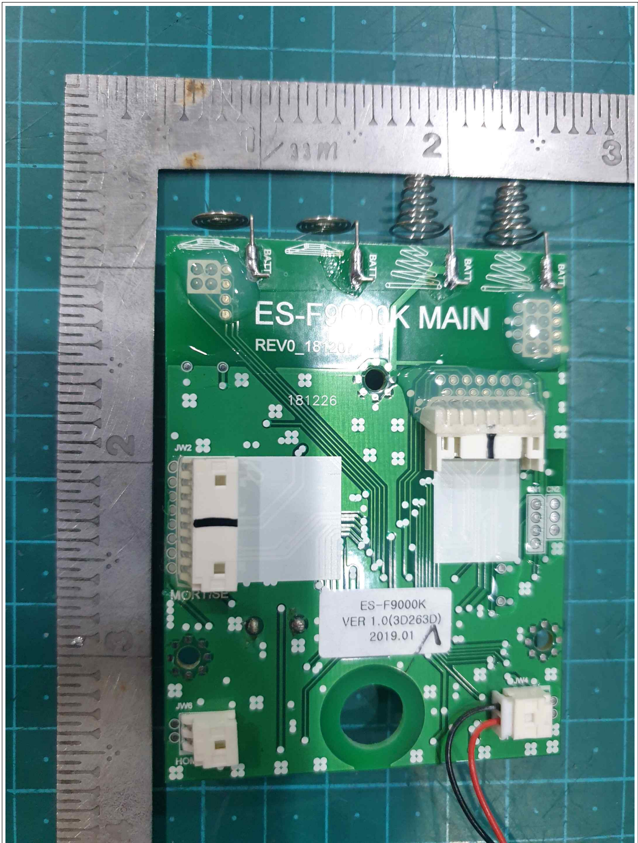
View of PCB 1 (Bottom)
