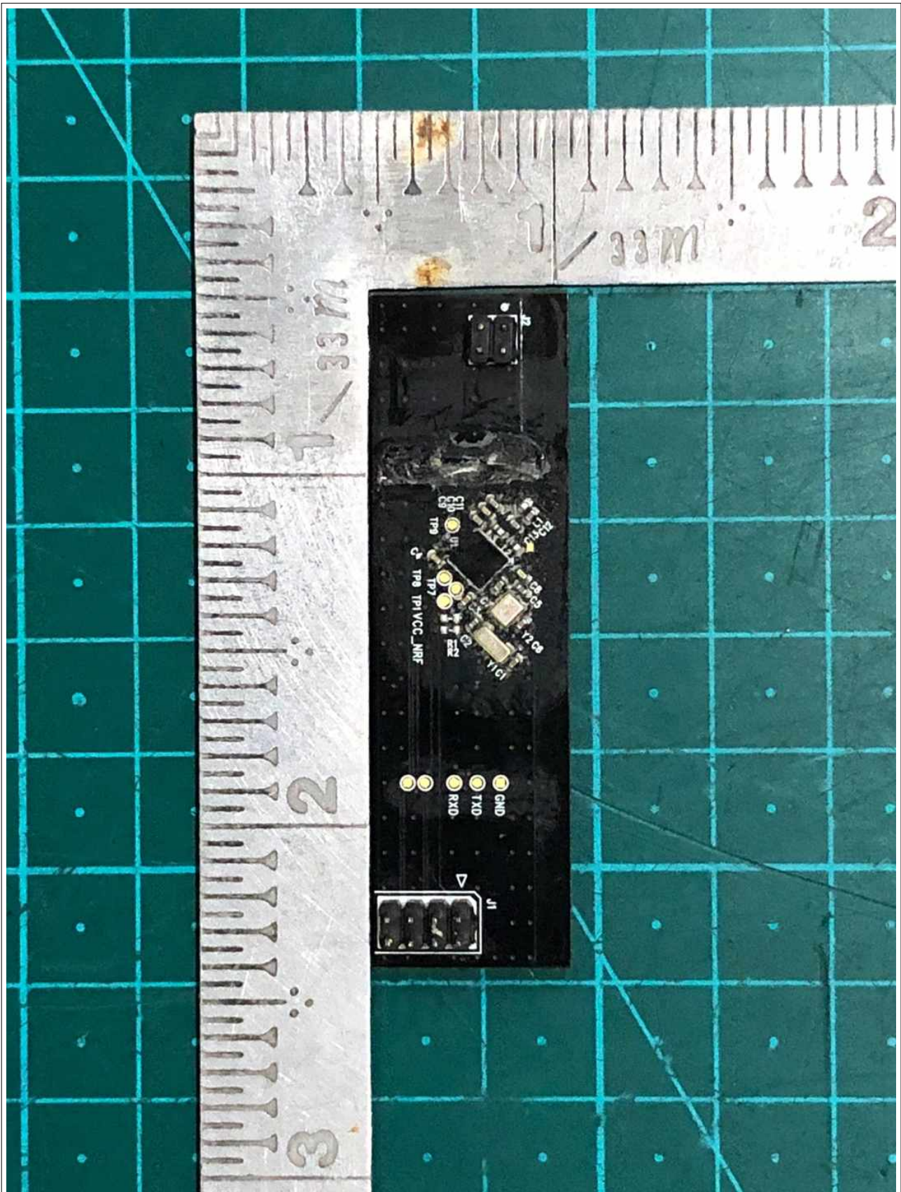
View of PCB 4 (Top)
