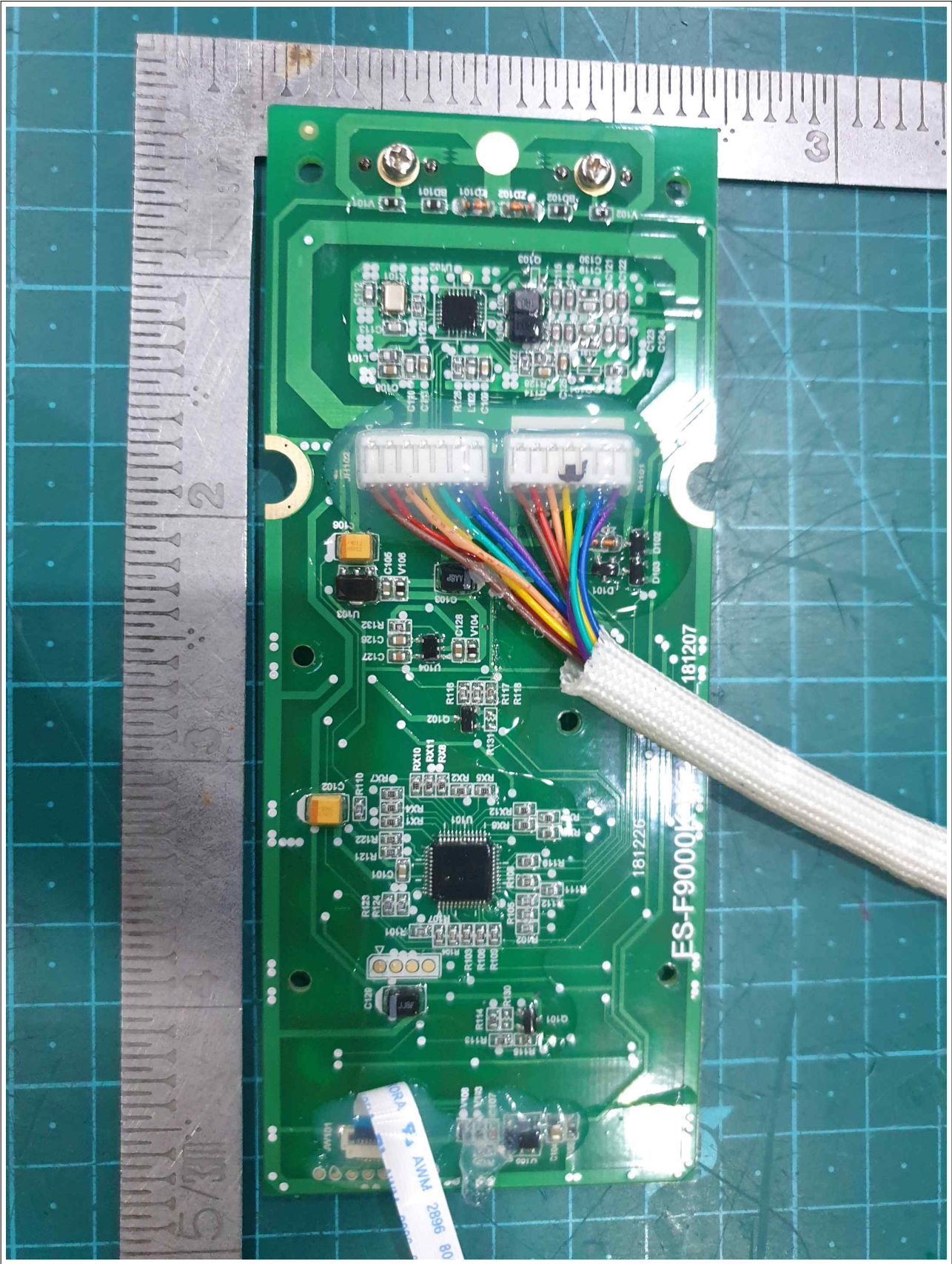
View of PCB 2 (Top)
