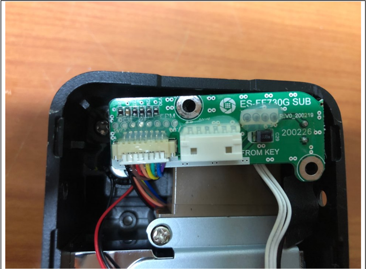
SubBoard-Rear
