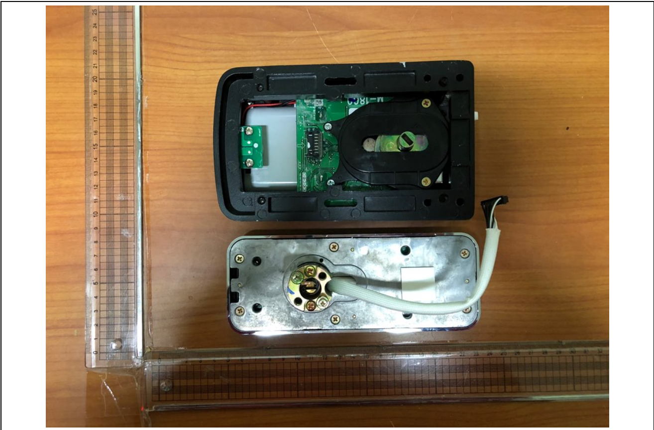
Rear
