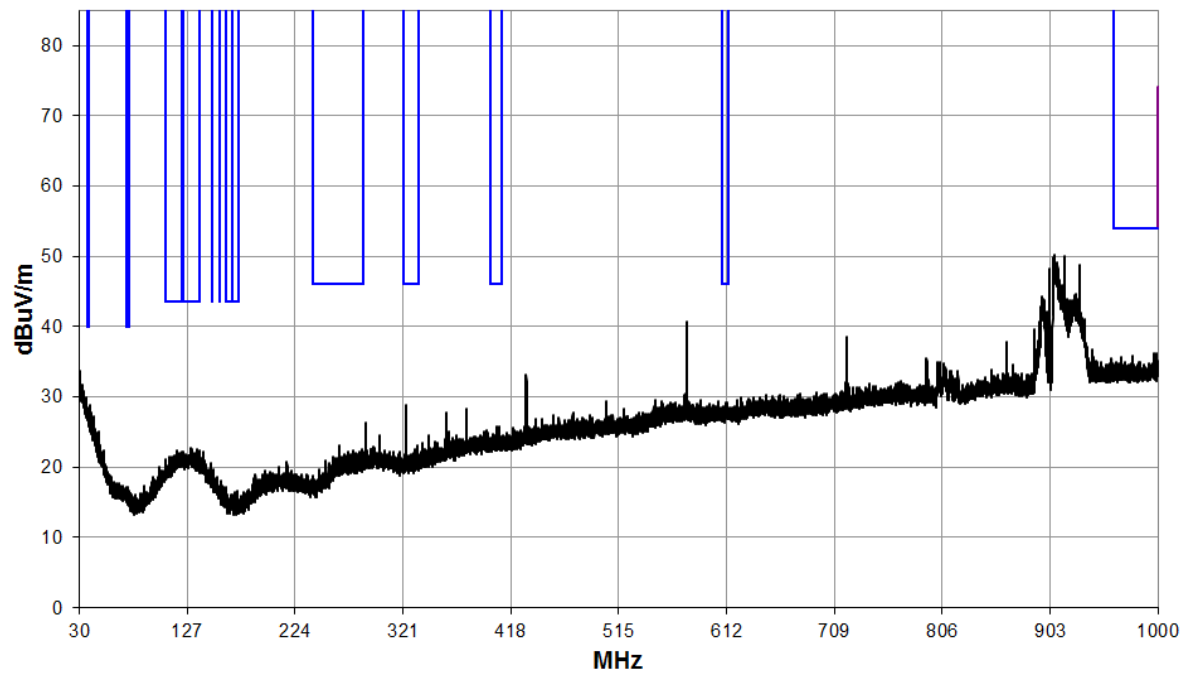
30 MHz to 1 GHz with Notch Filter
