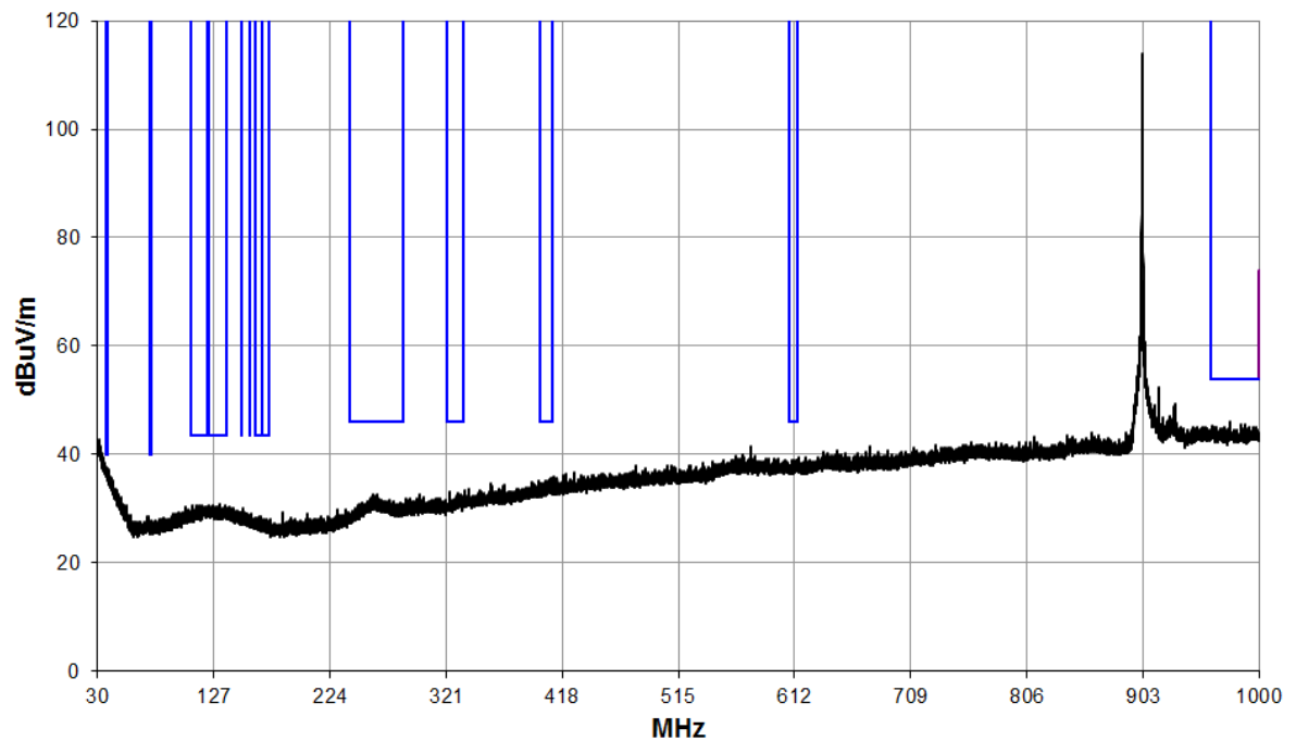
30 MHz to 1 GHz without Notch Filter
