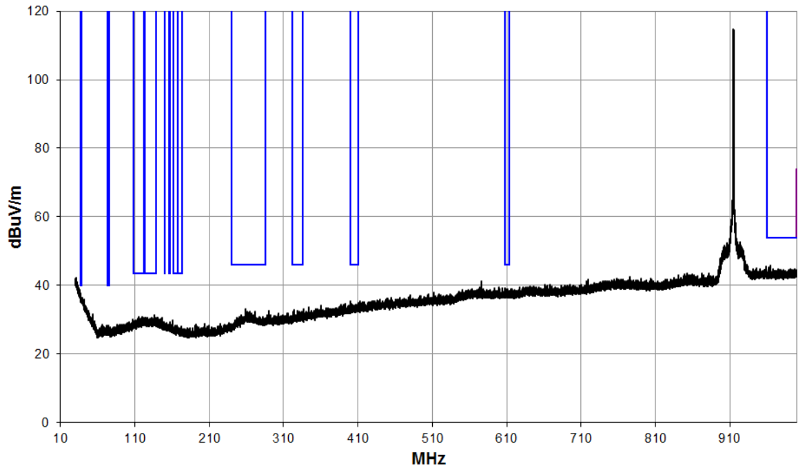
30 MHz to 1 GHz without Notch Filter
