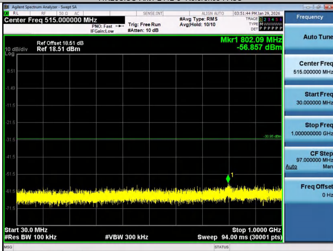
11N20SISO-Ant1-2412-30~1000-PASS
