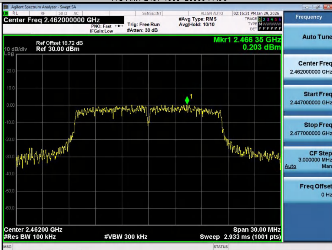
11G-Ant1-2462-0~Reference-PASS
