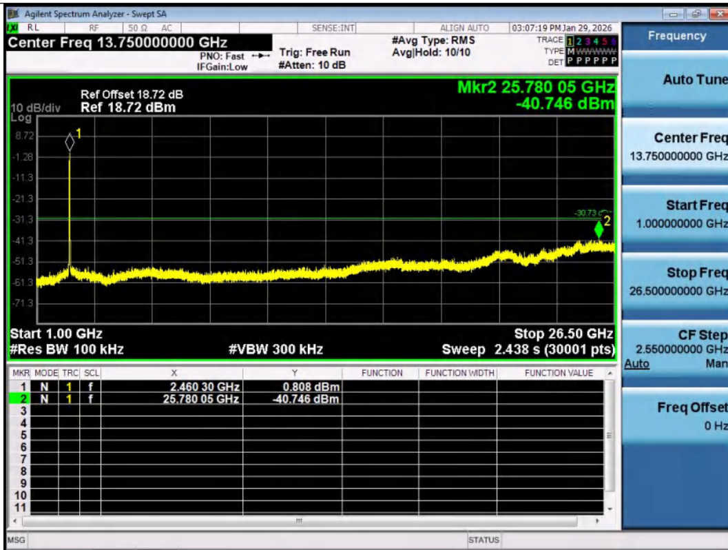
11N20SISO-Ant1-2462-1000~26500-PASS
