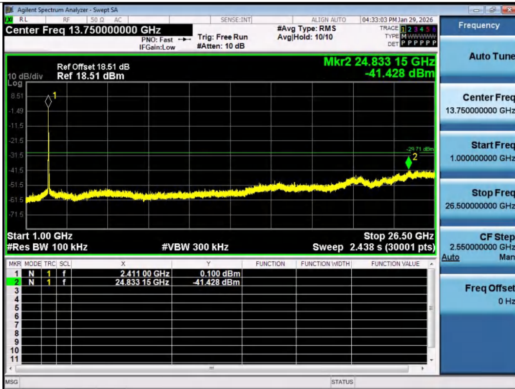
11AX20SISO-Ant1-2412-1000~26500-PASS
