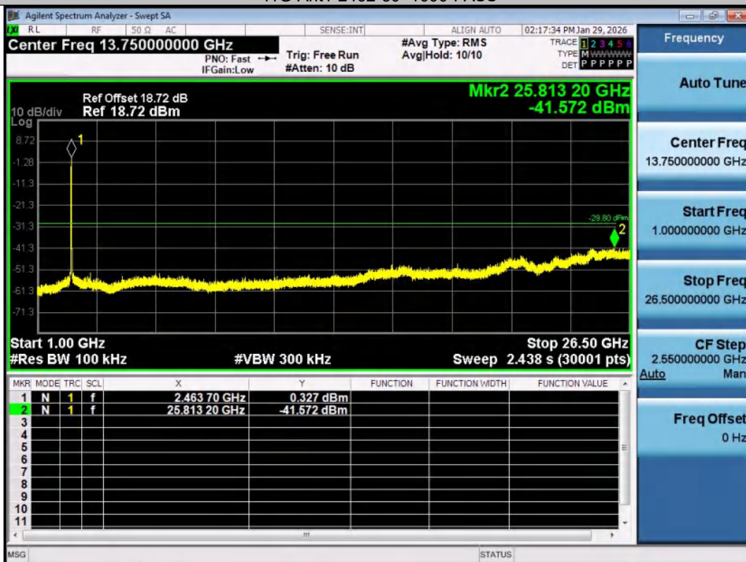
11G-Ant1-2462-1000~26500-PASS
