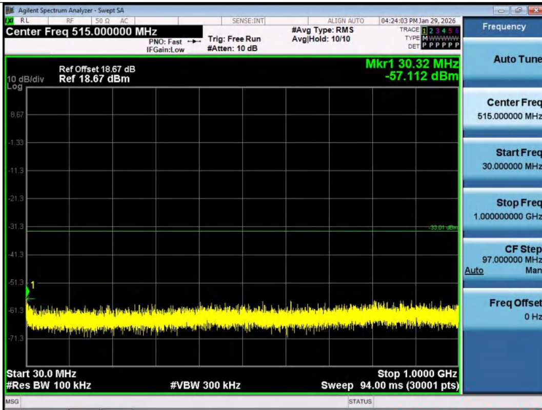
11N40SISO-Ant1-2452-30~1000-PASS
