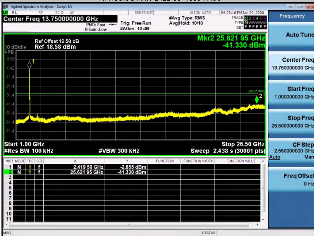
11N40SISO-Ant1-2422-1000~26500-PASS
