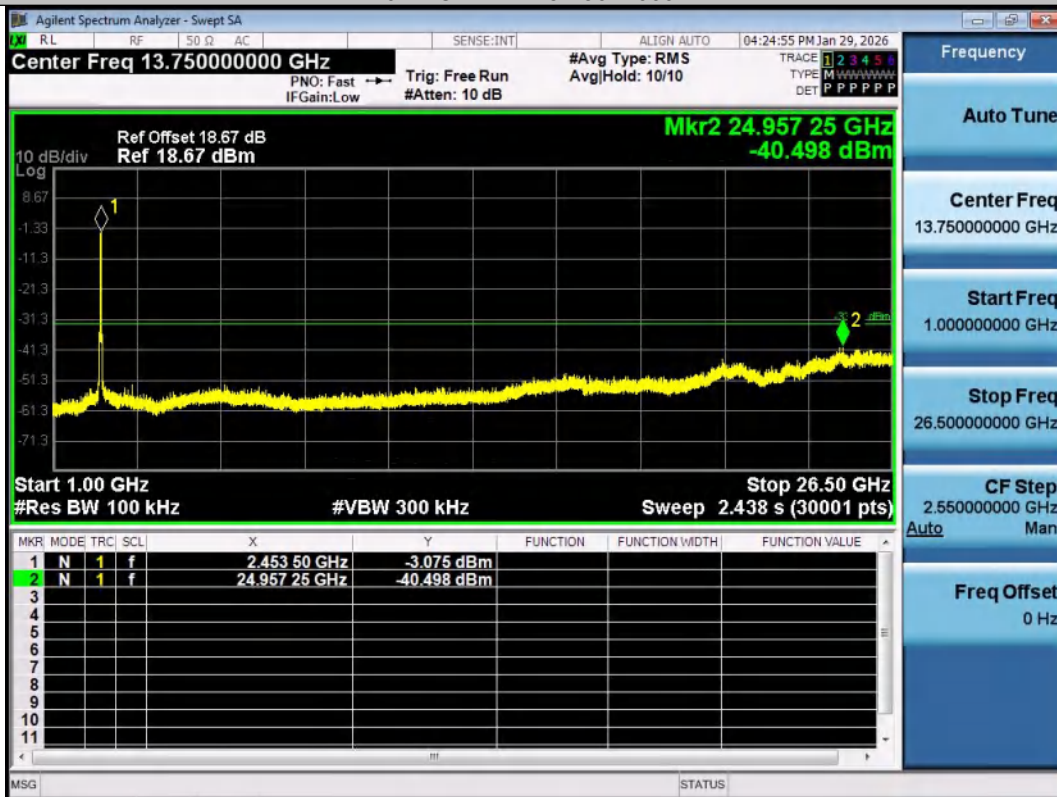
11N40SISO-Ant1-2452-1000~26500-PASS
