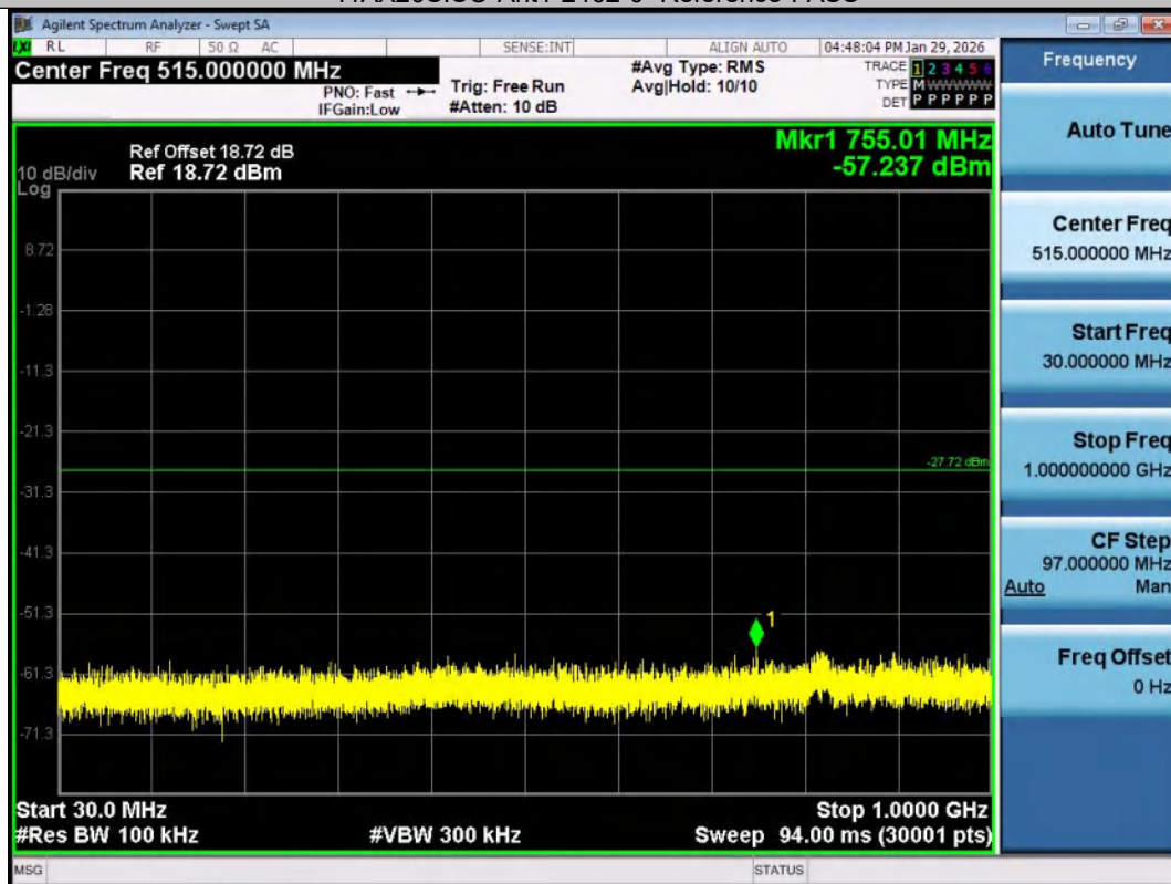
11AX20SISO-Ant1-2462-30~1000-PASS
