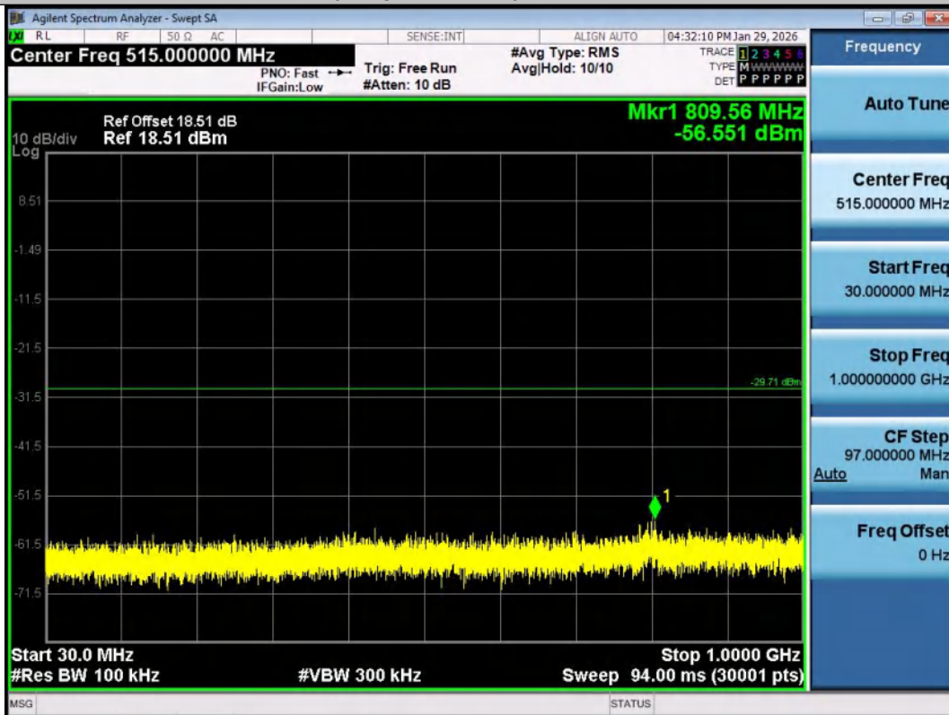
11AX20SISO-Ant1-2412-30~1000-PASS
