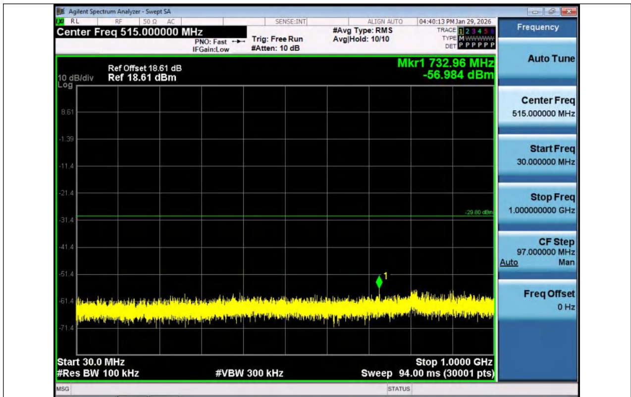
11AX20SISO-Ant1-2437-30~1000-PASS
