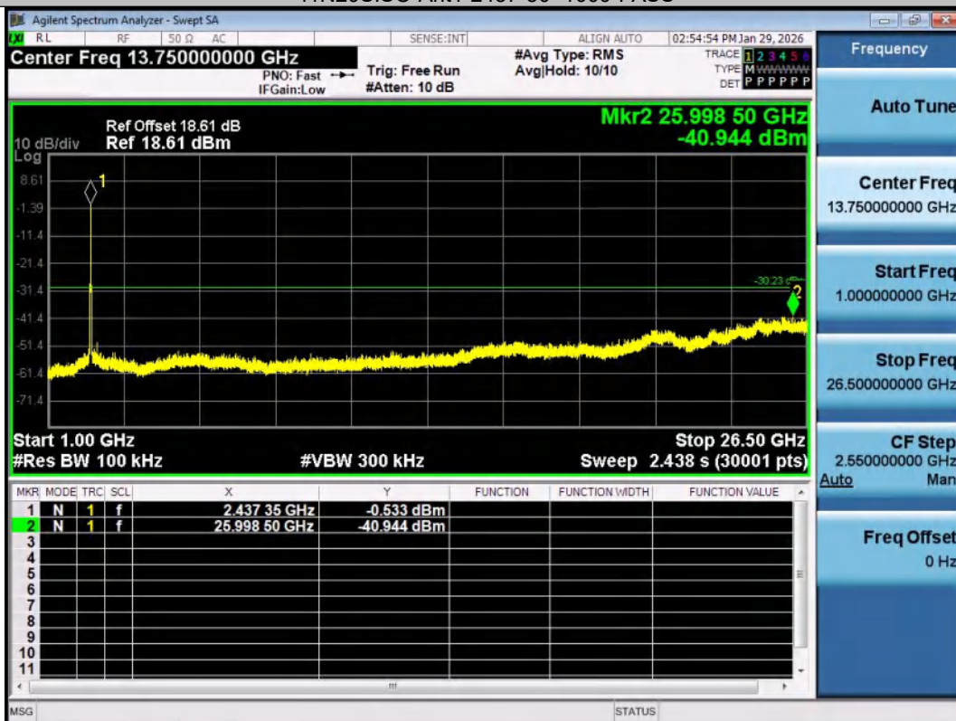
11N20SISO-Ant1-2437-1000~26500-PASS
