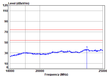
11g_TX_CH_11_Vertical
