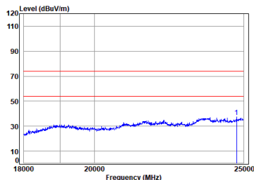
11g_TX_CH_06_Vertical
