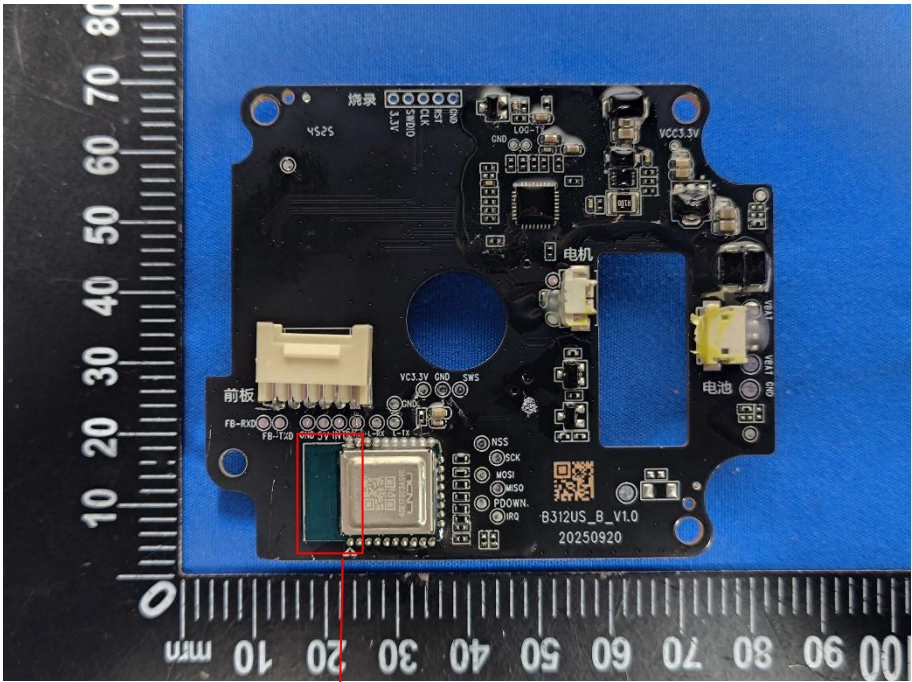
Back lock Bluetooth Ant.
