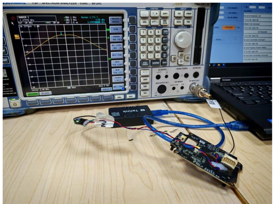
Radio Test Setup View (Back lock)
