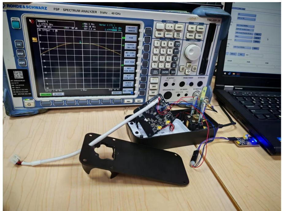
Radio Test Setup View (Front lock)
