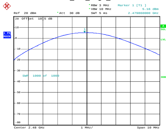
BLE_1M_High_Channel
