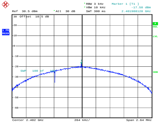
BLE_2M_Low_Channel
