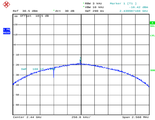
BLE_2M_Middle_Channel
