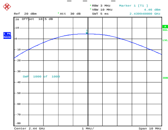
BLE_2M_Middle_Channel
