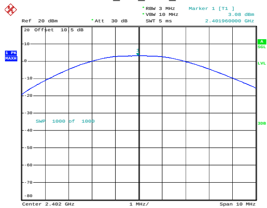
BLE_2M_Low_Channel
