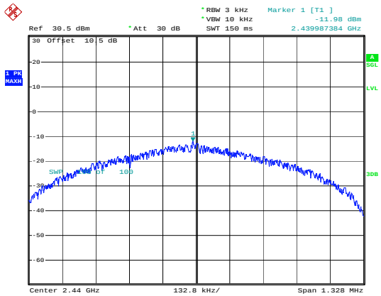
BLE_1M_Middle_Channel
