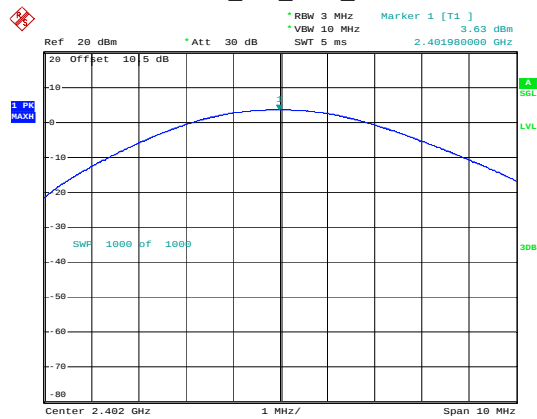
BLE_1M_Low_Channel
