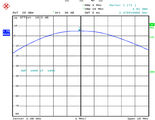
BLE_2M_High_Channel
