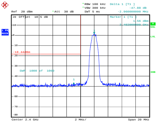
BLE_1M_Low_Channel
