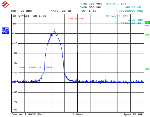
BLE_2M_High_Channel
