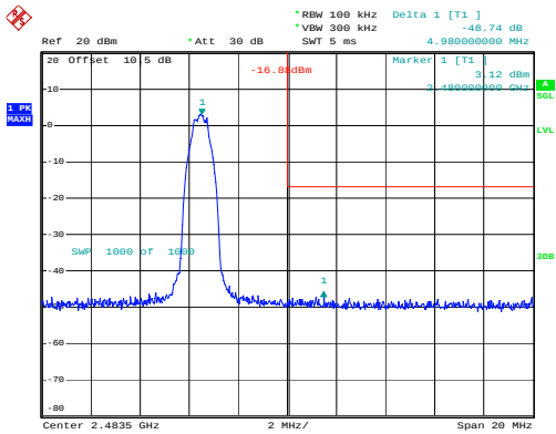
BLE_1M_High_Channel
