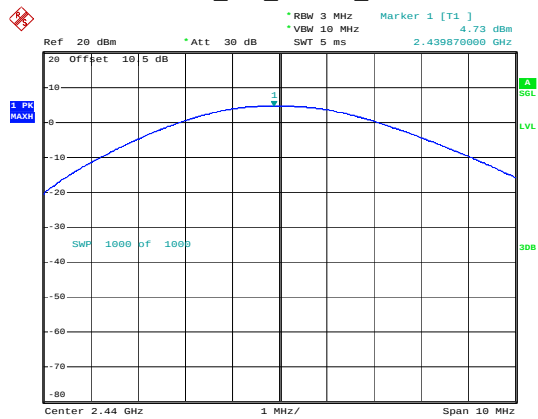
BLE_1M_Middle_Channel
