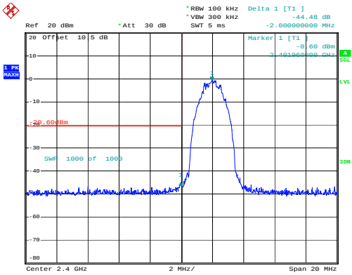
BLE_2M_Low_Channel
