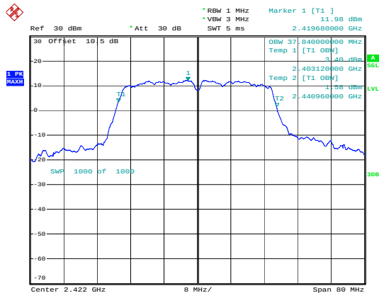
802.11n40_2422MHz
