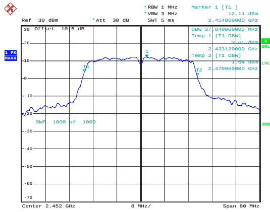
802.11n40_2452MHz
