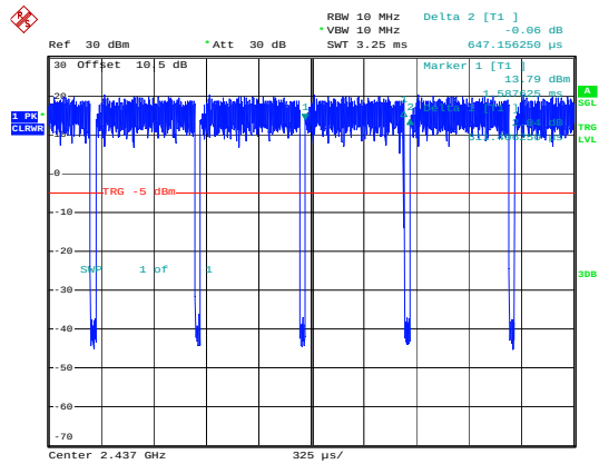
802.11n40_2437MHz
