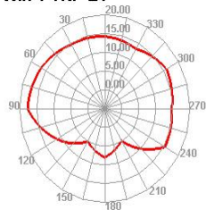
Wifi 7 TRP
