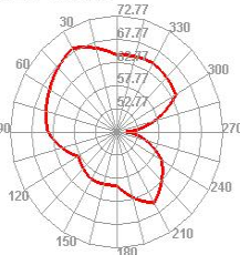
Wifi 7 TIS H
