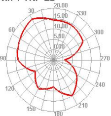
Wifi 7 TRP H
