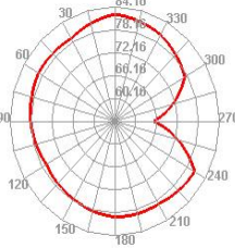
Wifi 1 TIS H
