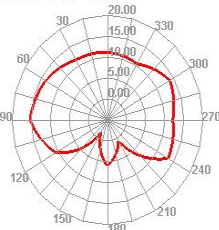
Wifi 7 TRP
