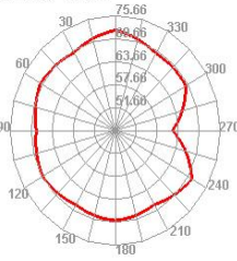
Wifi 13 TIS H
