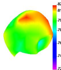
Wifi 1 TIS
