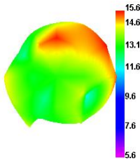
Wifi 1 TRP
