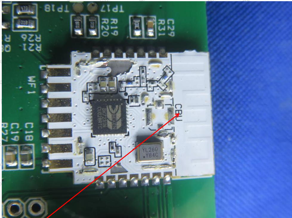
WIFI ANT
