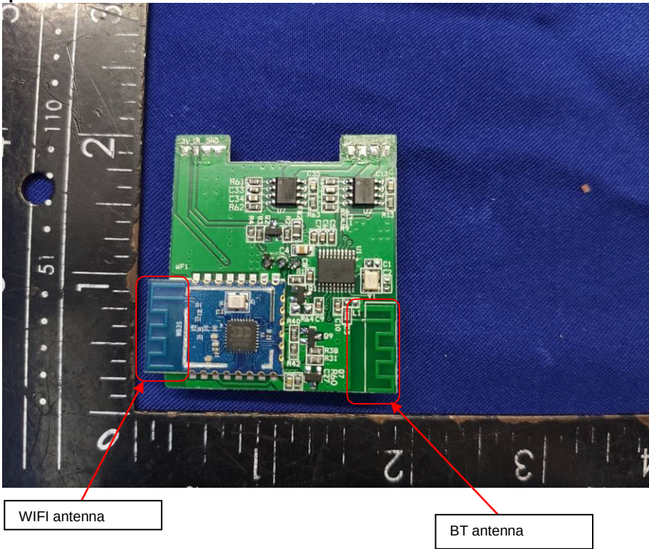
Solder Board-Component View 7
