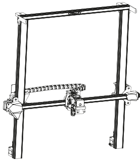
2 Gantry Frame Assembly
