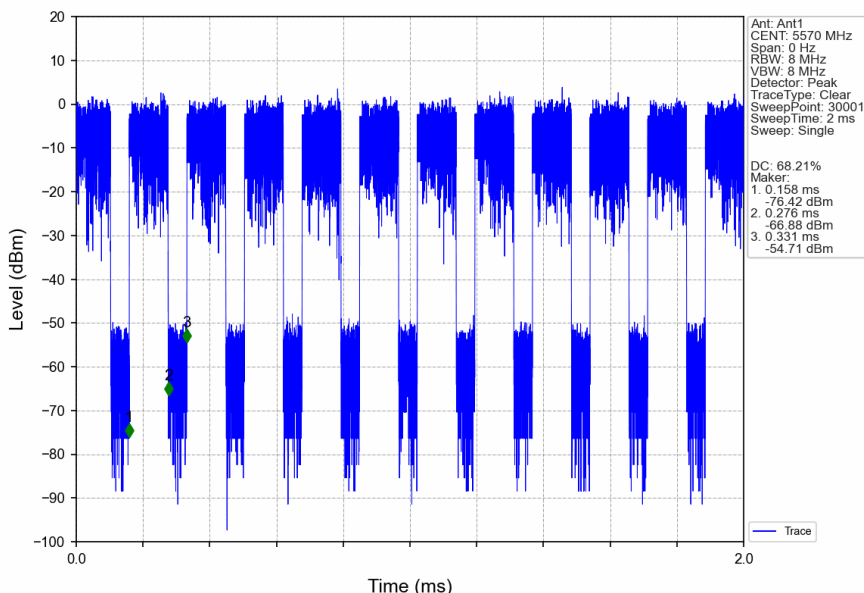
802.11ac(VHT160)_MCH_5570MHz_Ant1_NTNV
