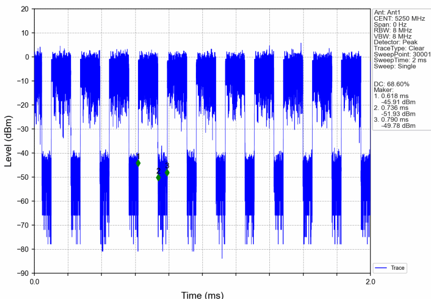
802.11ac(VHT160)_MCH_5250MHz_Ant1_NTNV
