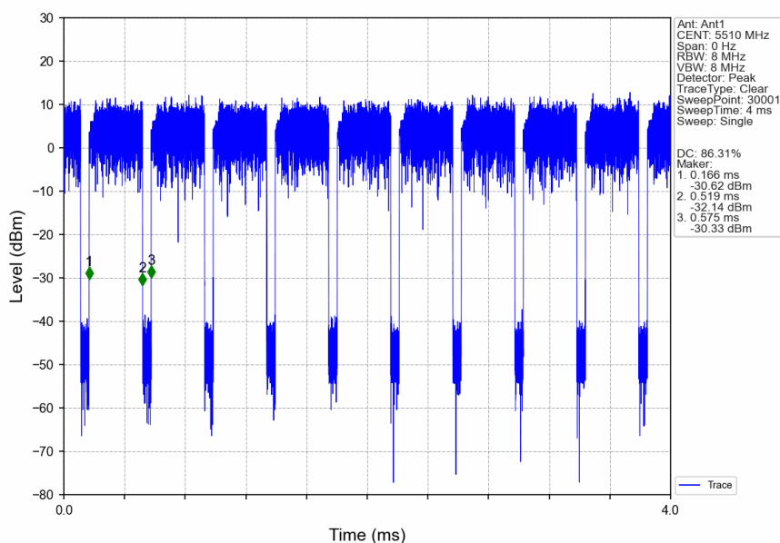
802.11ac(VHT40)_LCH_5510MHz_Ant1_NTNV
