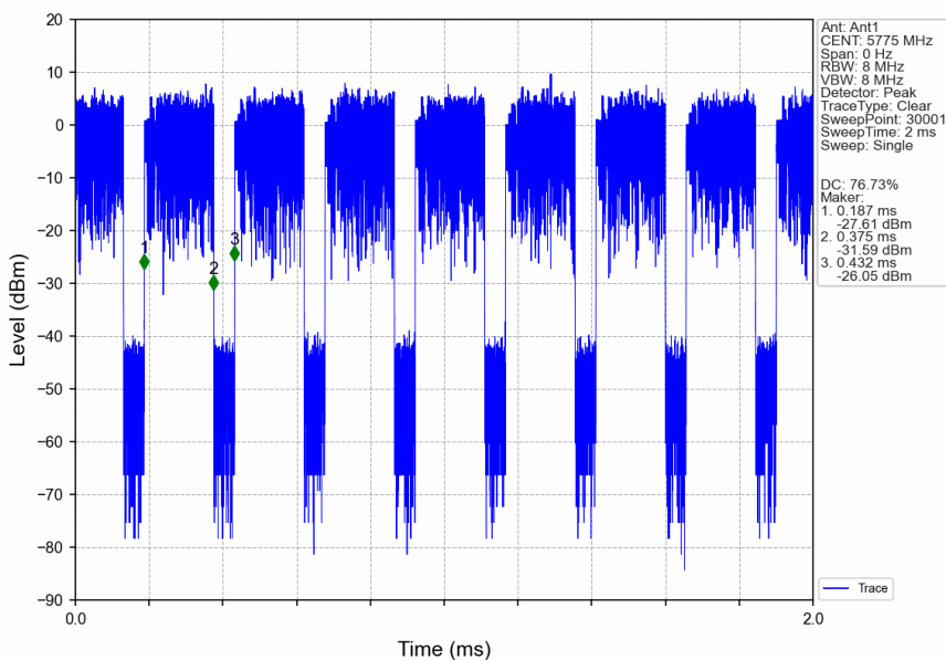
802.11ac(VHT80)_MCH_5775MHz_Ant1_NTNV
