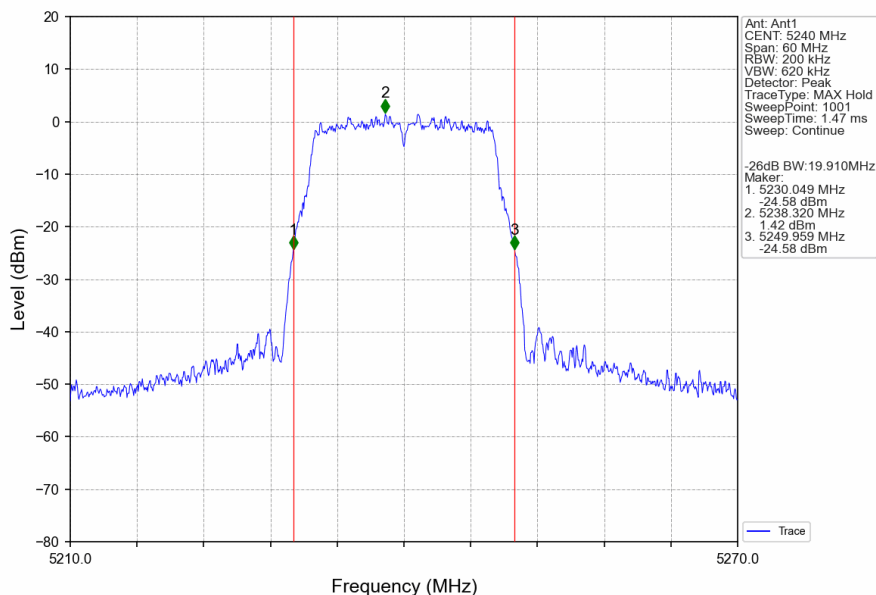
802.11a_HCH_5240MHz_Ant1_NTNV
