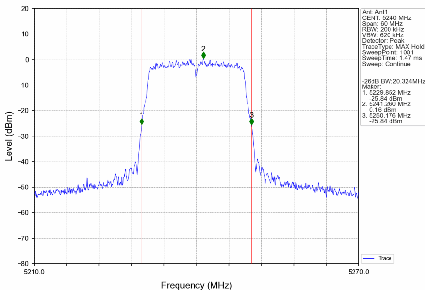
802.11ac(VHT20)_HCH_5240MHz_Ant1_NTNV
