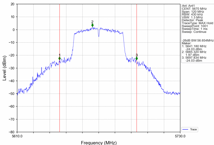
802.11n(HT40)_HCH_5670MHz_Ant1_NTNV
