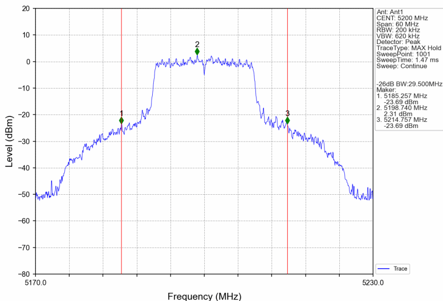
802.11n(HT20)_MCH_5200MHz_Ant1_NTNV
