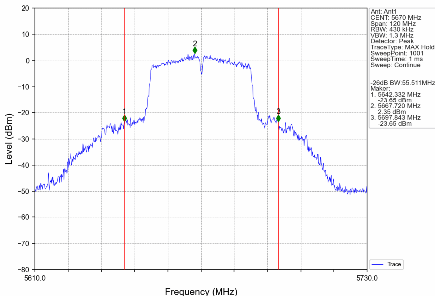
802.11ac(VHT40)_HCH_5670MHz_Ant1_NTNV
