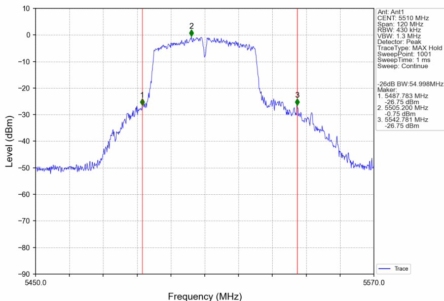
802.11ac(VHT40)_LCH_5510MHz_Ant1_NTNV
