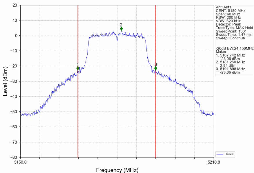
802.11ac(VHT20)_LCH_5180MHz_Ant1_NTNV
