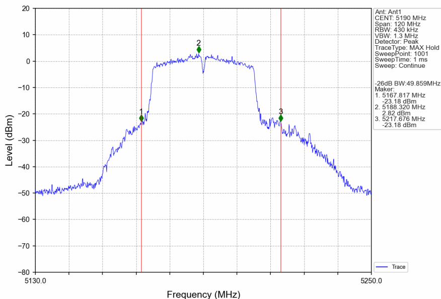
802.11ac(VHT40)_LCH_5190MHz_Ant1_NTNV
