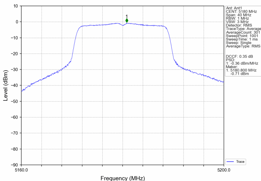
802.11ac(VHT20)_LCH_5180MHz_Ant1_NTNV
