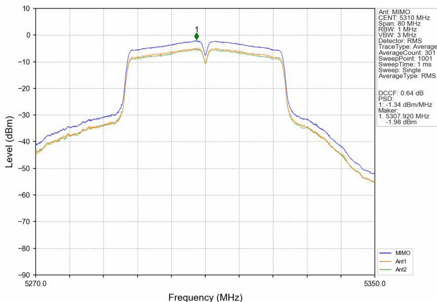
802.11n(HT40)_HCH_5310MHz_MIMO_NTNV
