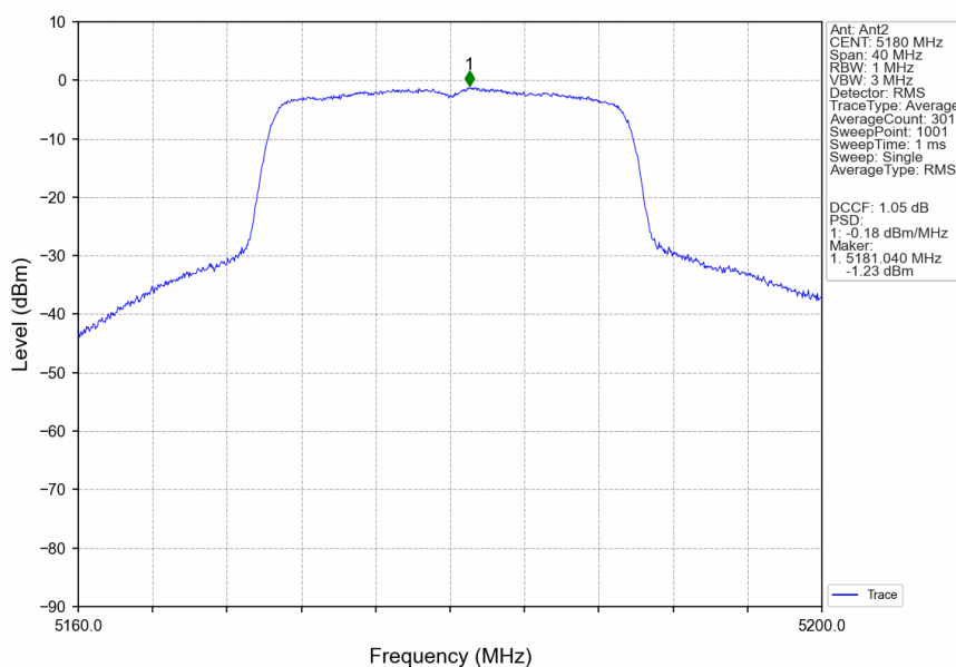
802.11ax(HEW20)_LCH_5180MHz_SU_ / _Ant2_NTNV
