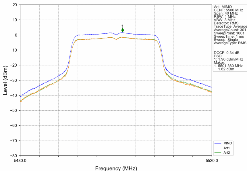
802.11ac(VHT20)_LCH_5500MHz_MIMO_NTNV
