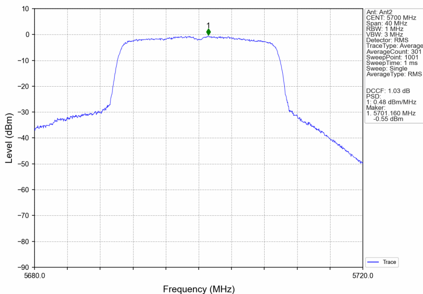
802.11ax(HEW20)_HCH_5700MHz_SU_/_Ant2_NTNV
