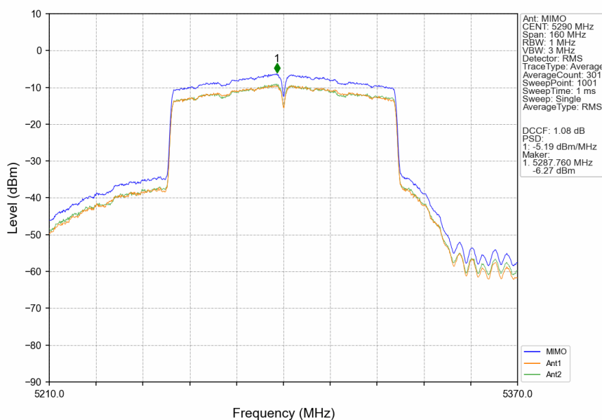
802.11ac(VHT80)_MCH_5290MHz_MIMO_NTNV
