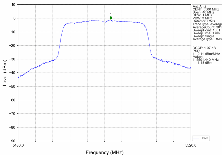
802.11ax(HEW20)_LCH_5500MHz_SU_ / _Ant2_NTNV
