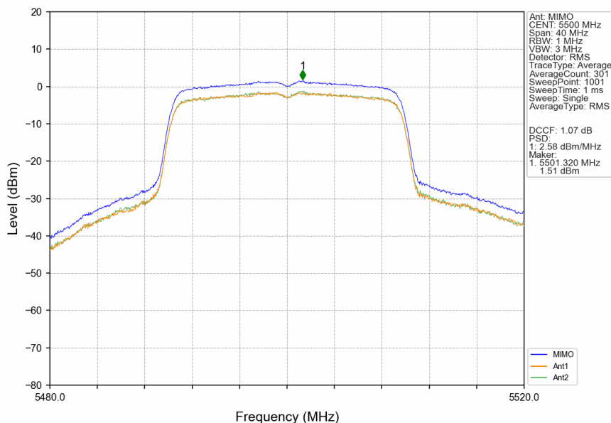
802.11ax(HEW20)_LCH_5500MHz_SU_/_MIMO_NTNV
