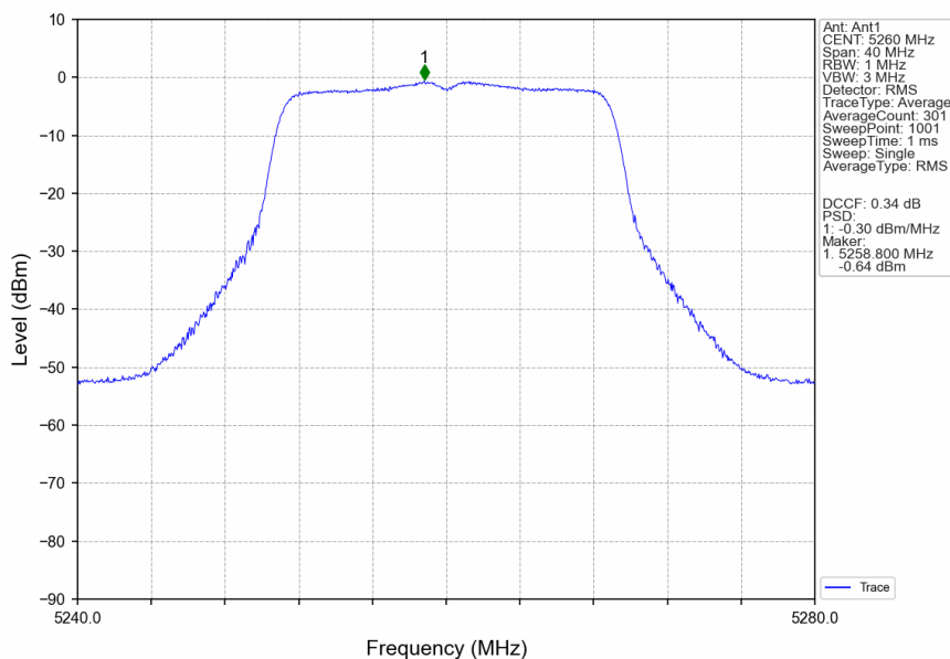
802.11ac(VHT20)_LCH_5260MHz_Ant1_NTNV
