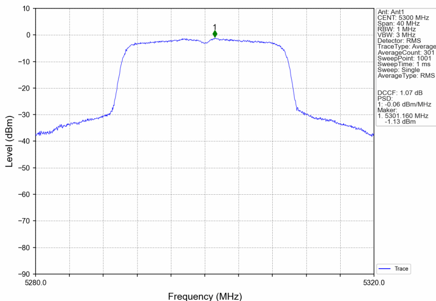
802.11ax(HEW20)_MCH_5300MHz_SU_/_Ant1_NTNV
