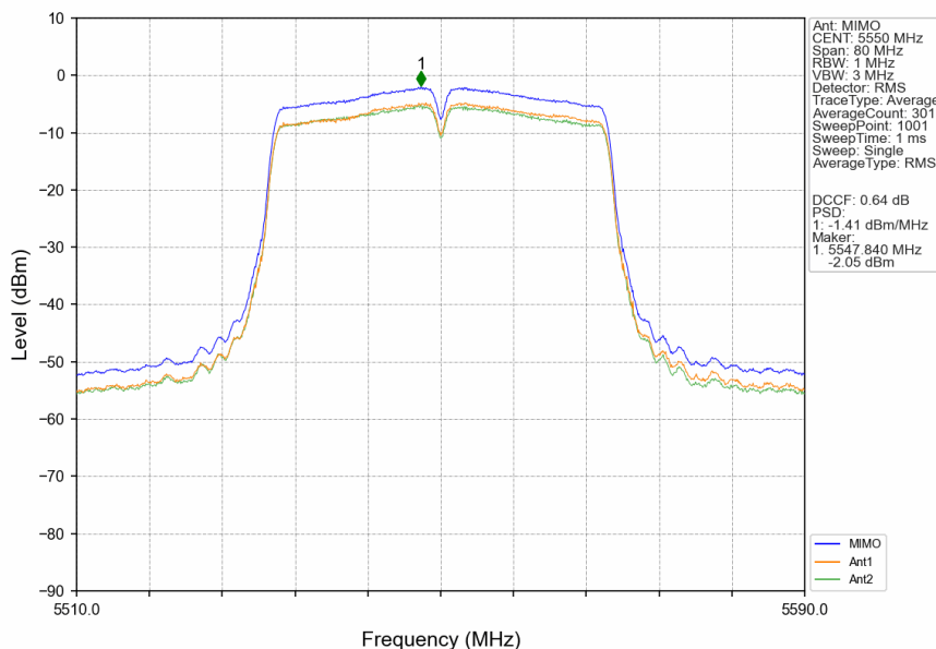
802.11ac(VHT40)_MCH_5550MHz_MIMO_NTNV
