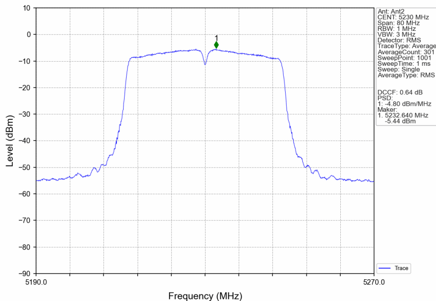
802.11ac(VHT40)_HCH_5230MHz_Ant2_NTNV
