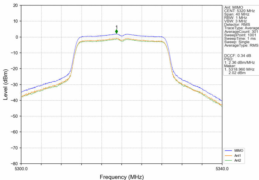
802.11ac(VHT20)_HCH_5320MHz_MIMO_NTNV
