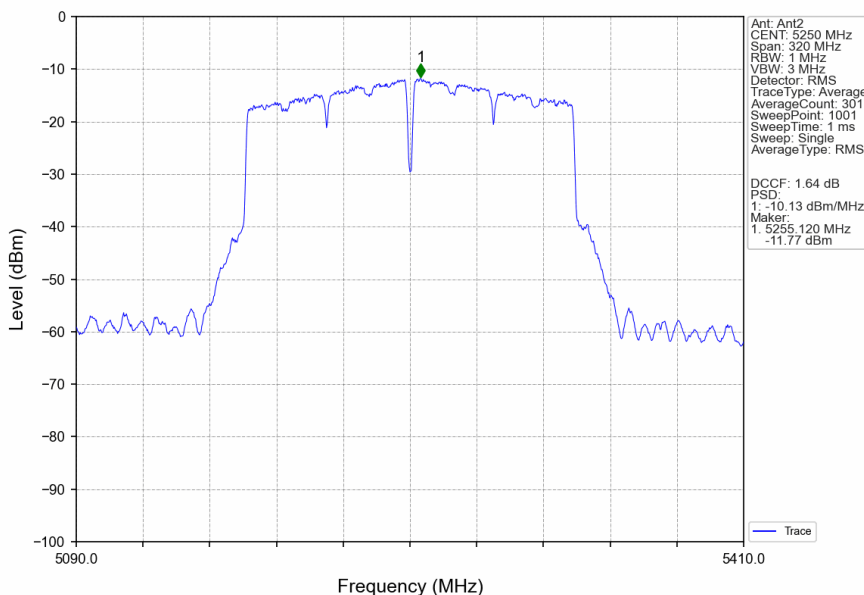
802.11ac(VHT160)_MCH_5250MHz_Ant2_NTNV
