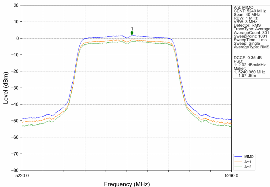
802.11ac(VHT20)_HCH_5240MHz_MIMO_NTNV
