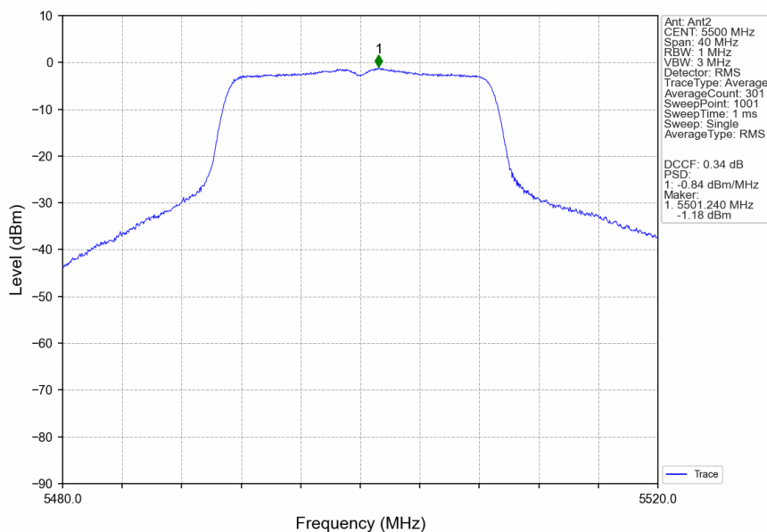
802.11ac(VHT20)_LCH_5500MHz_Ant2_NTNV
