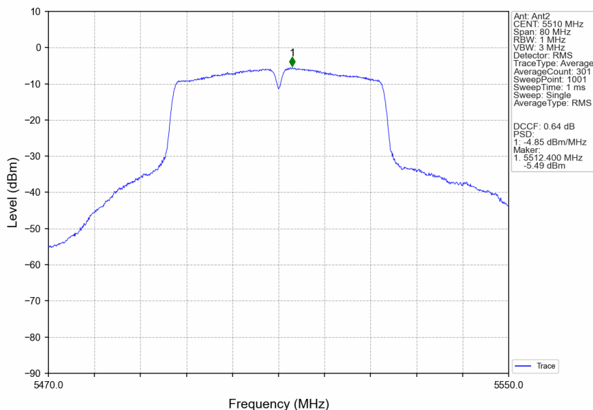
802.11ac(VHT40)_LCH_5510MHz_Ant2_NTNV
