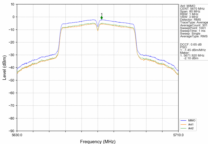
802.11ac(VHT40)_HCH_5670MHz_MIMO_NTNV
