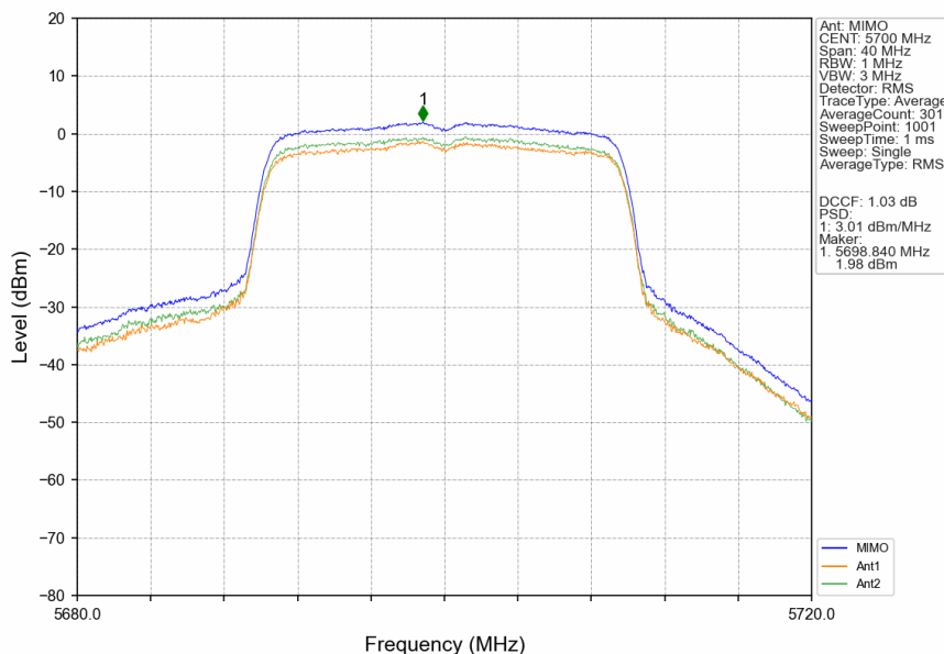
802.11ax(HEW20)_HCH_5700MHz_SU_/_MIMO_NTNV
