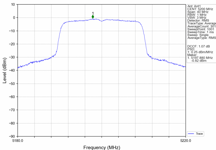
802.11ax(HEW20)_MCH_5200MHz_SU_/_Ant1_NTNV
