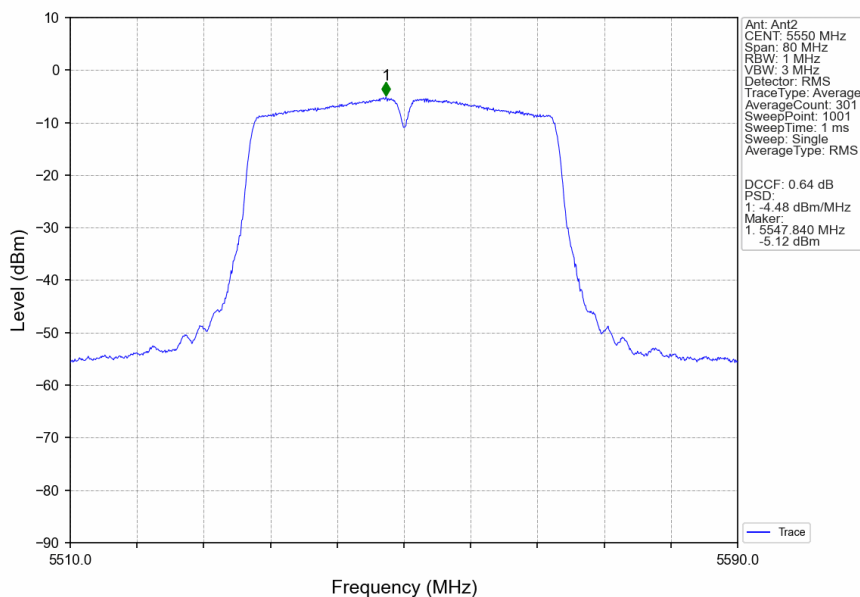
802.11ac(VHT40)_MCH_5550MHz_Ant2_NTNV
