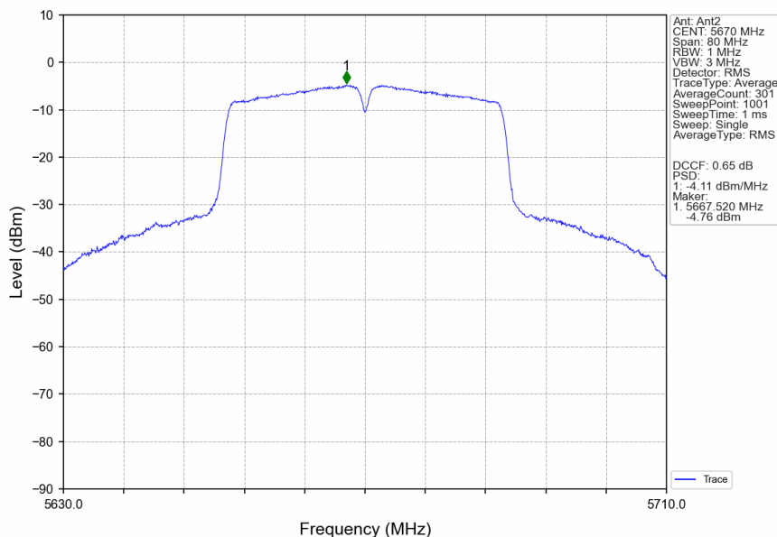
802.11ac(VHT40)_HCH_5670MHz_Ant2_NTNV
