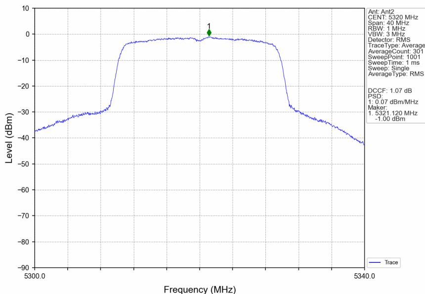
802.11ax(HEW20)_HCH_5320MHz_SU_/_Ant2_NTNV
