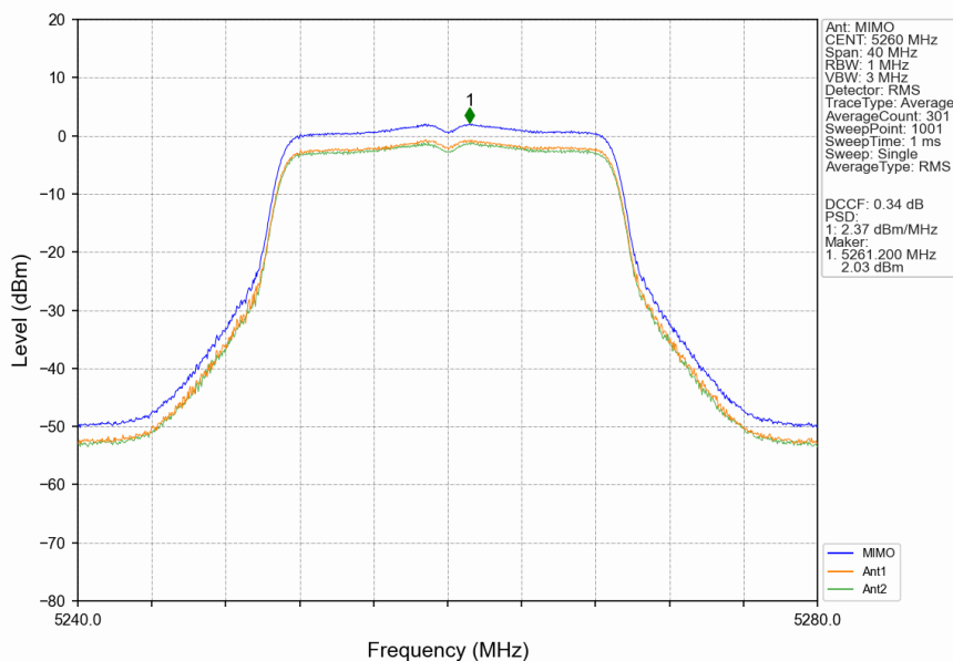
802.11ac(VHT20)_LCH_5260MHz_MIMO_NTNV
