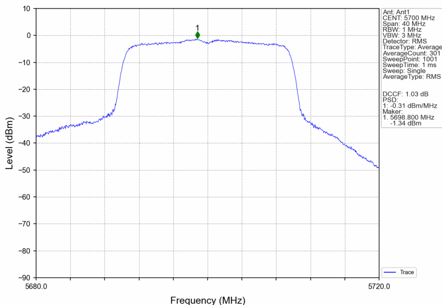
802.11ax(HEW20)_HCH_5700MHz_SU_/_Ant1_NTNV
