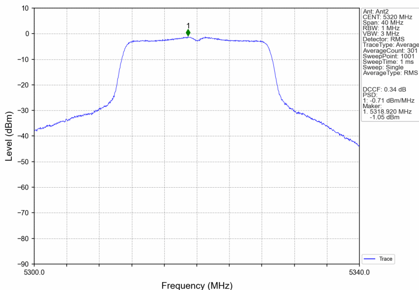
802.11ac(VHT20)_HCH_5320MHz_Ant2_NTNV
