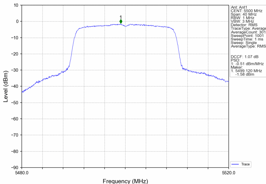
802.11ax(HEW20)_LCH_5500MHz_SU_ / _Ant1_NTNV
