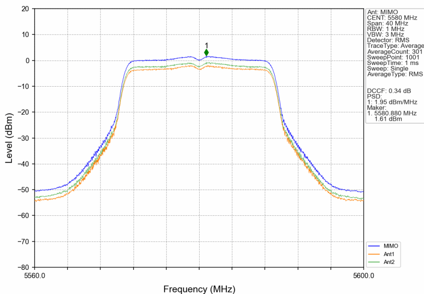
802.11ac(VHT20)_MCH_5580MHz_MIMO_NTNV
