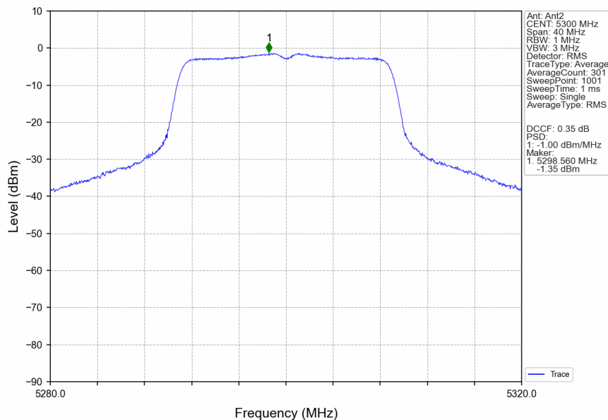
802.11ac(VHT20)_MCH_5300MHz_Ant2_NTNV
