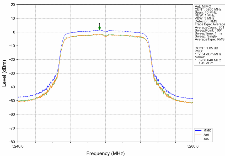
802.11ax(HEW20)_LCH_5260MHz_SU_ / _MIMO_NTNV
