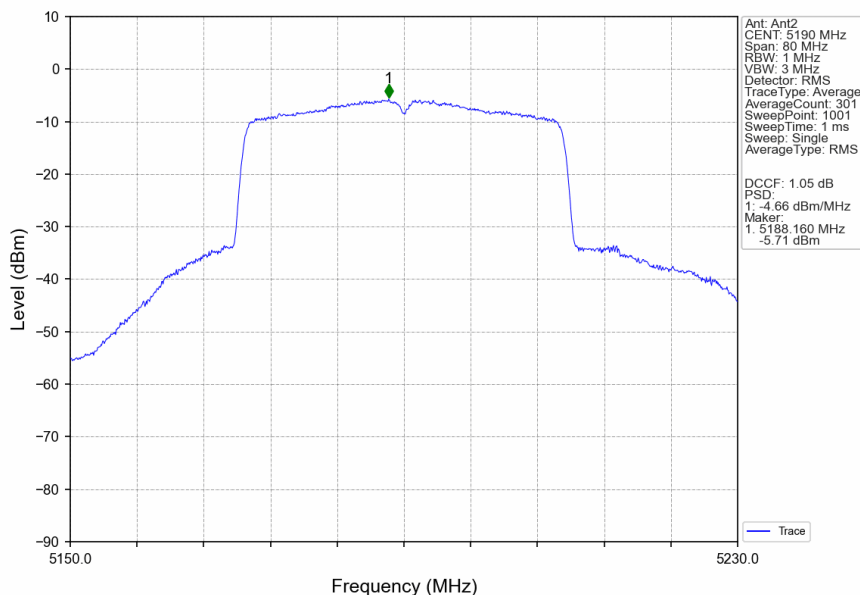
802.11ax(HEW40)_LCH_5190MHz_SU_ / _Ant2_NTNV
