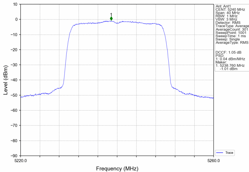
802.11ax(HEW20)_HCH_5240MHz_SU_/_Ant1_NTNV
