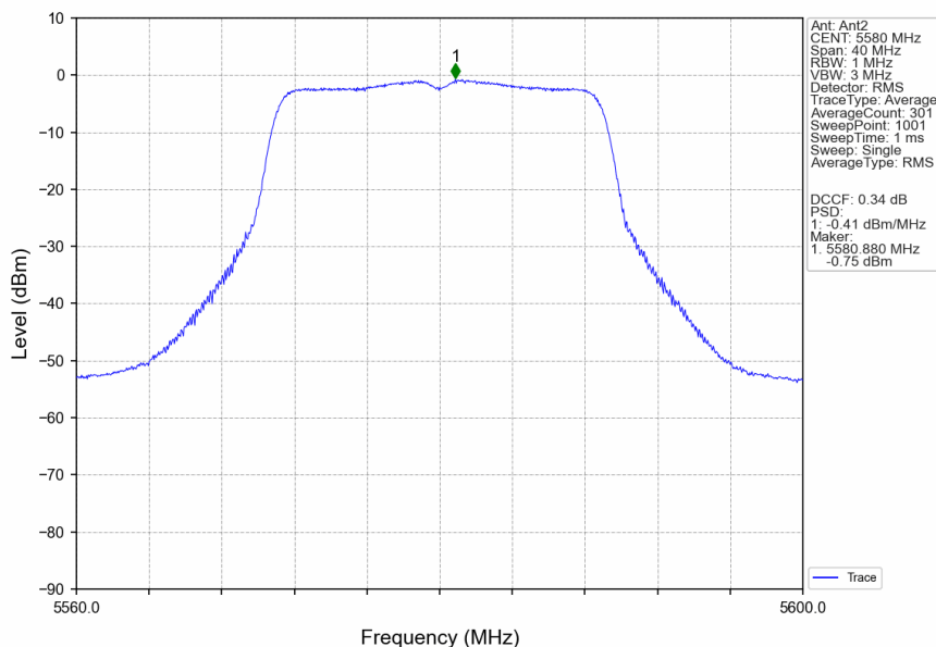
802.11ac(VHT20)_MCH_5580MHz_Ant2_NTNV
