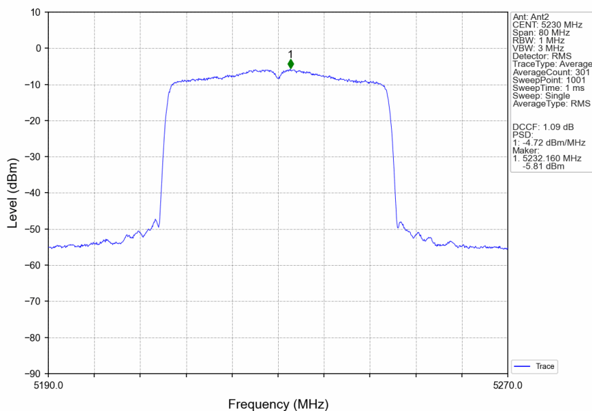
802.11ax(HEW40)_HCH_5230MHz_SU_/_Ant2_NTNV
