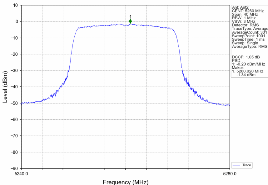
802.11ax(HEW20)_LCH_5260MHz_SU_ / _Ant2_NTNV
