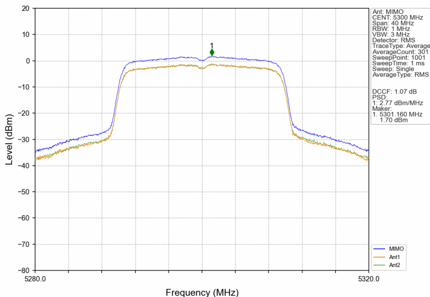
802.11ax(HEW20)_MCH_5300MHz_SU_/_MIMO_NTNV
