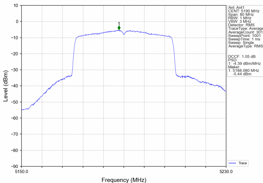
802.11ax(HEW40)_LCH_5190MHz_SU_/_Ant1_NTNV
