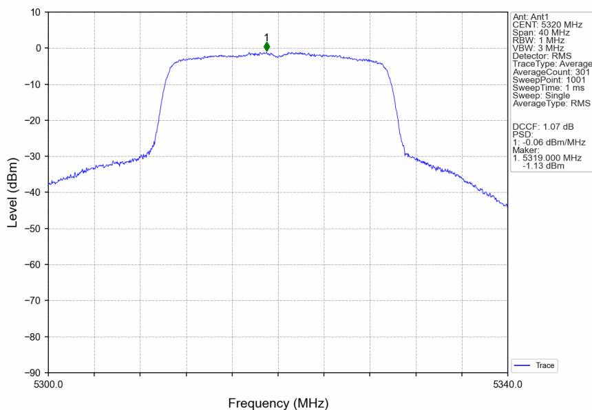
802.11ax(HEW20)_HCH_5320MHz_SU_/_Ant1_NTNV
