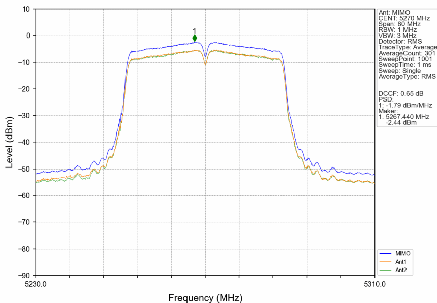
802.11ac(VHT40)_LCH_5270MHz_MIMO_NTNV
