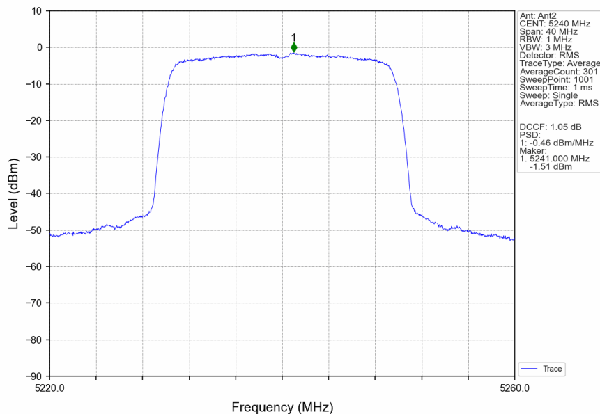
802.11ax(HEW20)_HCH_5240MHz_SU_/_Ant2_NTNV
