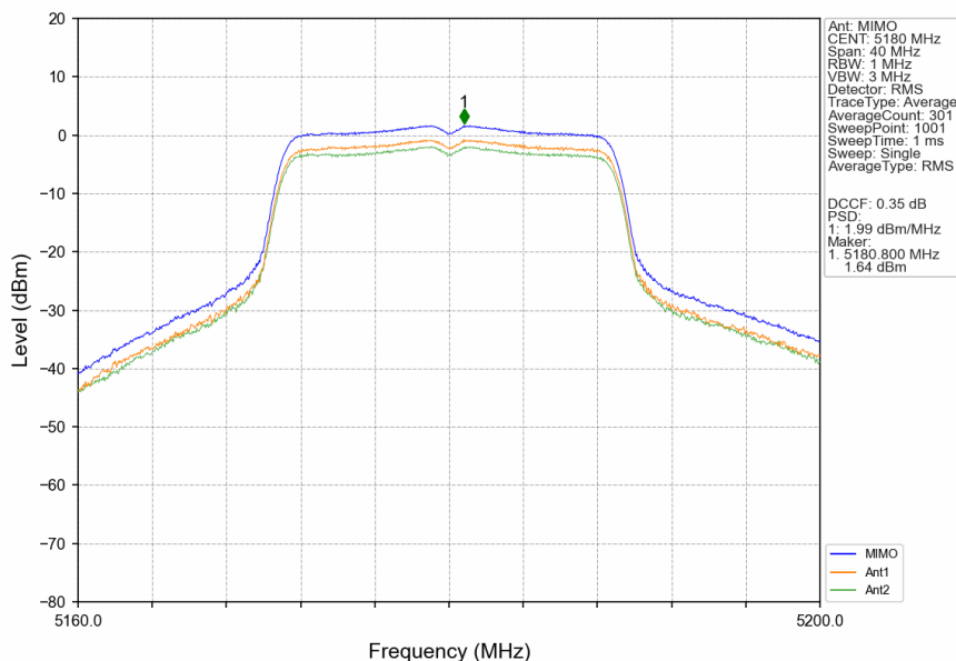
802.11ac(VHT20)_LCH_5180MHz_MIMO_NTNV
