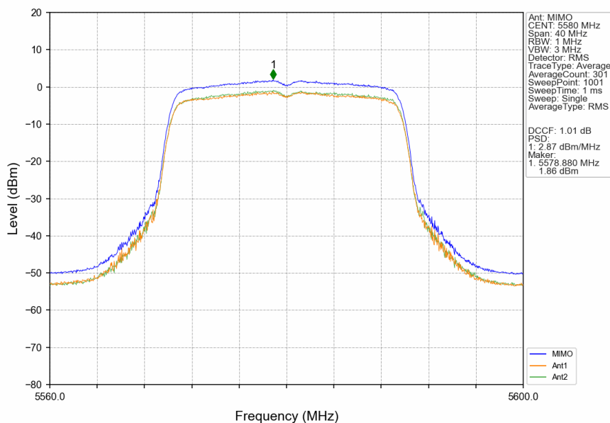
802.11ax(HEW20)_MCH_5580MHz_SU_/_MIMO_NTNV
