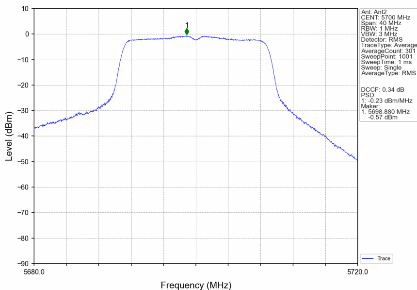
802.11ac(VHT20)_HCH_5700MHz_Ant2_NTNV
