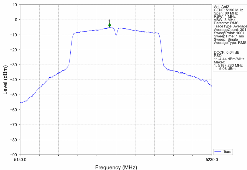
802.11ac(VHT40)_LCH_5190MHz_Ant2_NTNV
