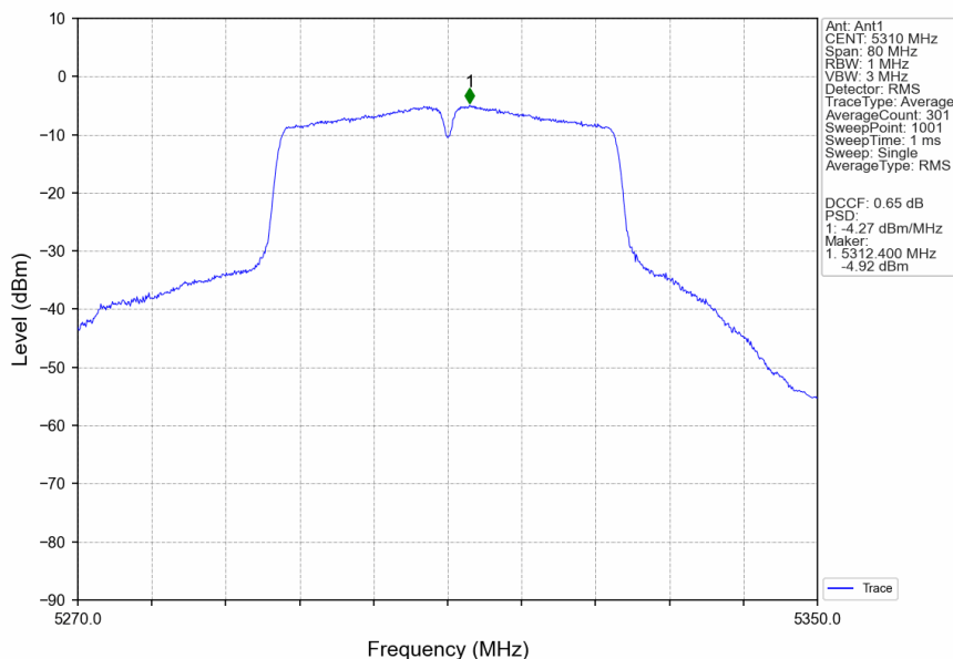
802.11ac(VHT40)_HCH_5310MHz_Ant1_NTNV
