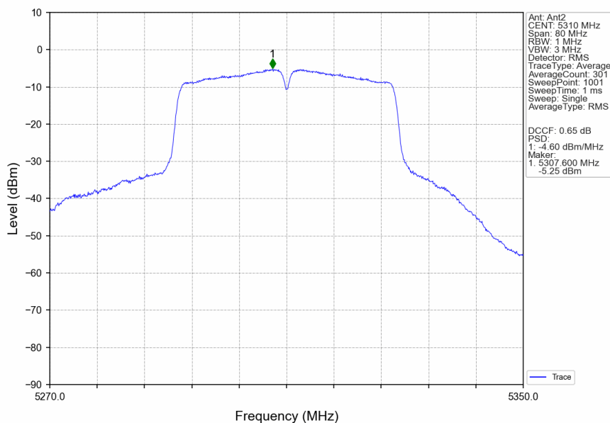
802.11ac(VHT40)_HCH_5310MHz_Ant2_NTNV
