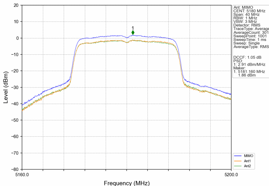
802.11ax(HEW20)_LCH_5180MHz_SU_/_MIMO_NTNV
