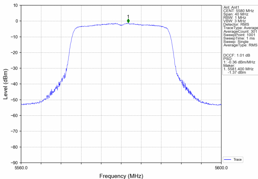
802.11ax(HEW20)_MCH_5580MHz_SU_/_Ant1_NTNV
