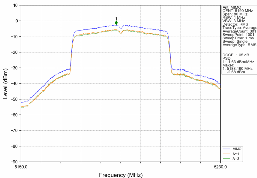
802.11ax(HEW40)_LCH_5190MHz_SU_ / _MIMO_NTNV
