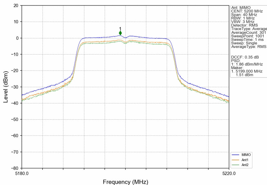
802.11ac(VHT20)_MCH_5200MHz_MIMO_NTNV
