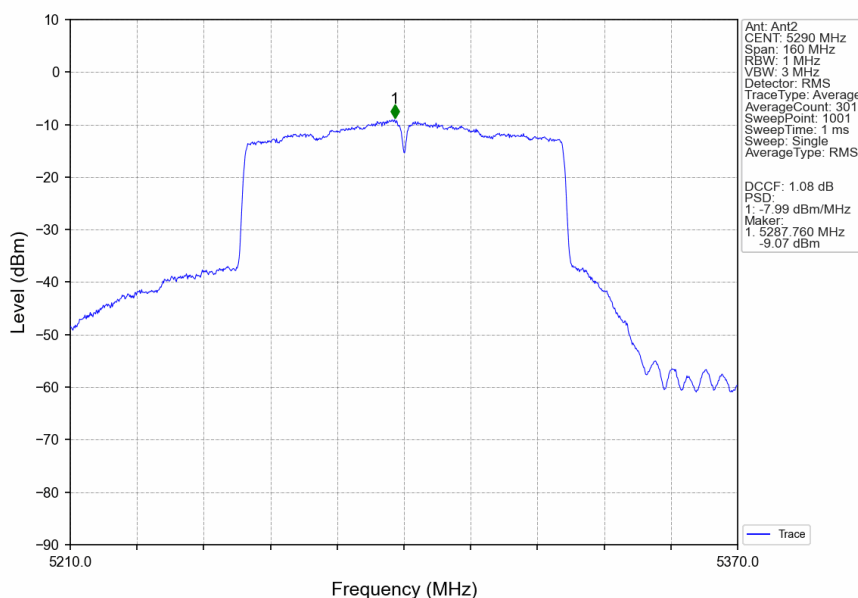
802.11ac(VHT80)_MCH_5290MHz_Ant2_NTNV
