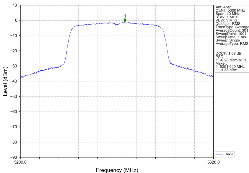
802.11ax(HEW20)_MCH_5300MHz_SU_/_Ant2_NTNV
