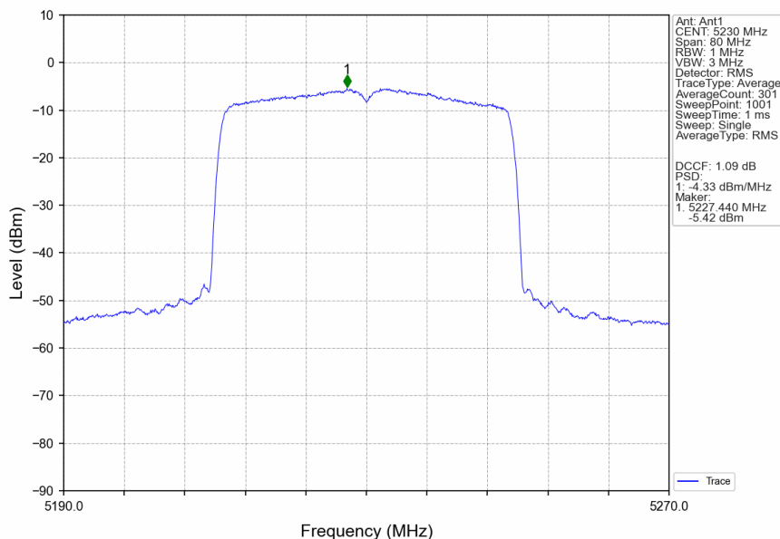
802.11ax(HEW40)_HCH_5230MHz_SU_/_Ant1_NTNV
