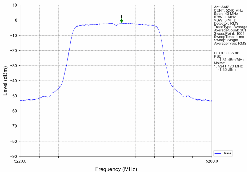
802.11ac(VHT20)_HCH_5240MHz_Ant2_NTNV
