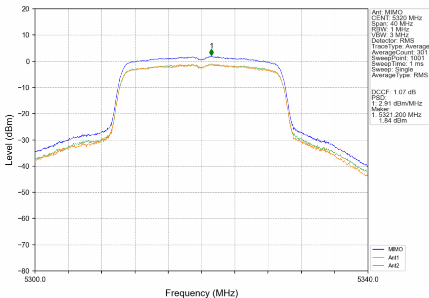
802.11ax(HEW20)_HCH_5320MHz_SU_/_MIMO_NTNV
