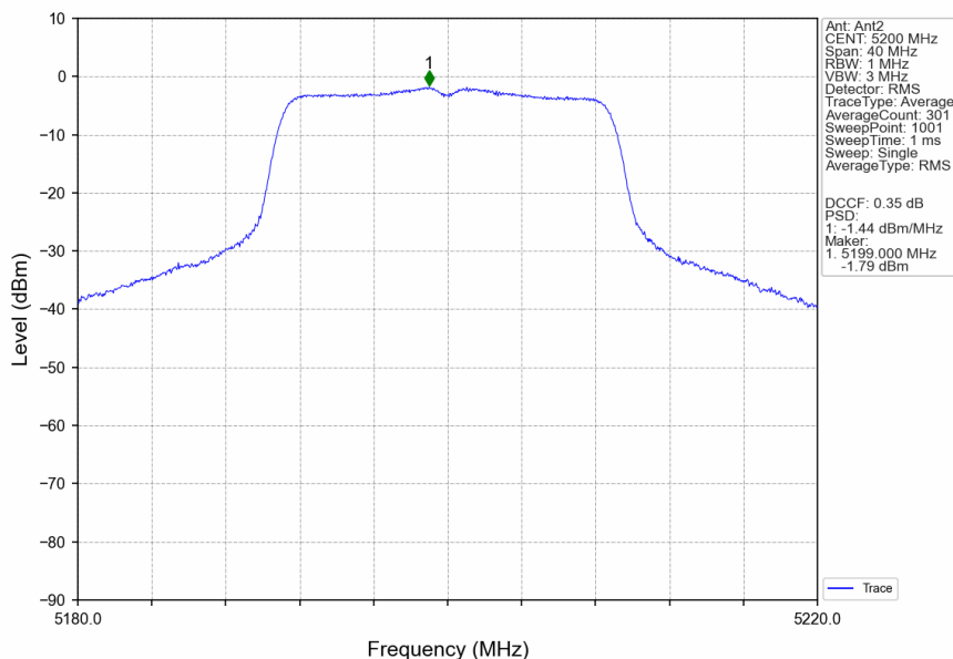
802.11ac(VHT20)_MCH_5200MHz_Ant2_NTNV
