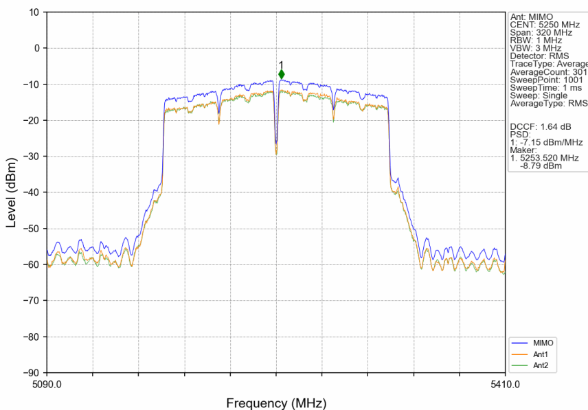
802.11ac(VHT160)_MCH_5250MHz_MIMO_NTNV
