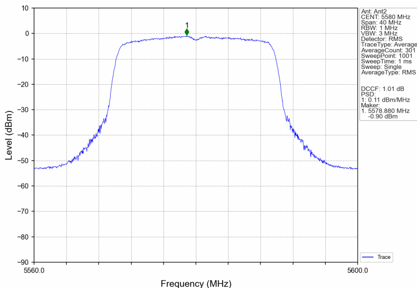
802.11ax(HEW20)_MCH_5580MHz_SU_/_Ant2_NTNV
