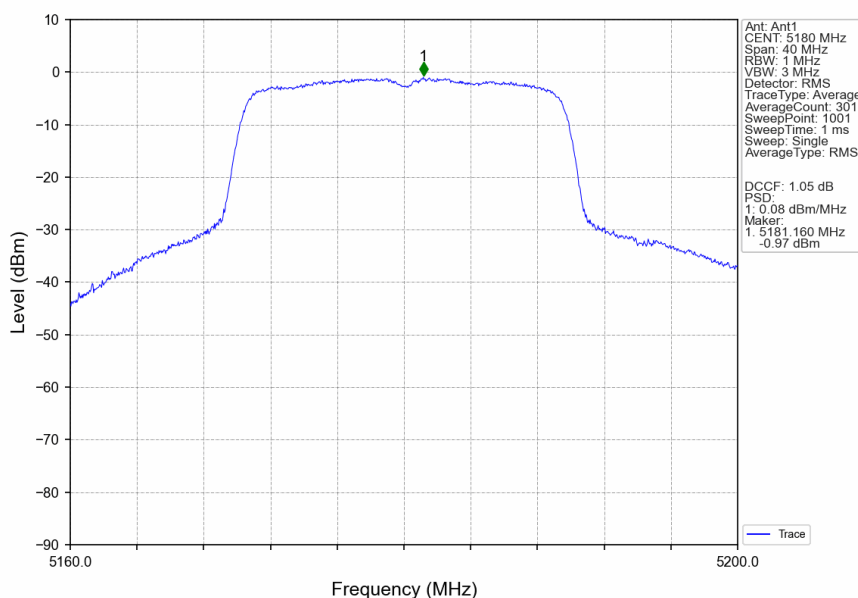
802.11ax(HEW20)_LCH_5180MHz_SU_ / _Ant1_NTNV
