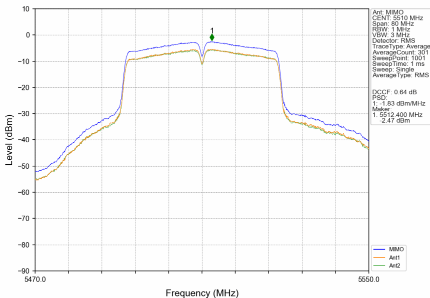
802.11ac(VHT40)_LCH_5510MHz_MIMO_NTNV
