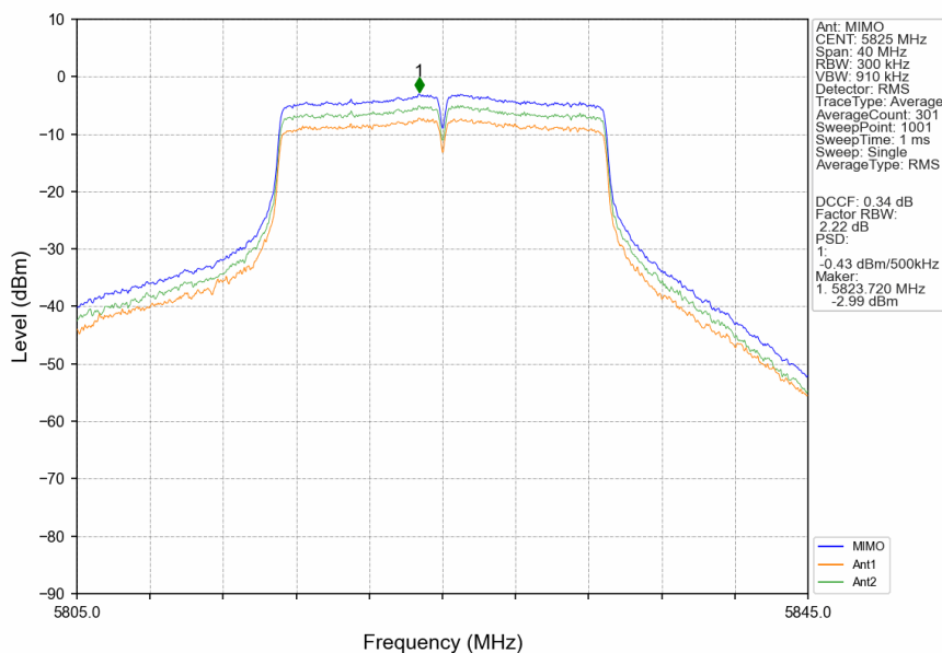
802.11ac(VHT20)_HCH_5825MHz_MIMO_NTNV
