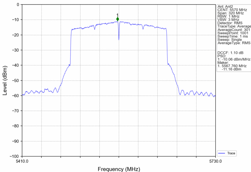
802.11ax(HEW160)_MCH_5570MHz_SU_/_Ant2_NTNV
