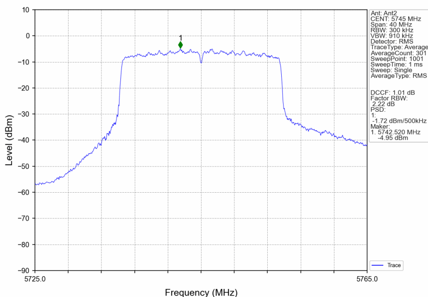
802.11ax(HEW20)_LCH_5745MHz_SU_ / _Ant2_NTNV
