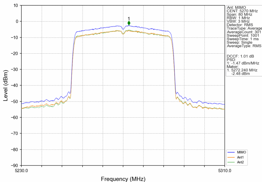
802.11ax(HEW40)_LCH_5270MHz_SU_ / _MIMO_NTNV
