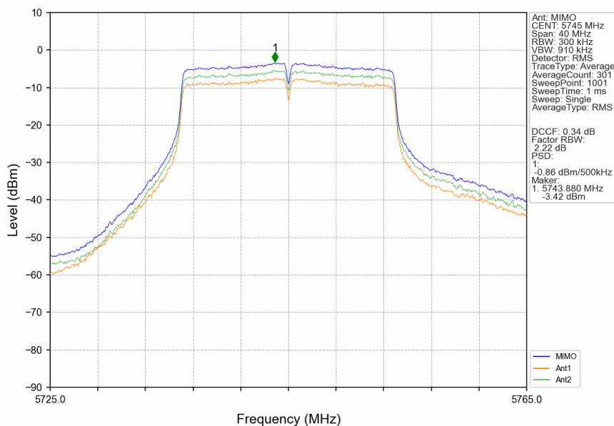
802.11ac(VHT20)_LCH_5745MHz_MIMO_NTNV
