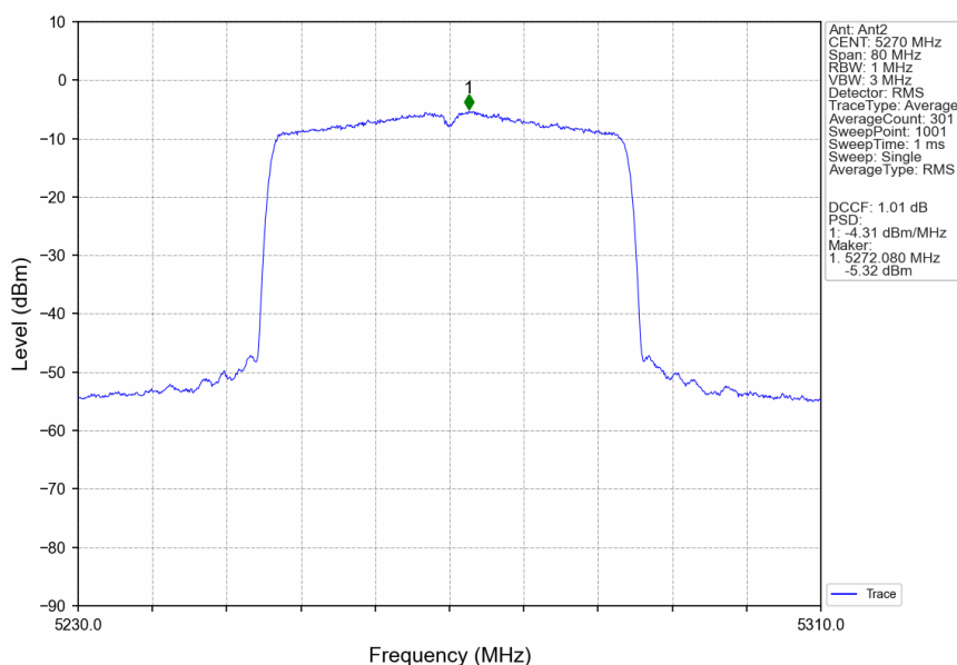
802.11ax(HEW40)_LCH_5270MHz_SU_ / _Ant2_NTNV
