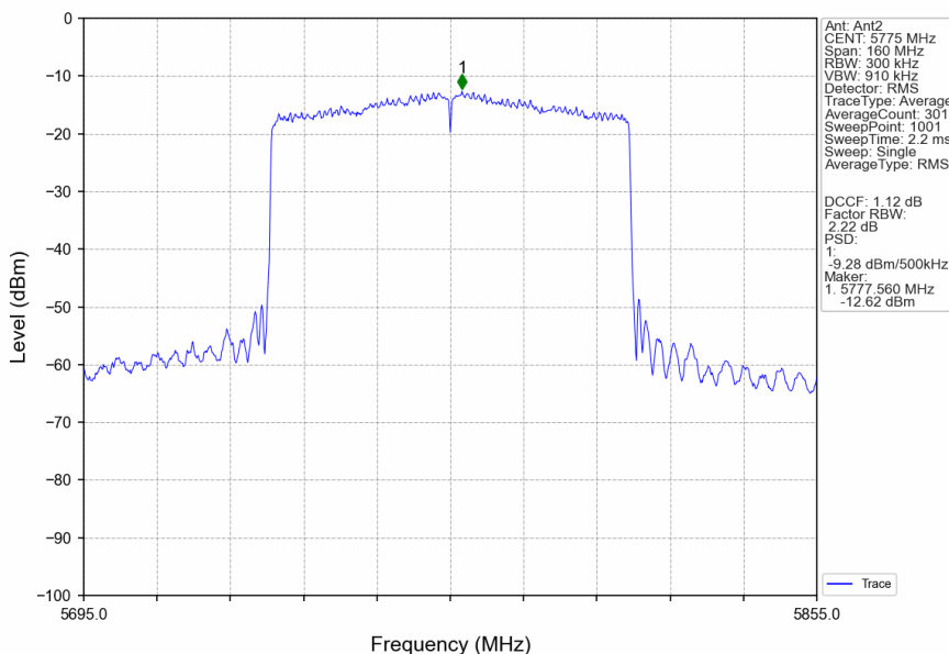
802.11ax(HEW80)_MCH_5775MHz_SU_/_Ant2_NTNV
