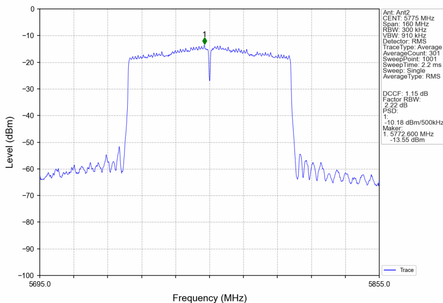
802.11ac(VHT80)_MCH_5775MHz_Ant2_NTNV
