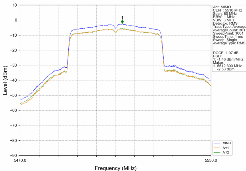
802.11ax(HEW40)_LCH_5510MHz_SU_/_MIMO_NTNV
