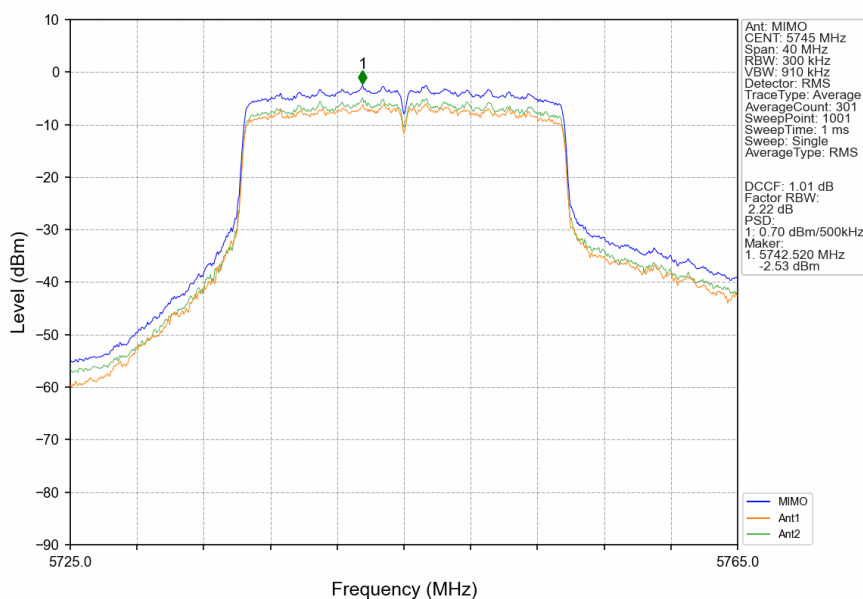
802.11ax(HEW20)_LCH_5745MHz_SU_ / _MIMO_NTNV
