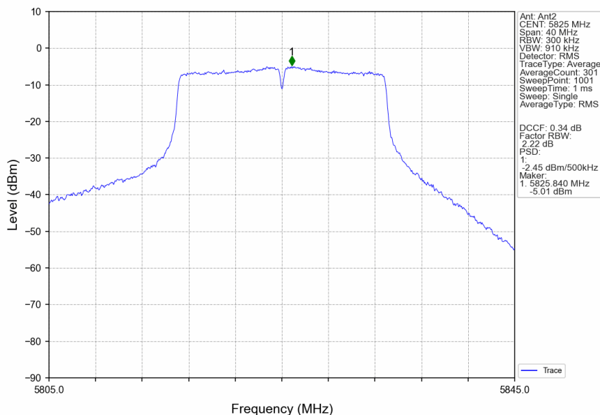
802.11ac(VHT20)_HCH_5825MHz_Ant2_NTNV
