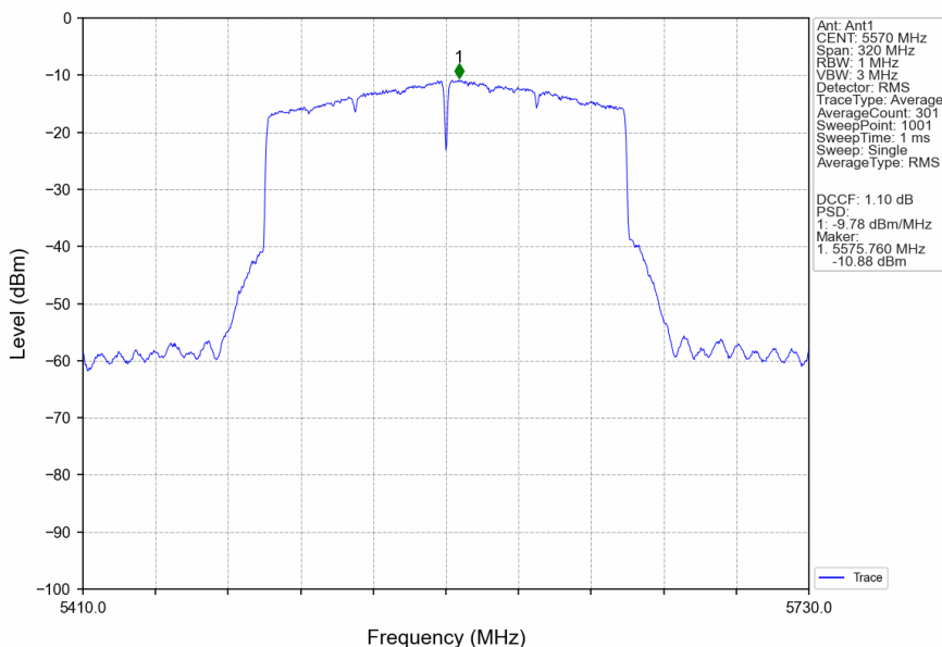
802.11ax(HEW160)_MCH_5570MHz_SU_/_Ant1_NTNV
