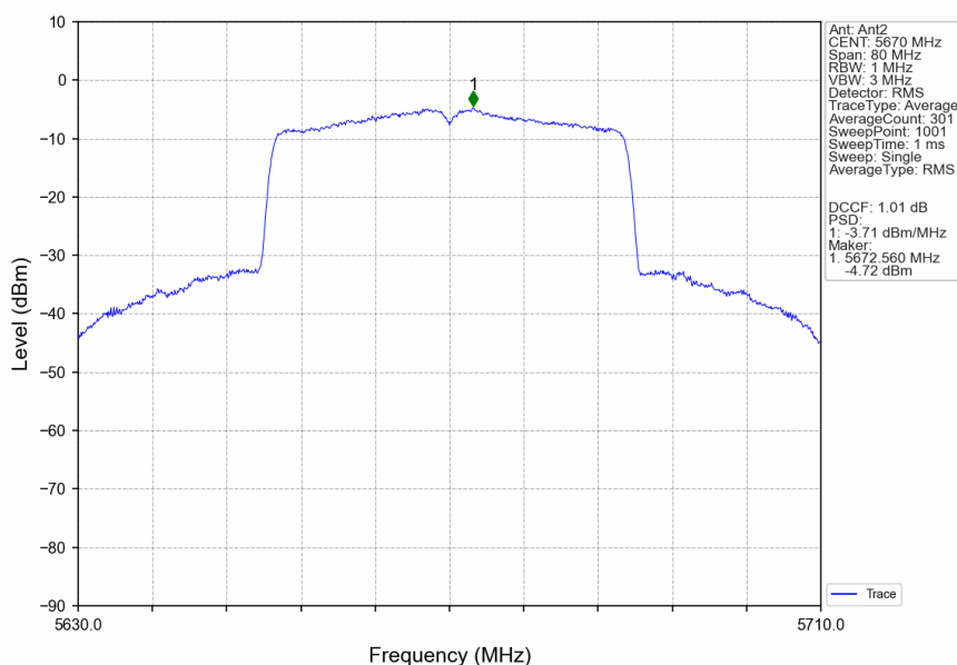
802.11ax(HEW40)_HCH_5670MHz_SU_/_Ant2_NTNV
