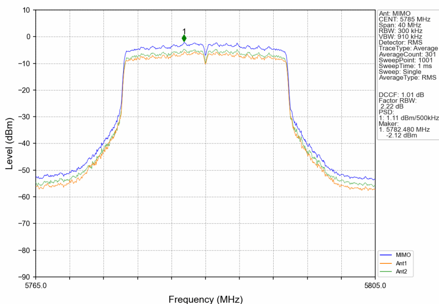
802.11ax(HEW20)_MCH_5785MHz_SU_/_MIMO_NTNV
