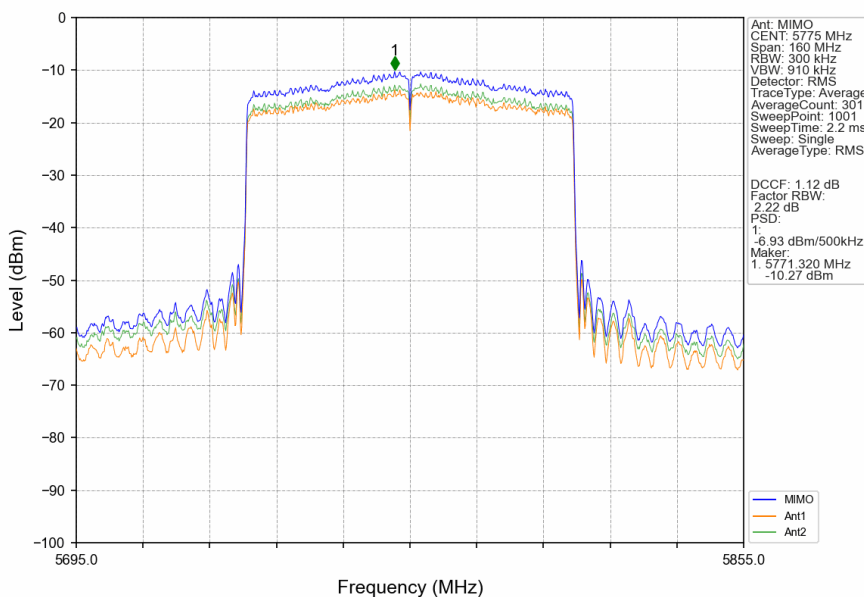
802.11ax(HEW80)_MCH_5775MHz_SU_/_MIMO_NTNV
