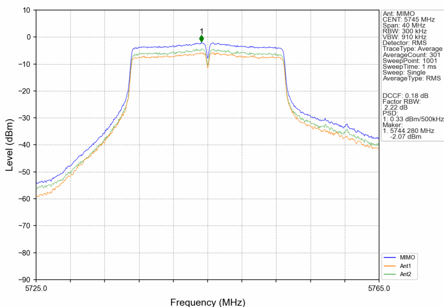
802.11n(HT20)_LCH_5745MHz_MIMO_NTNV
