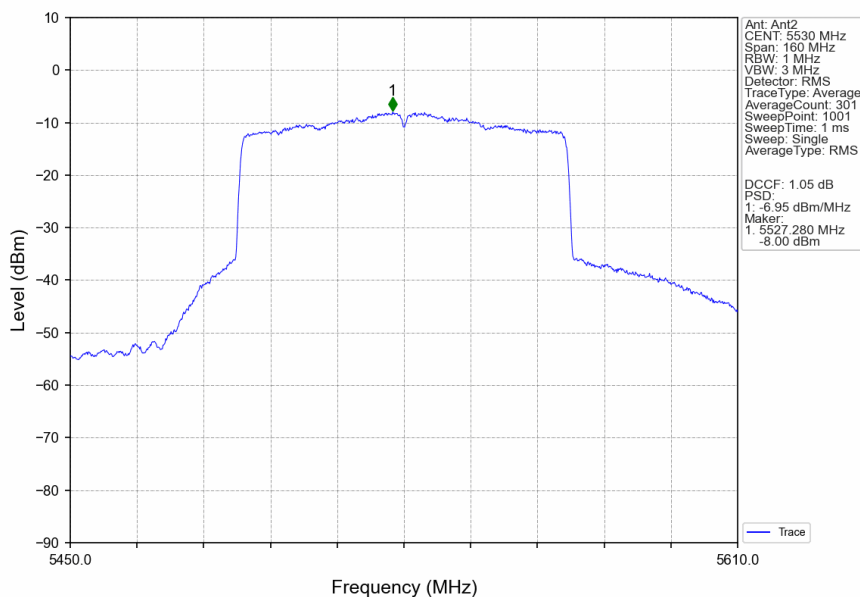
802.11ax(HEW80)_LCH_5530MHz_SU_ / _Ant2_NTNV
