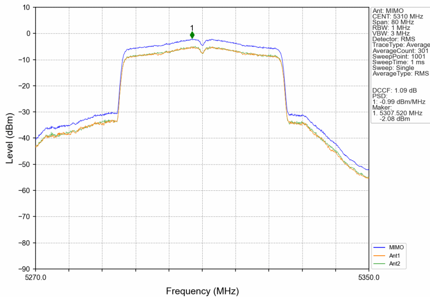
802.11ax(HEW40)_HCH_5310MHz_SU_/_MIMO_NTNV
