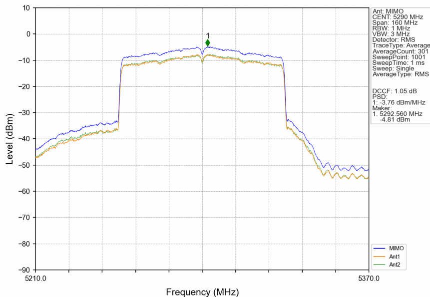
802.11ax(HEW80)_MCH_5290MHz_SU_/_MIMO_NTNV
