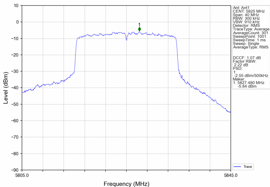
802.11ax(HEW20)_HCH_5825MHz_SU_/_Ant1_NTNV
