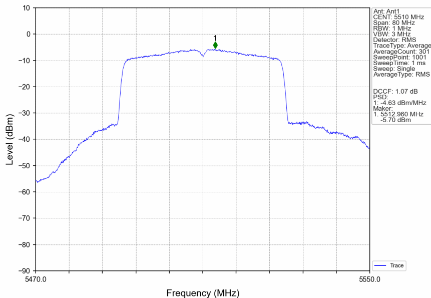
802.11ax(HEW40)_LCH_5510MHz_SU_/_Ant1_NTNV
