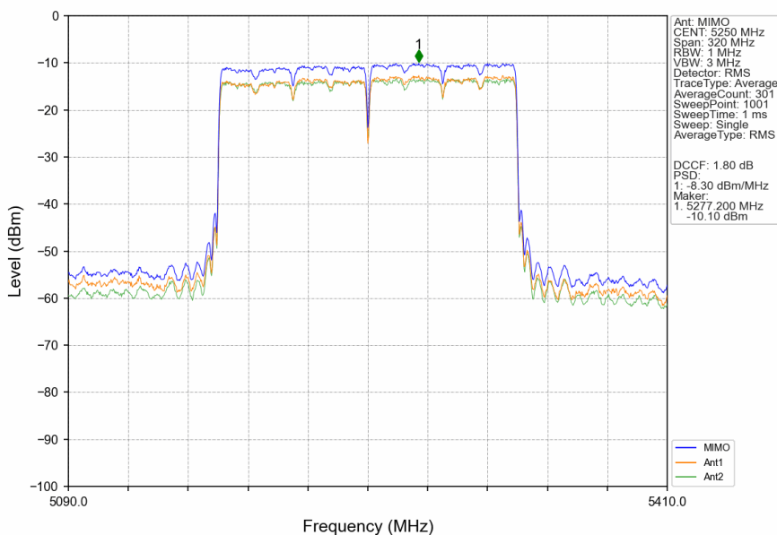
802.11ax(HEW160)_MCH_5250MHz_SU_/_MIMO_NTNV
