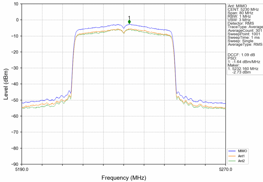
802.11ax(HEW40)_HCH_5230MHz_SU_/_MIMO_NTNV
