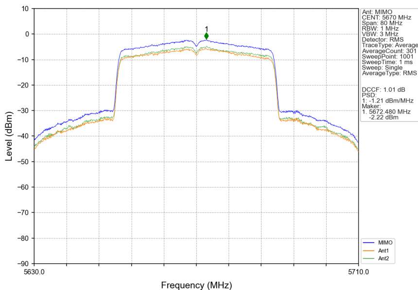
802.11ax(HEW40)_HCH_5670MHz_SU_/_MIMO_NTNV
