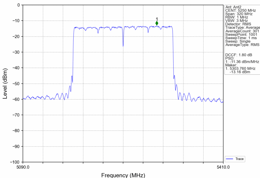
802.11ax(HEW160)_MCH_5250MHz_SU_/_Ant2_NTNV
