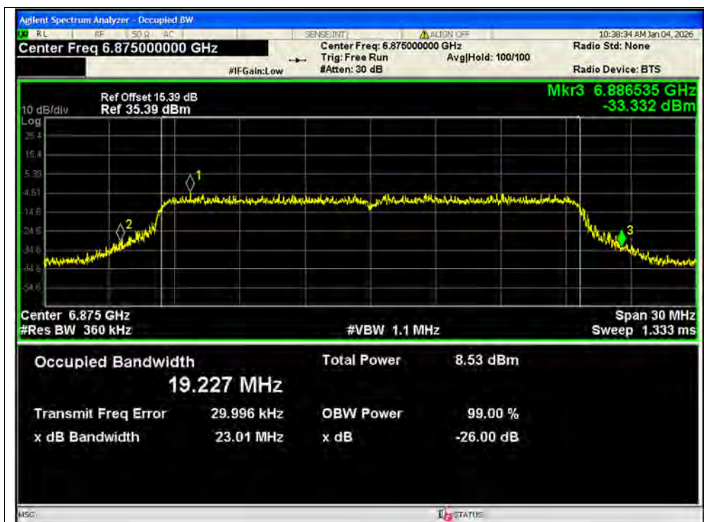
-26dB Bandwidth NVNT ax20 6875MHz Ant1 MIMO
