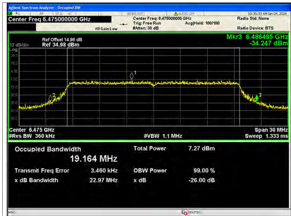
-26dB Bandwidth NVNT ax20 6475MHz Ant1 MIMO
