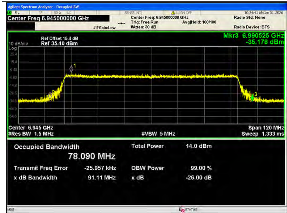
-26dB Bandwidth NVNT ax80 6945MHz Ant2 MIMO
