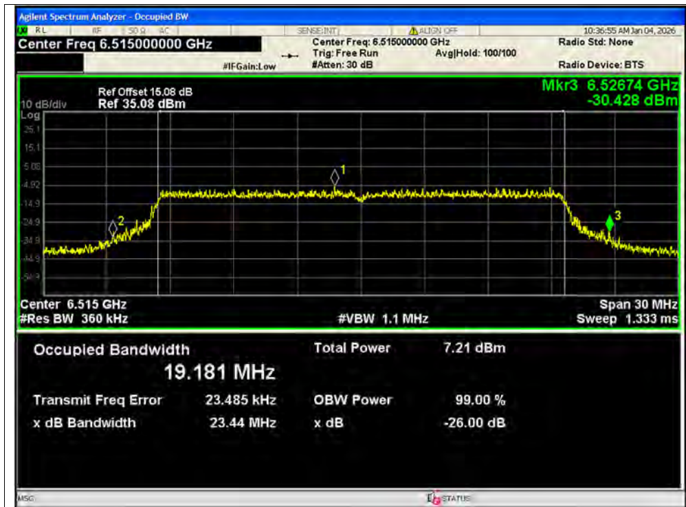
-26dB Bandwidth NVNT ax20 6515MHz Ant1 MIMO
