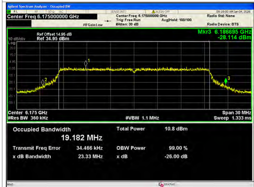
-26dB Bandwidth NVNT ax20 6175MHz Ant1 SISO
