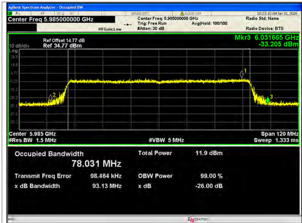
-26dB Bandwidth NVNT ax80 5985MHz Ant1 MIMO
