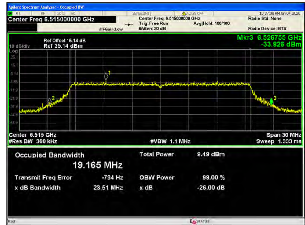
-26dB Bandwidth NVNT ax20 6515MHz Ant2 MIMO
