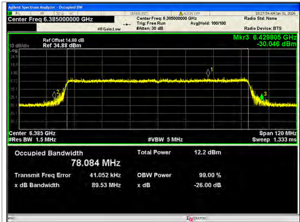
-26dB Bandwidth NVNT ax80 6385MHz Ant1 MIMO
