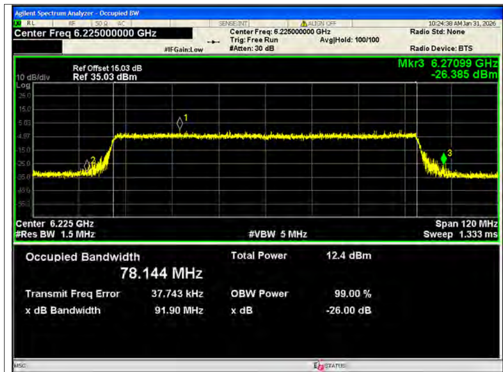
-26dB Bandwidth NVNT ax80 6225MHz Ant1 MIMO
