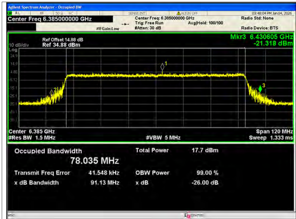
-26dB Bandwidth NVNT ax80 6385MHz Ant1 SISO
