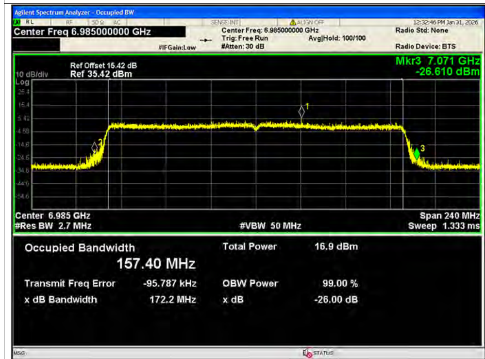
-26dB Bandwidth NVNT ax160 6985MHz Ant2 MIMO
