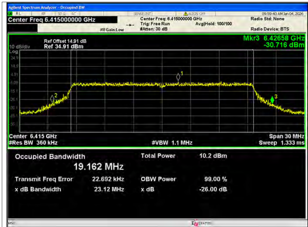
-26dB Bandwidth NVNT ax20 6415MHz Ant2 SISO
