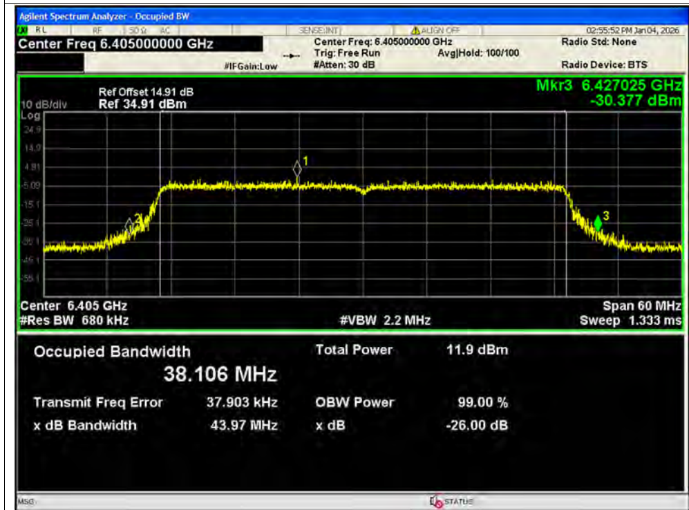
-26dB Bandwidth NVNT ax40 6405MHz Ant2 MIMO
