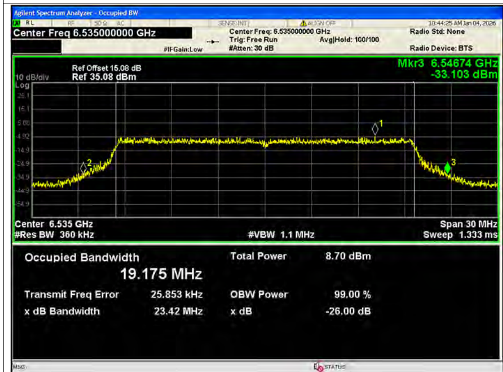
-26dB Bandwidth NVNT ax20 6535MHz Ant2 MIMO
