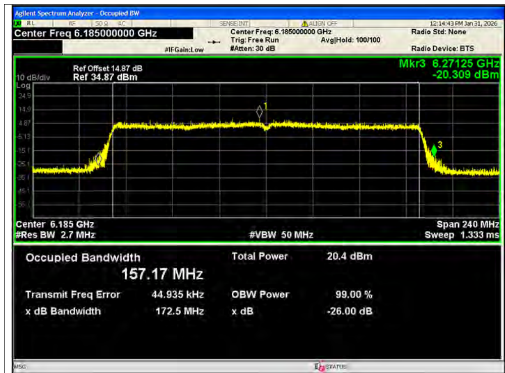
-26dB Bandwidth NVNT ax160 6185MHz Ant2 SISO
