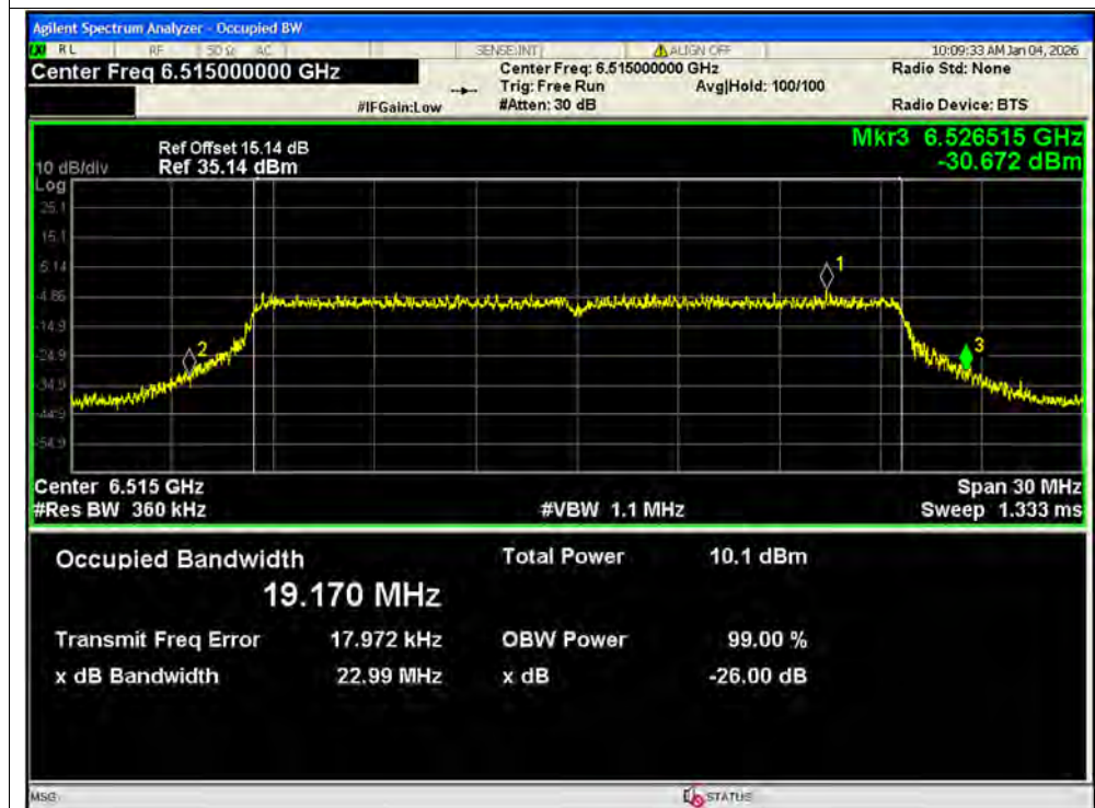
-26dB Bandwidth NVNT ax20 6515MHz Ant2 SISO
