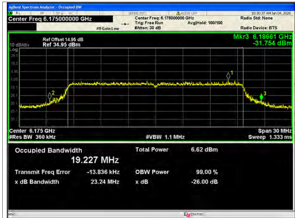
-26dB Bandwidth NVNT ax20 6175MHz Ant1 MIMO
