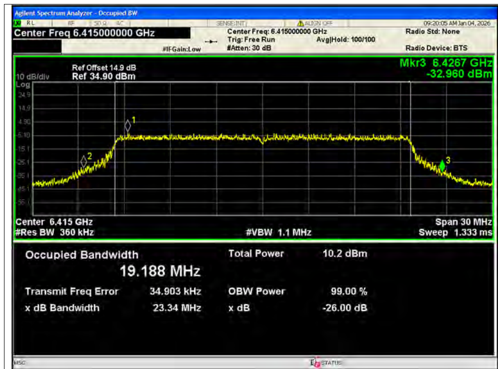
-26dB Bandwidth NVNT ax20 6415MHz Ant1 SISO
