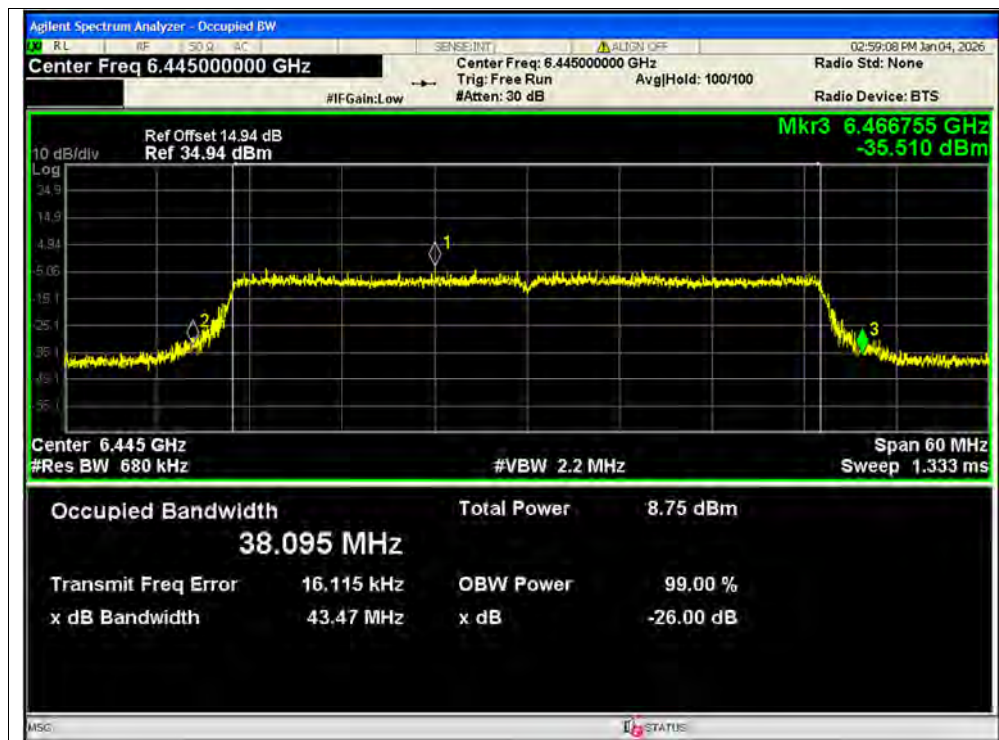
-26dB Bandwidth NVNT ax40 6445MHz Ant1 MIMO
