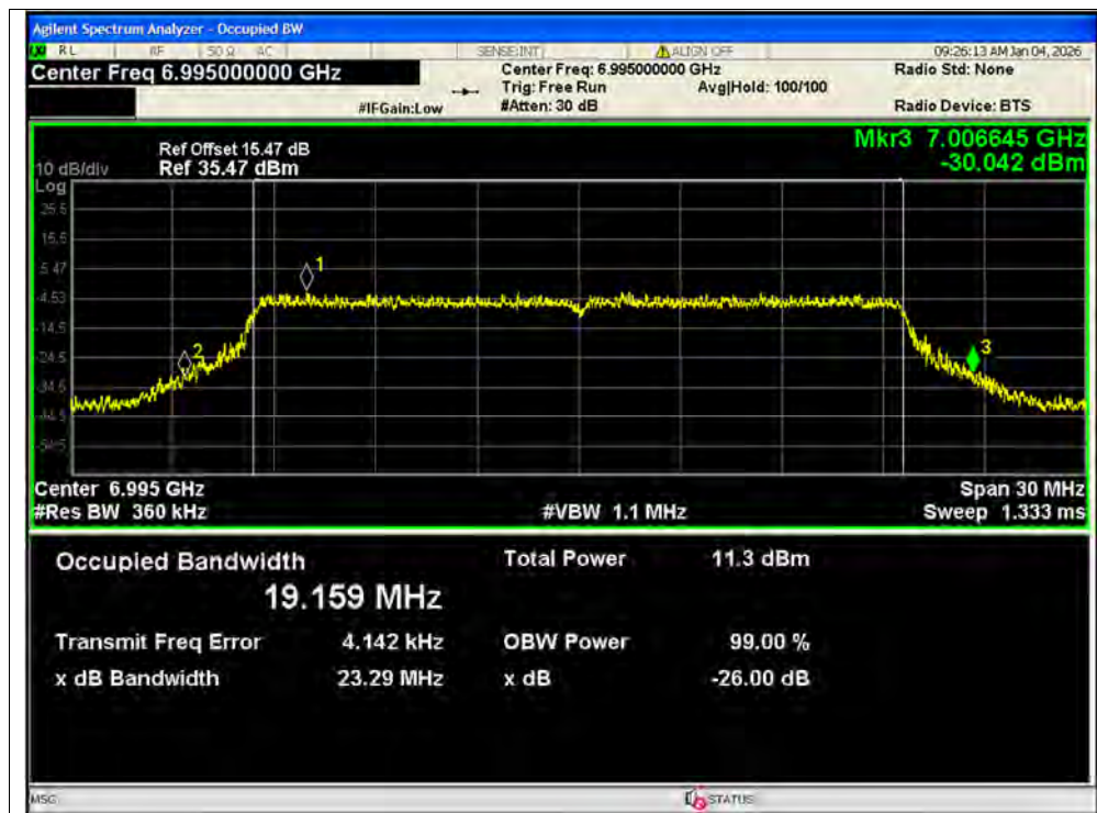
-26dB Bandwidth NVNT ax20 6995MHz Ant1 SISO
