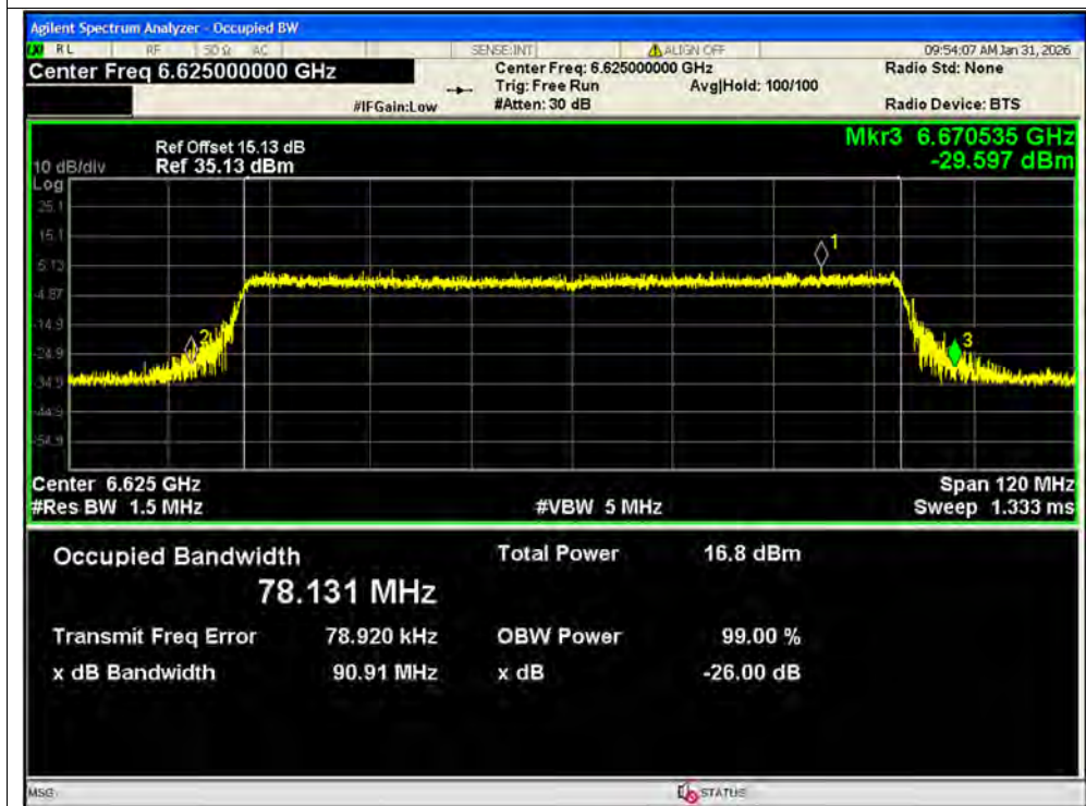
-26dB Bandwidth NVNT ax80 6625MHz Ant2 SISO
