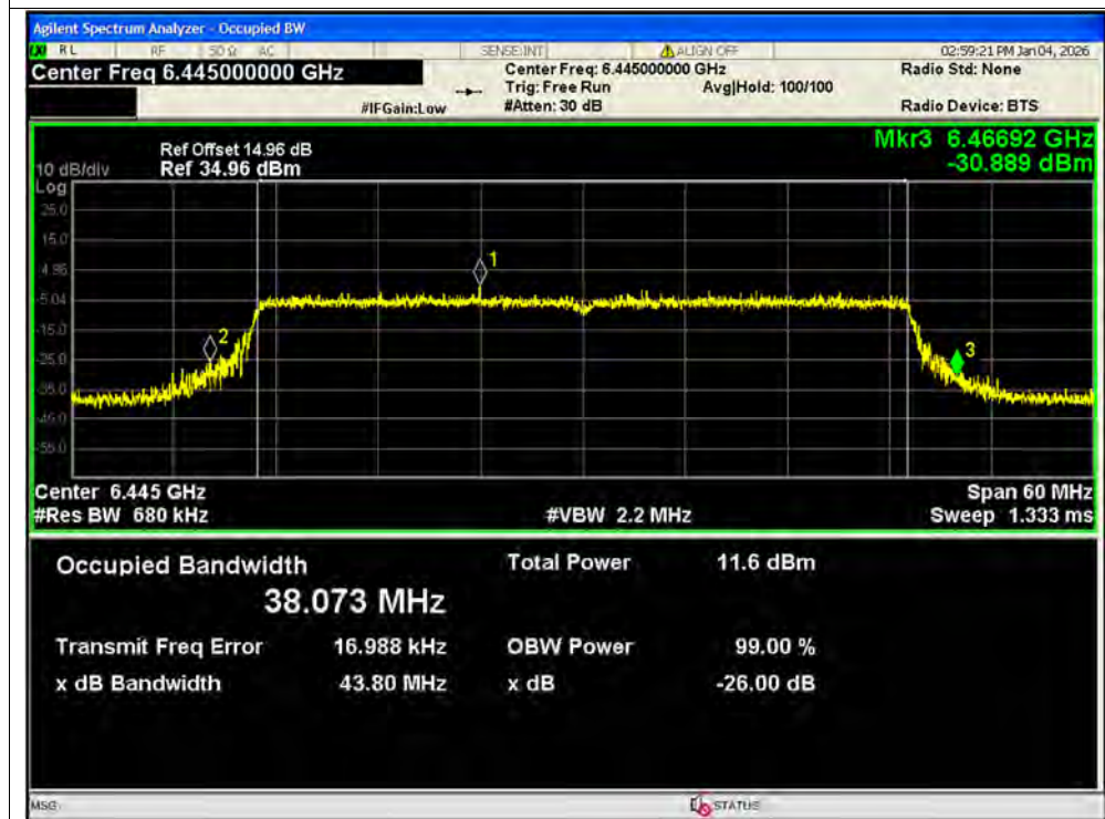
-26dB Bandwidth NVNT ax40 6445MHz Ant2 MIMO
