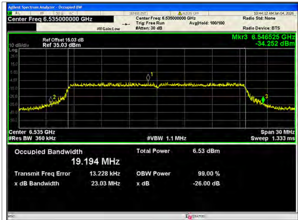
-26dB Bandwidth NVNT ax20 6535MHz Ant1 MIMO
