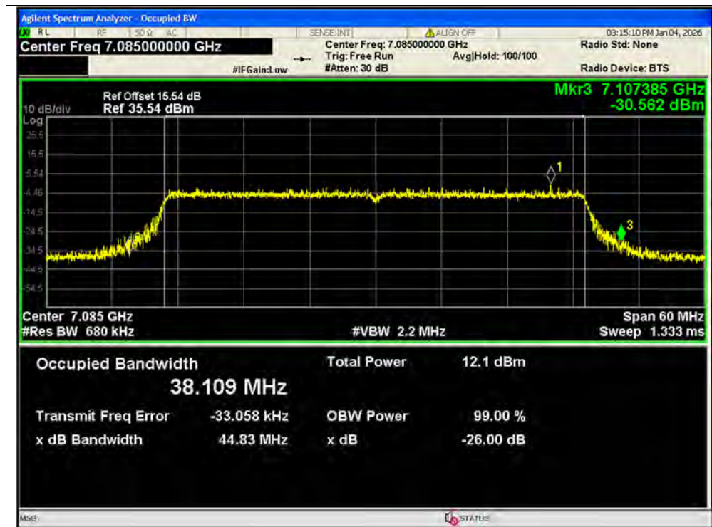
-26dB Bandwidth NVNT ax40 7085MHz Ant2 MIMO
