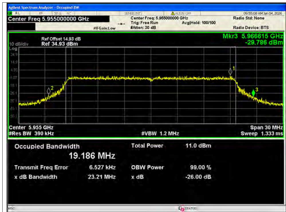
-26dB Bandwidth NVNT ax20 5955MHz Ant2 SISO
