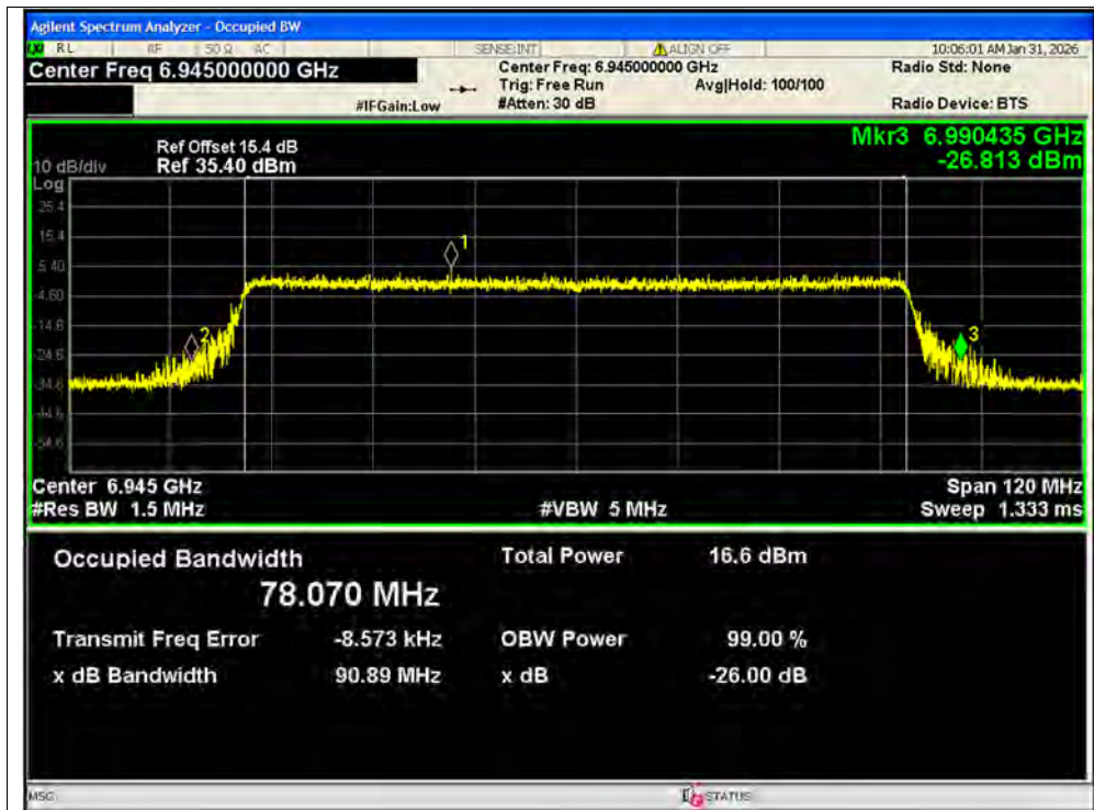
-26dB Bandwidth NVNT ax80 6945MHz Ant2 SISO
