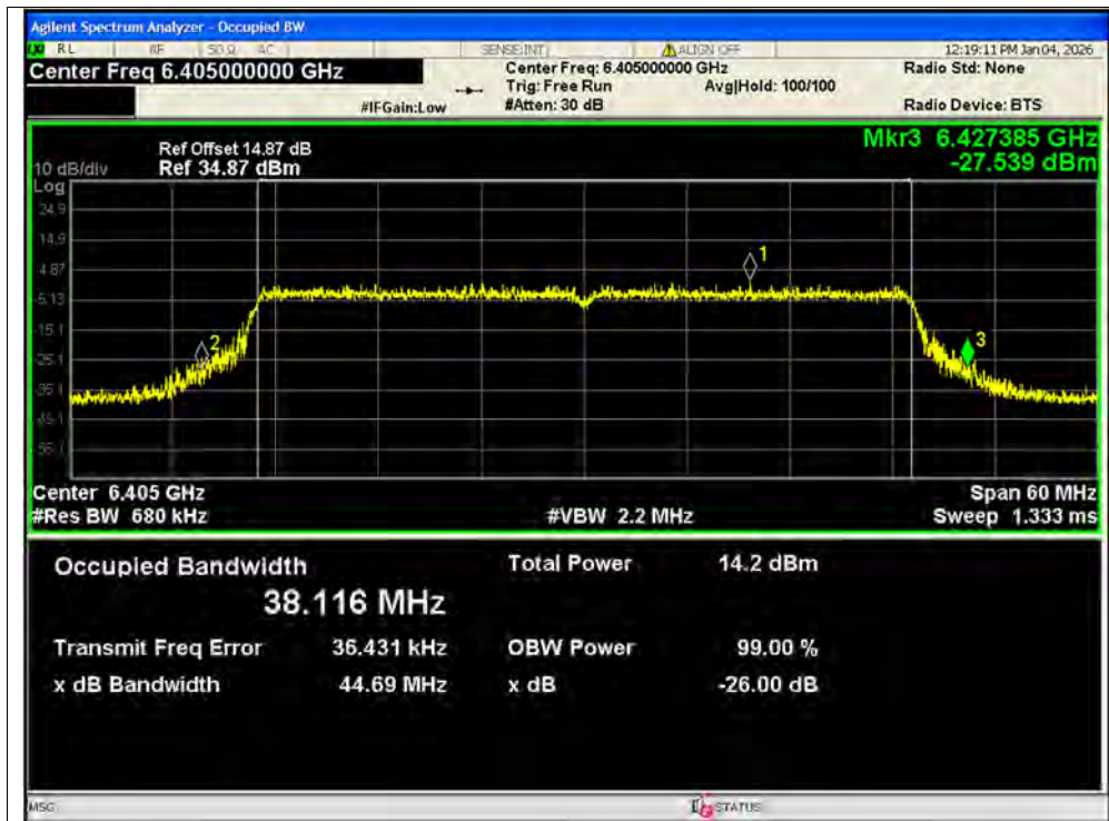
-26dB Bandwidth NVNT ax40 6405MHz Ant1 SISO
