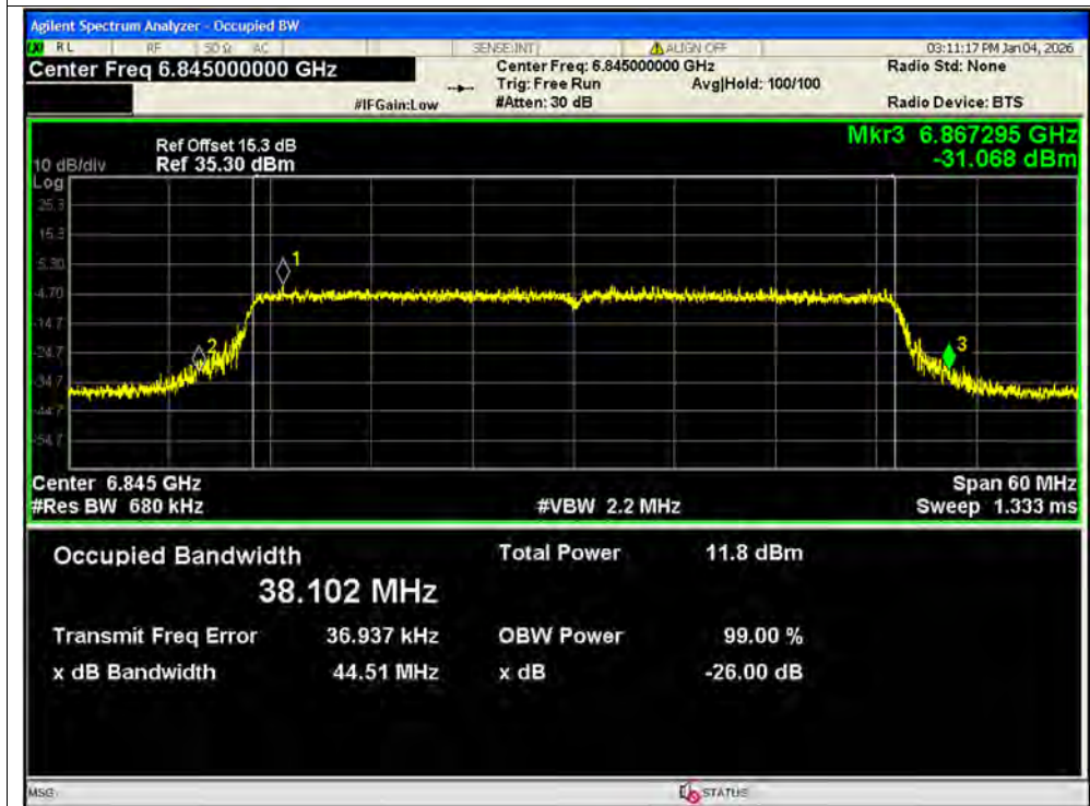
-26dB Bandwidth NVNT ax40 6845MHz Ant2 MIMO
