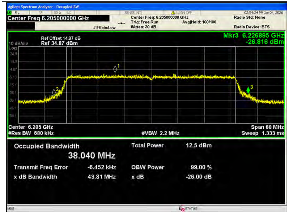
-26dB Bandwidth NVNT ax40 6205MHz Ant2 MIMO
