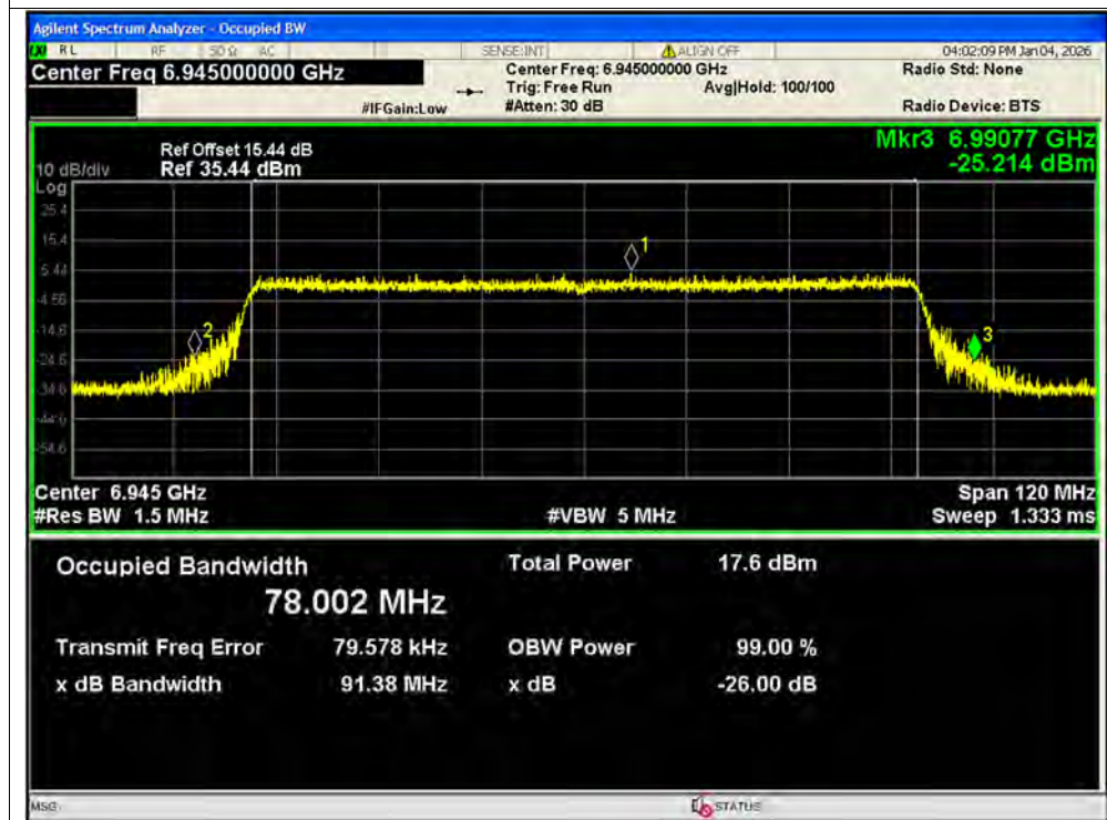
-26dB Bandwidth NVNT ax80 6945MHz Ant1 SISO
