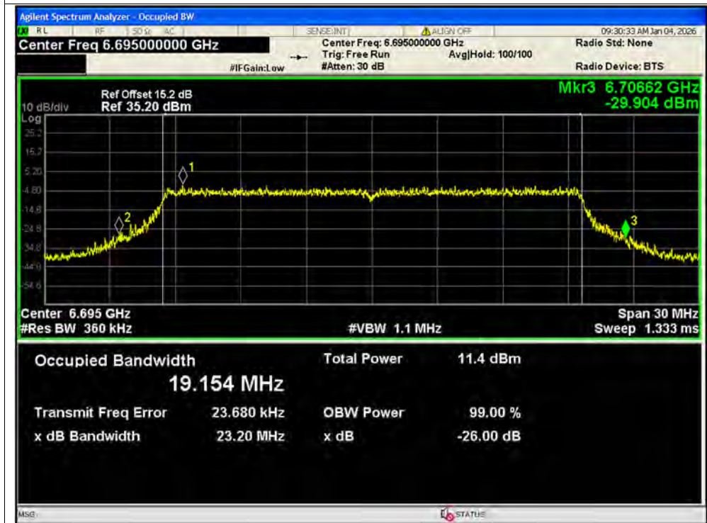
-26dB Bandwidth NVNT ax20 6695MHz Ant1 SISO
