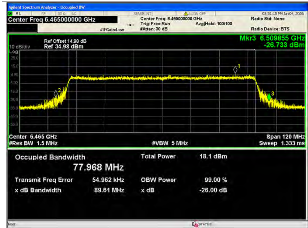
-26dB Bandwidth NVNT ax80 6465MHz Ant1 SISO
