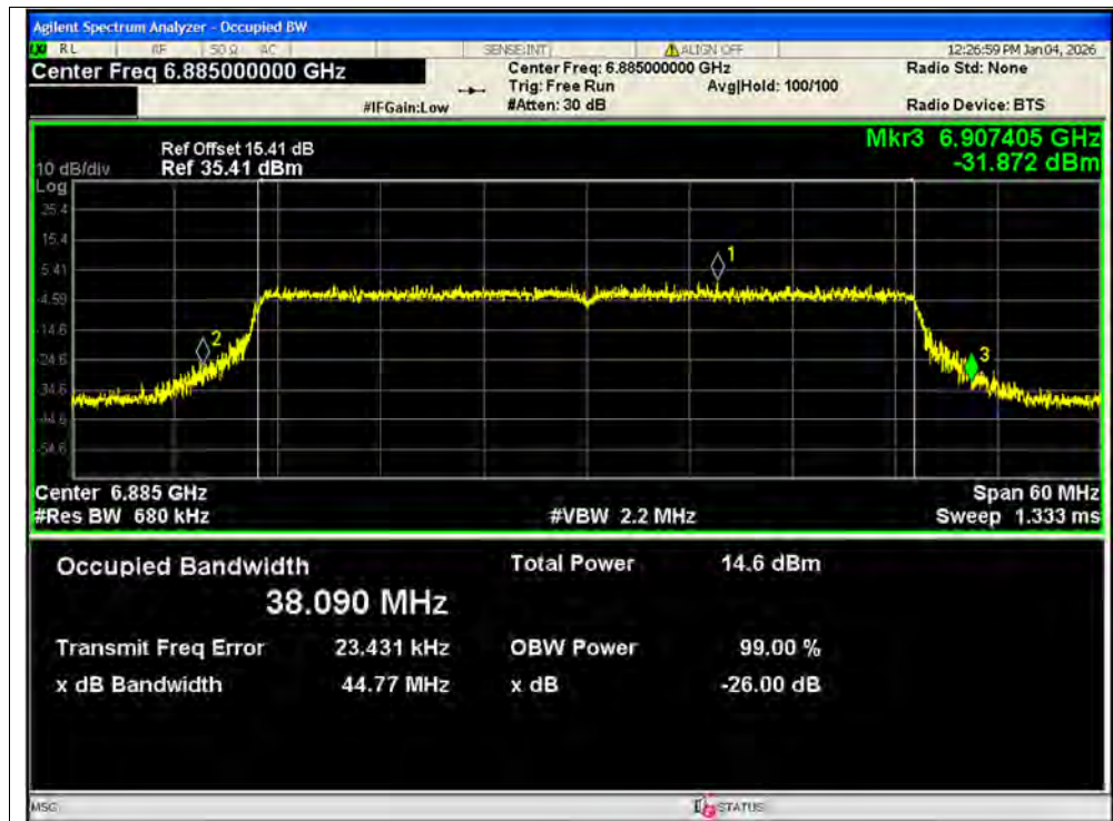
-26dB Bandwidth NVNT ax40 6885MHz Ant1 SISO
