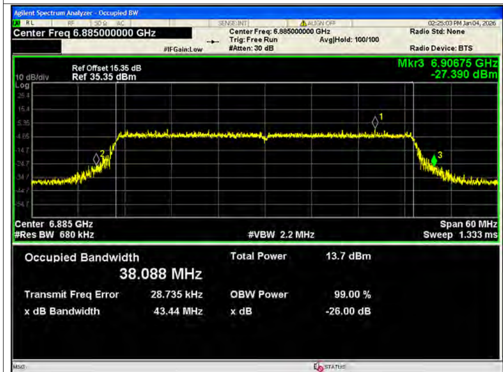
-26dB Bandwidth NVNT ax40 6885MHz Ant2 SISO
