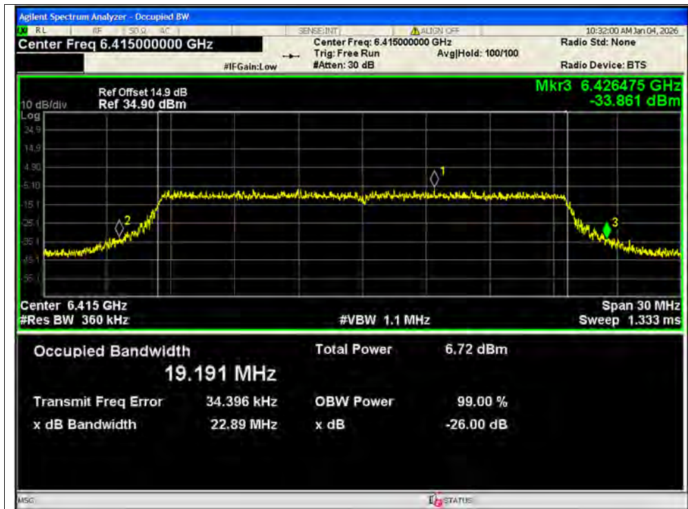
-26dB Bandwidth NVNT ax20 6415MHz Ant1 MIMO
