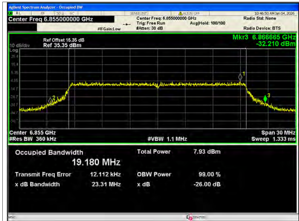
-26dB Bandwidth NVNT ax20 6855MHz Ant1 MIMO
