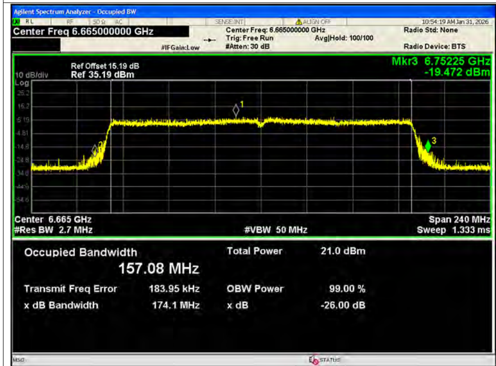
-26dB Bandwidth NVNT ax160 6665MHz Ant1 SISO
