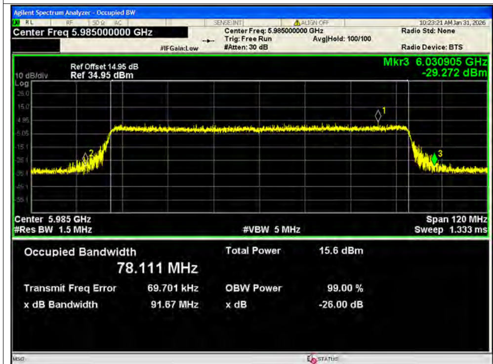
-26dB Bandwidth NVNT ax80 5985MHz Ant2 MIMO
