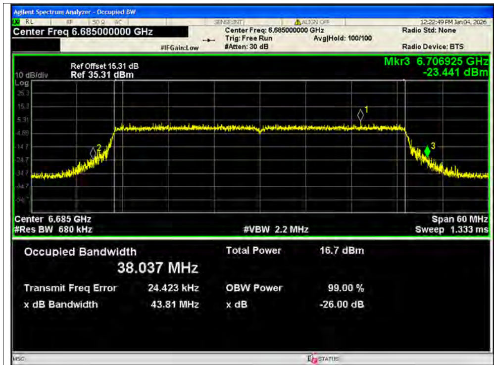
-26dB Bandwidth NVNT ax40 6685MHz Ant1 SISO
