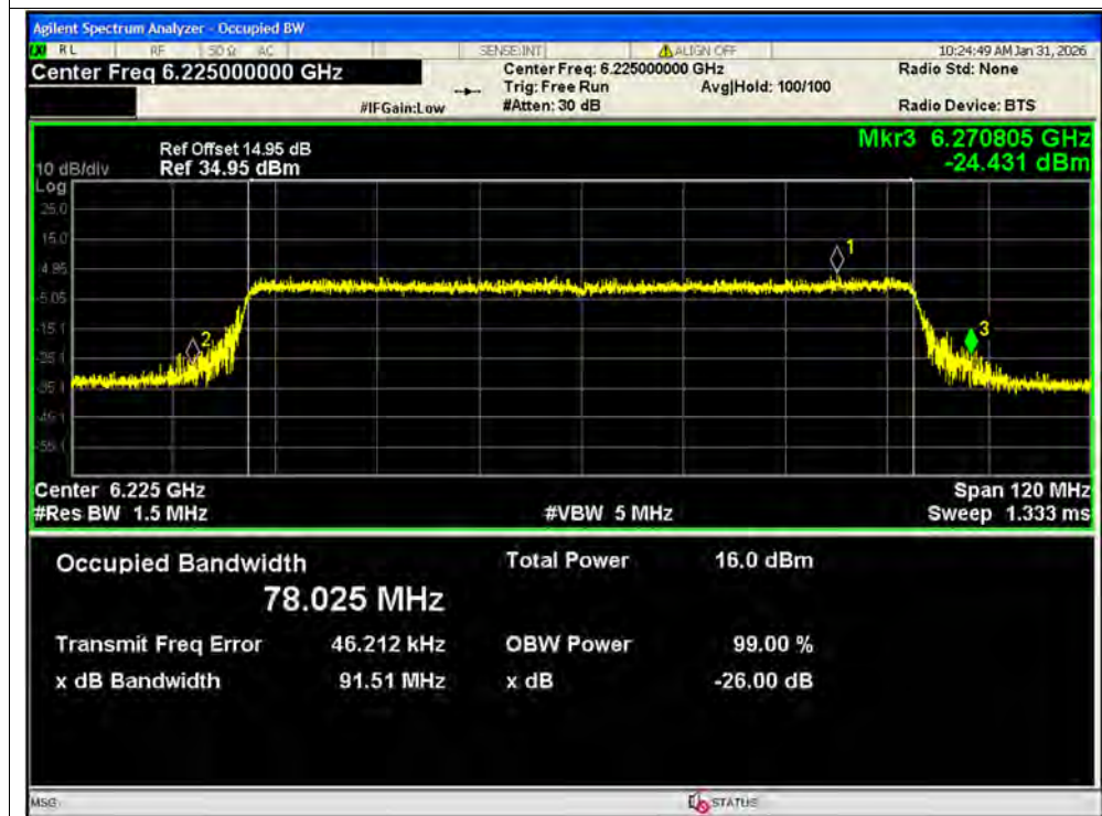
-26dB Bandwidth NVNT ax80 6225MHz Ant2 MIMO
