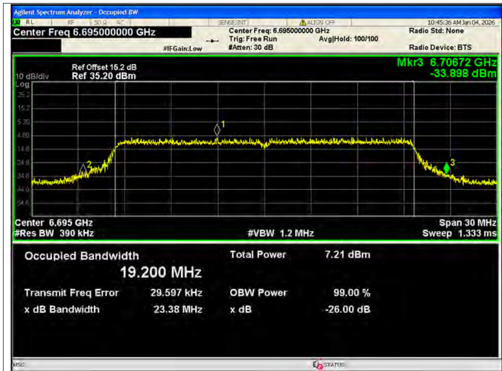
-26dB Bandwidth NVNT ax20 6695MHz Ant1 MIMO
