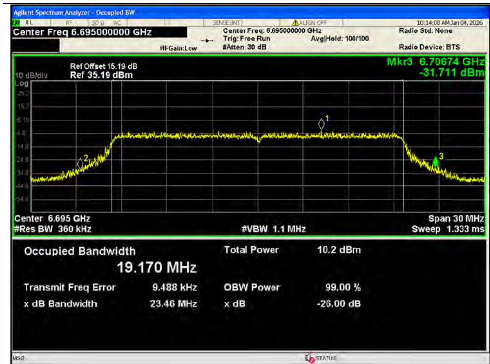
-26dB Bandwidth NVNT ax20 6695MHz Ant2 SISO
