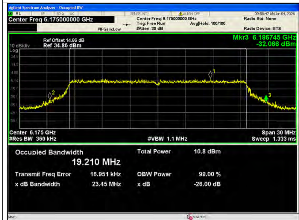
-26dB Bandwidth NVNT ax20 6175MHz Ant2 SISO
