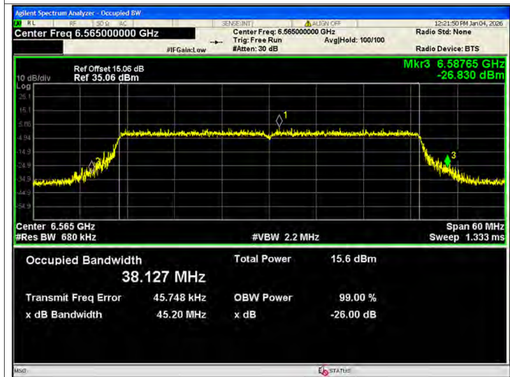
-26dB Bandwidth NVNT ax40 6565MHz Ant1 SISO
