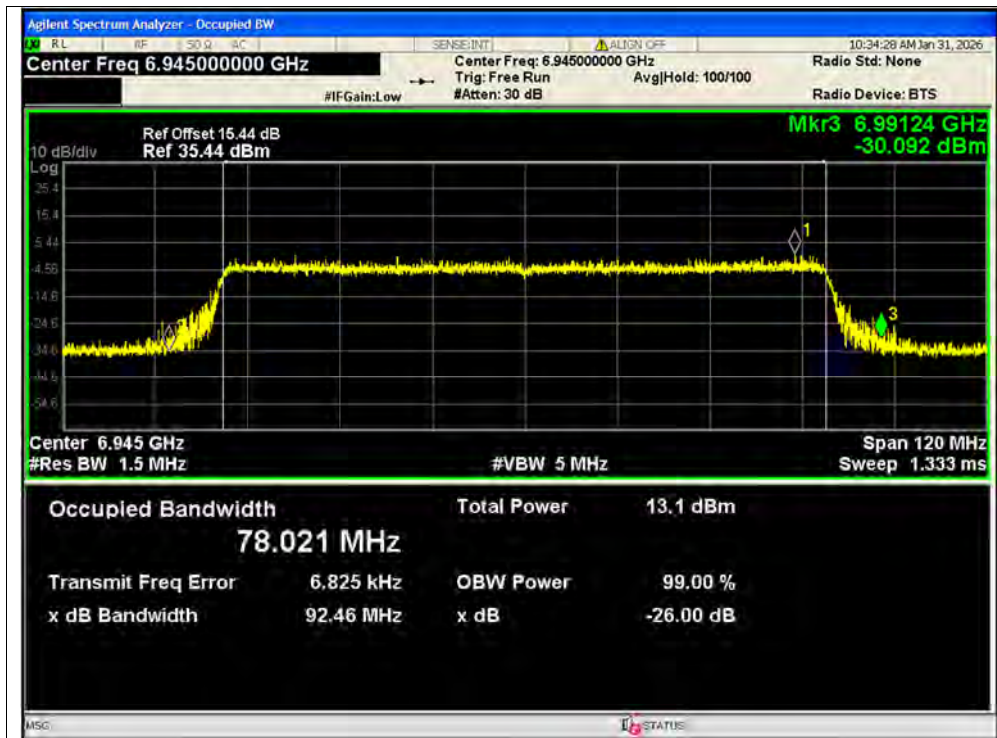
-26dB Bandwidth NVNT ax80 6945MHz Ant1 MIMO
