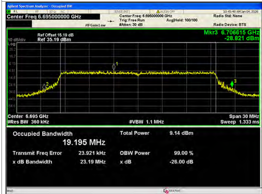
-26dB Bandwidth NVNT ax20 6695MHz Ant2 MIMO
