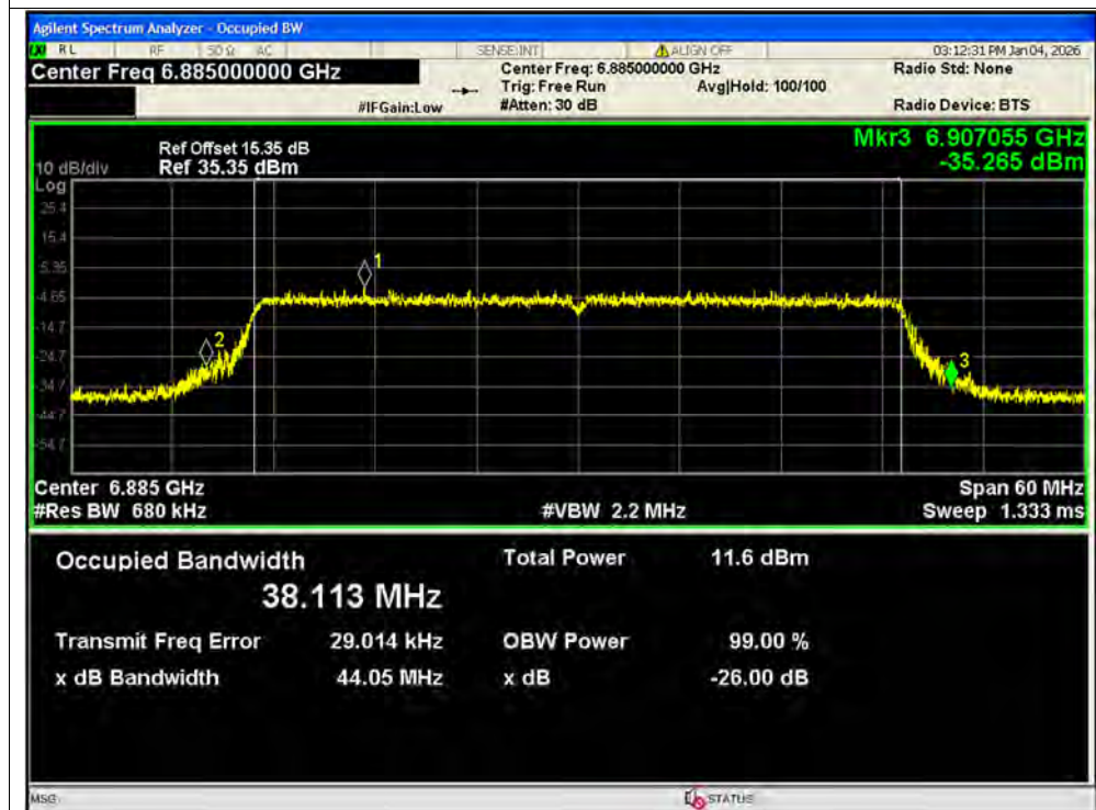
-26dB Bandwidth NVNT ax40 6885MHz Ant2 MIMO
