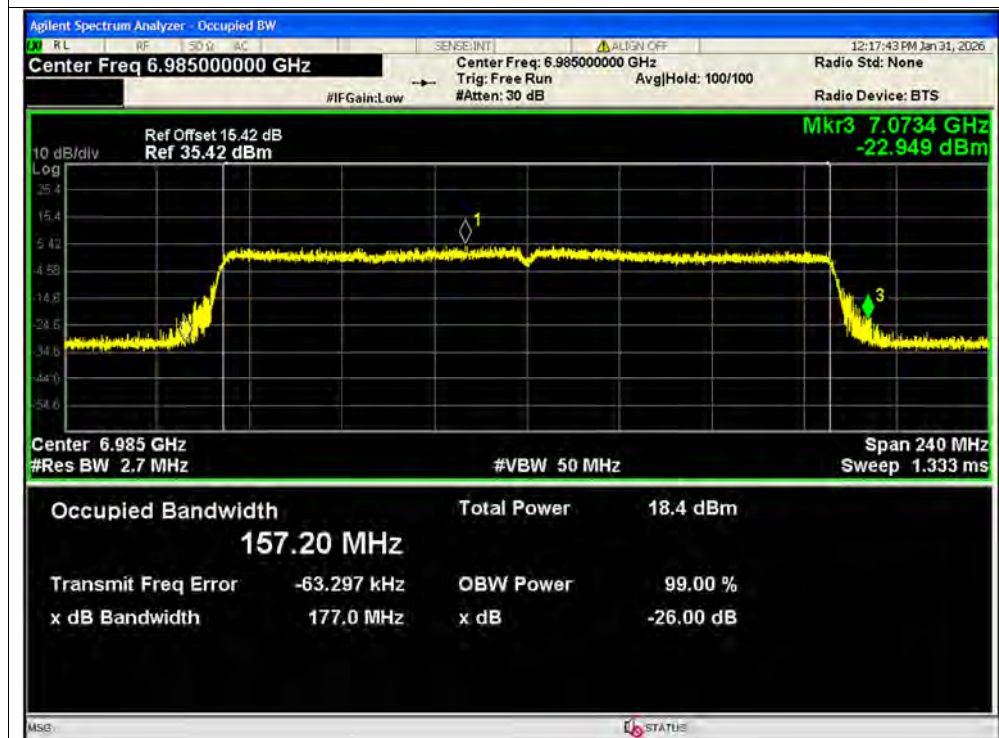
-26dB Bandwidth NVNT ax160 6985MHz Ant2 SISO
