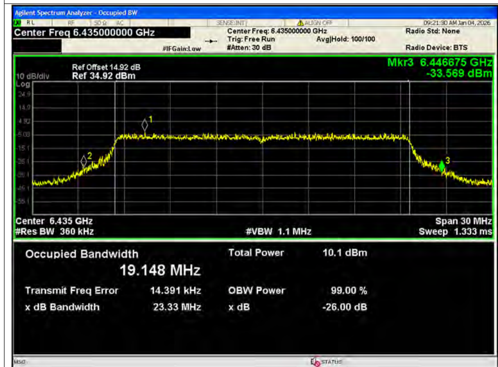
-26dB Bandwidth NVNT ax20 6435MHz Ant1 SISO
