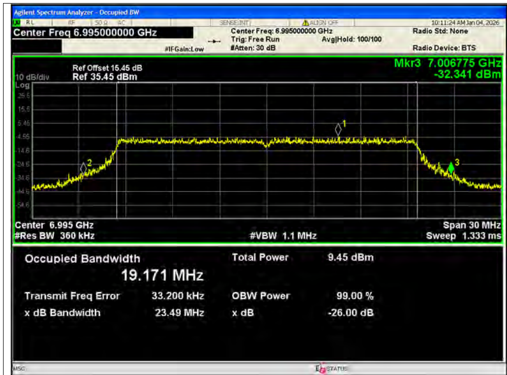
-26dB Bandwidth NVNT ax20 6995MHz Ant2 SISO
