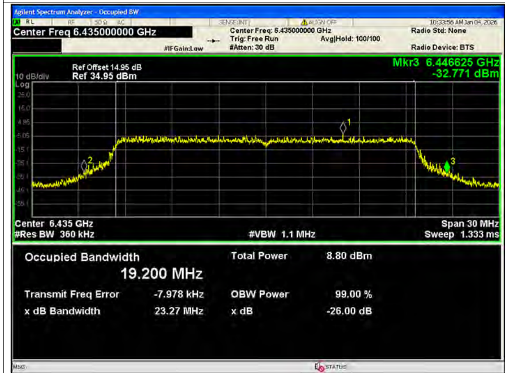
-26dB Bandwidth NVNT ax20 6435MHz Ant2 MIMO
