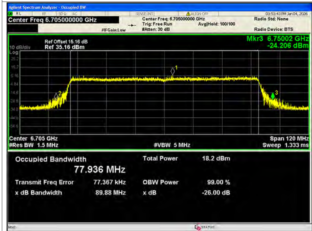
-26dB Bandwidth NVNT ax80 6705MHz Ant1 SISO
