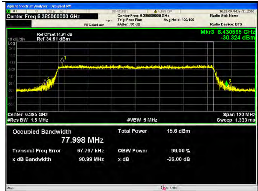
-26dB Bandwidth NVNT ax80 6385MHz Ant2 MIMO
