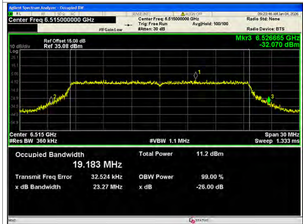
-26dB Bandwidth NVNT ax20 6515MHz Ant1 SISO
