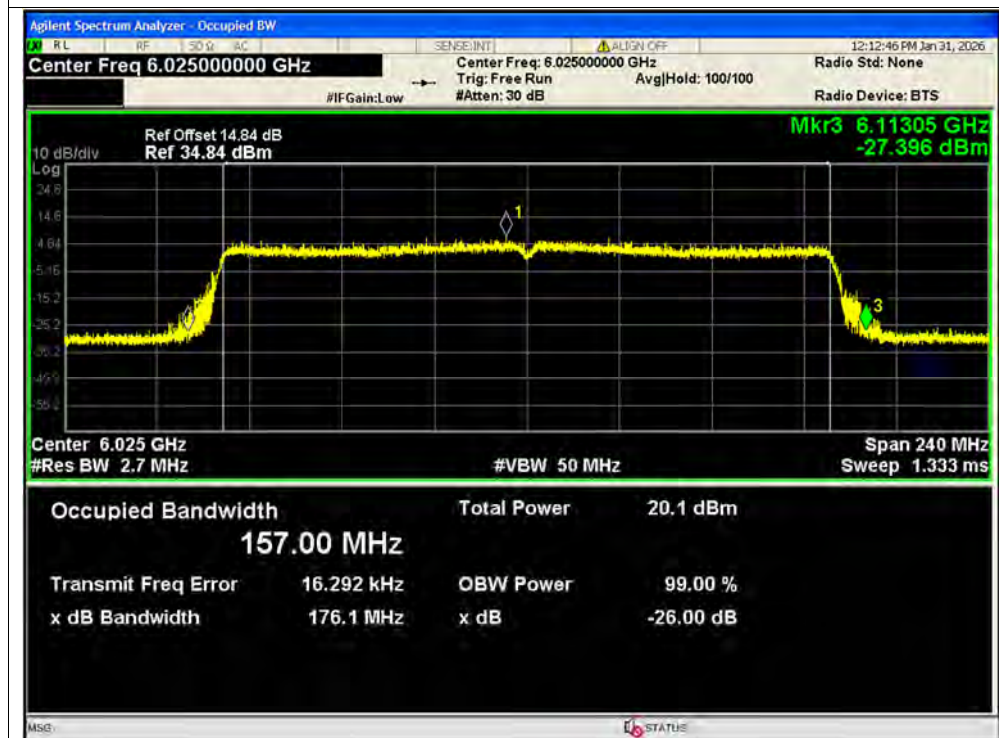
-26dB Bandwidth NVNT ax160 6025MHz Ant2 SISO
