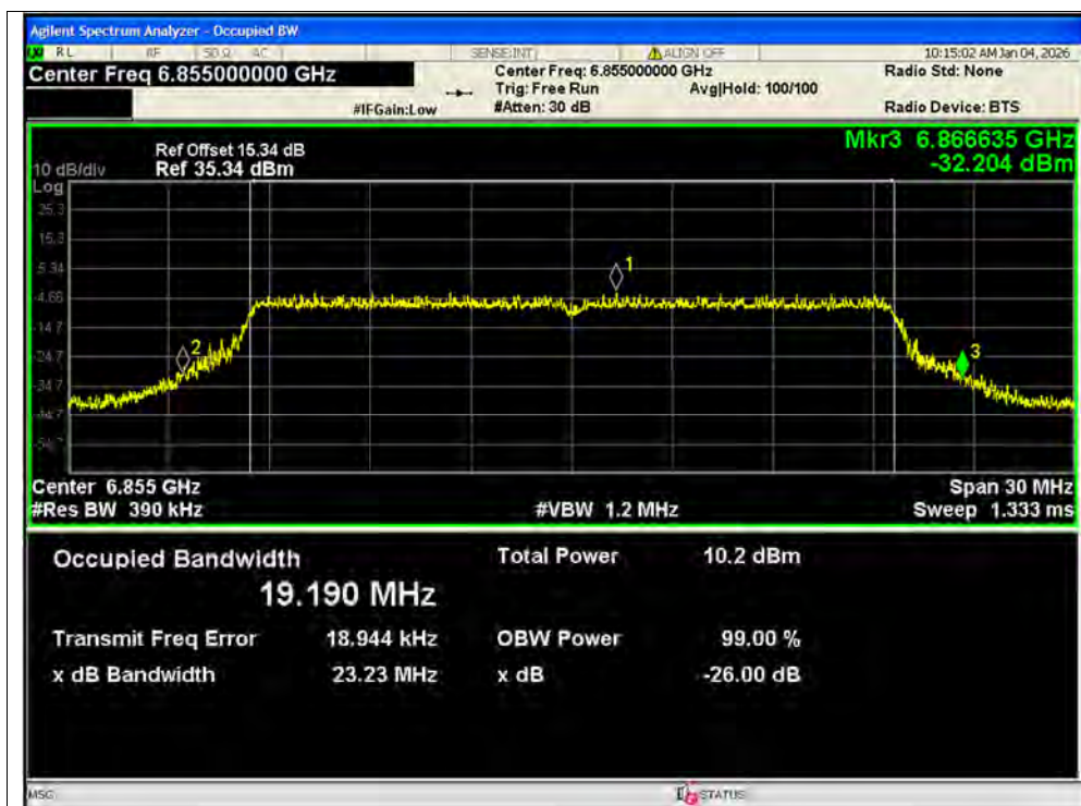
-26dB Bandwidth NVNT ax20 6855MHz Ant2 SISO
