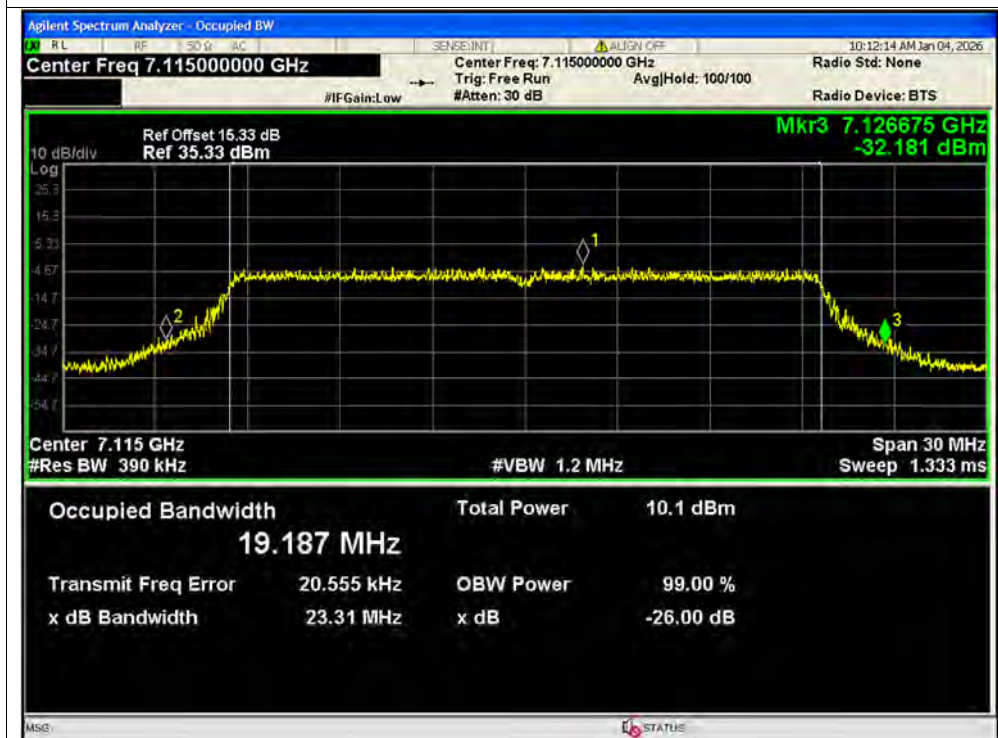
-26dB Bandwidth NVNT ax20 7115MHz Ant2 SISO
