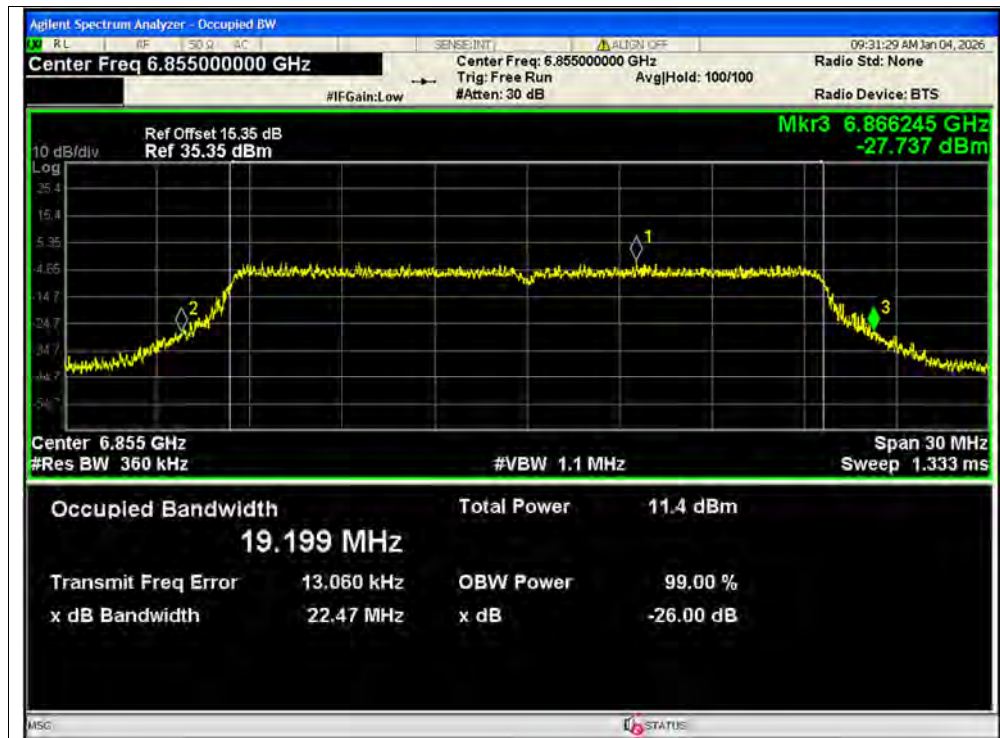
-26dB Bandwidth NVNT ax20 6855MHz Ant1 SISO
