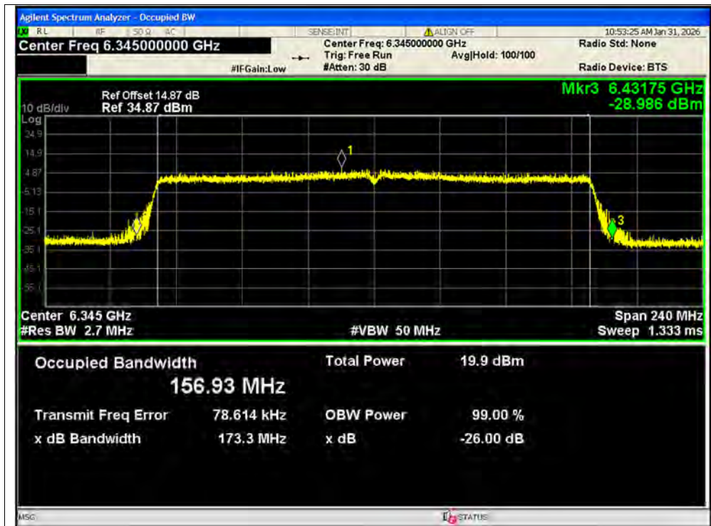
-26dB Bandwidth NVNT ax160 6345MHz Ant1 SISO
