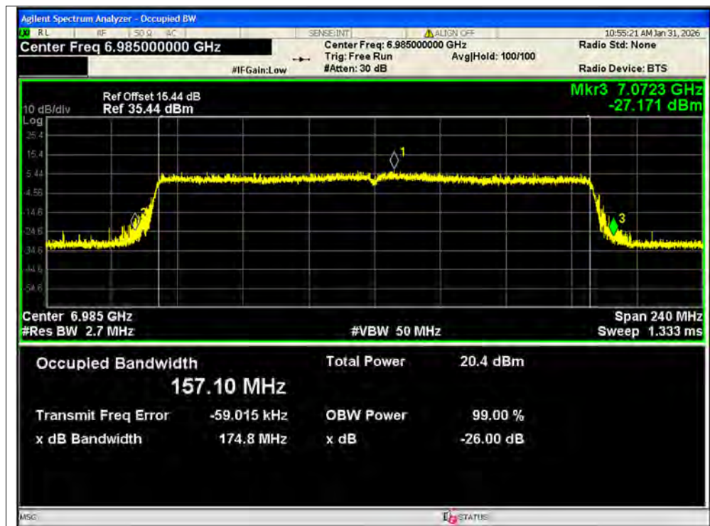
-26dB Bandwidth NVNT ax160 6985MHz Ant1 SISO
