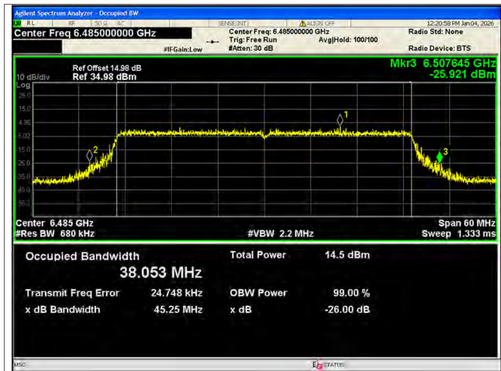
-26dB Bandwidth NVNT ax40 6485MHz Ant1 SISO
