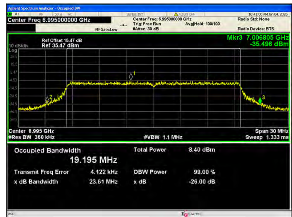
-26dB Bandwidth NVNT ax20 6995MHz Ant1 MIMO
