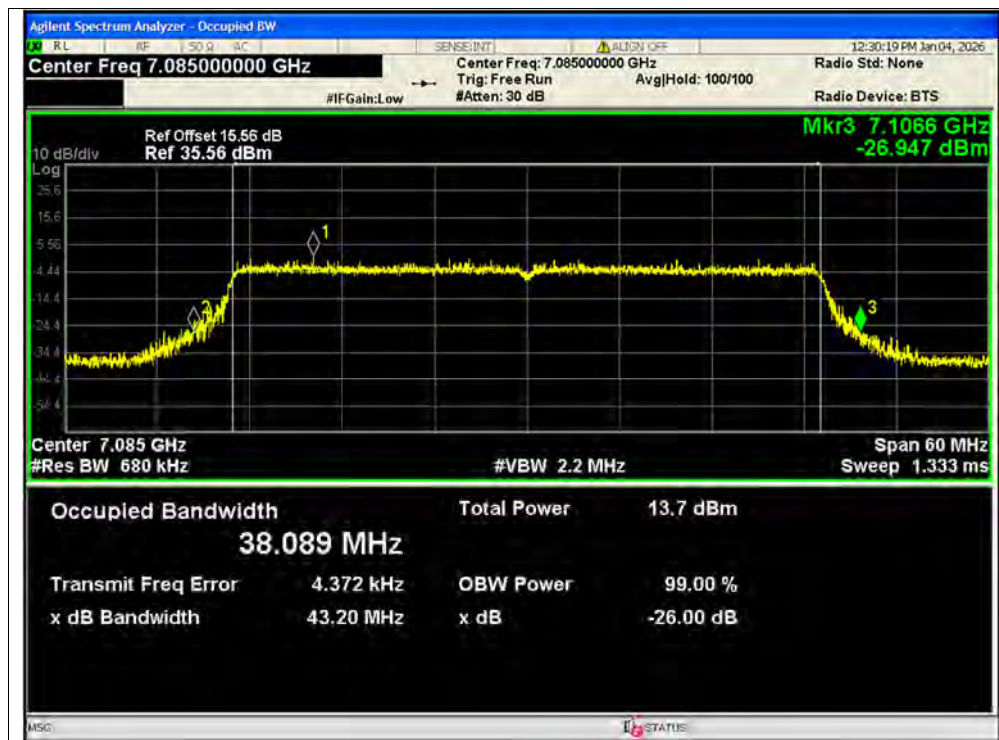
-26dB Bandwidth NVNT ax40 7085MHz Ant1 SISO
