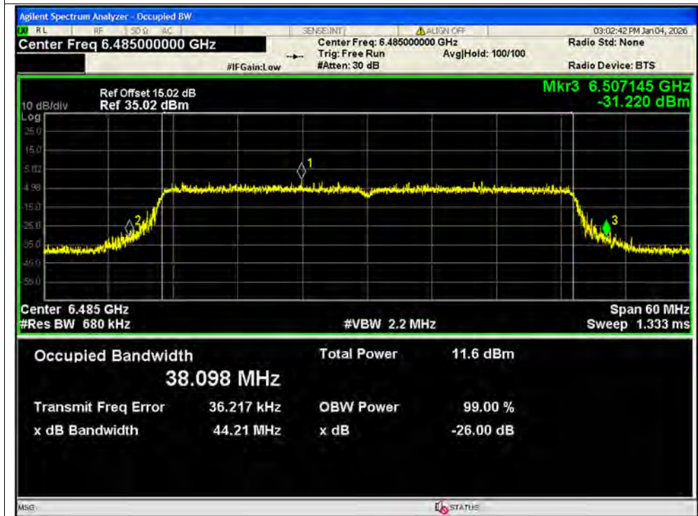
-26dB Bandwidth NVNT ax40 6485MHz Ant2 MIMO
