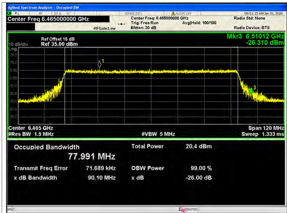
-26dB Bandwidth NVNT ax80 6465MHz Ant2 SISO
