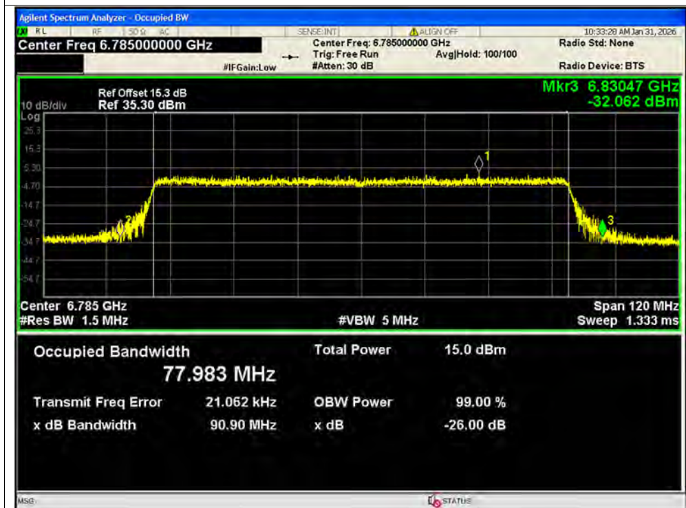
-26dB Bandwidth NVNT ax80 6785MHz Ant2 MIMO
