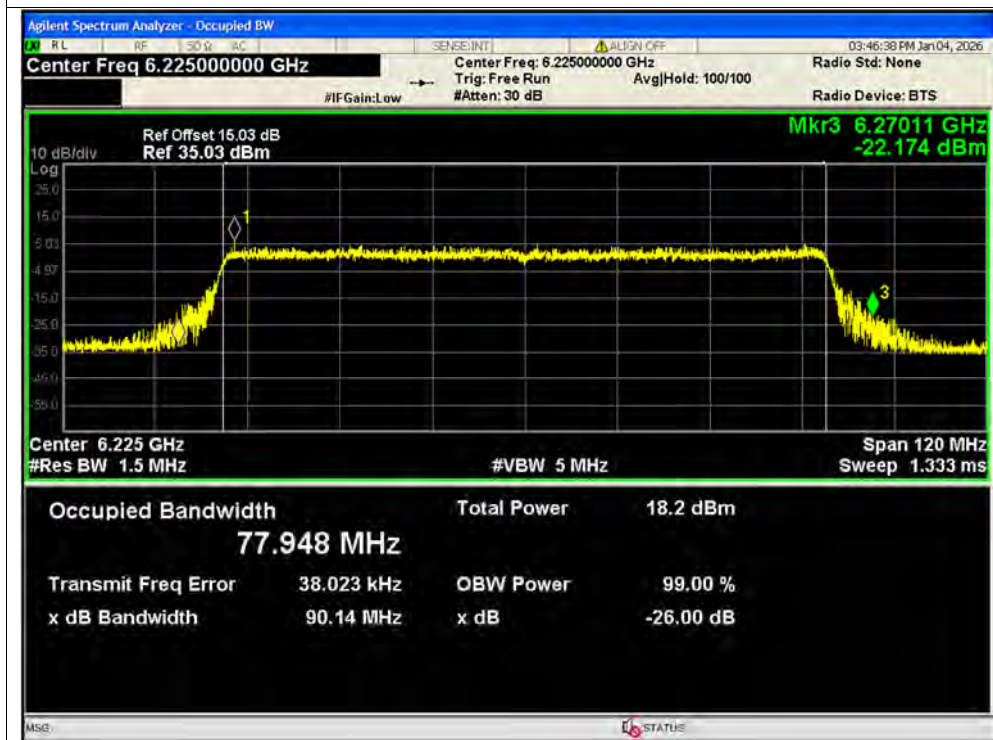
-26dB Bandwidth NVNT ax80 6225MHz Ant1 SISO
