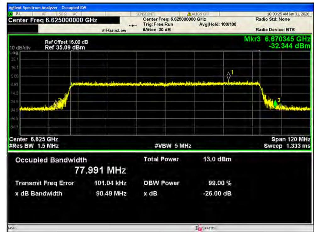
-26dB Bandwidth NVNT ax80 6625MHz Ant1 MIMO
