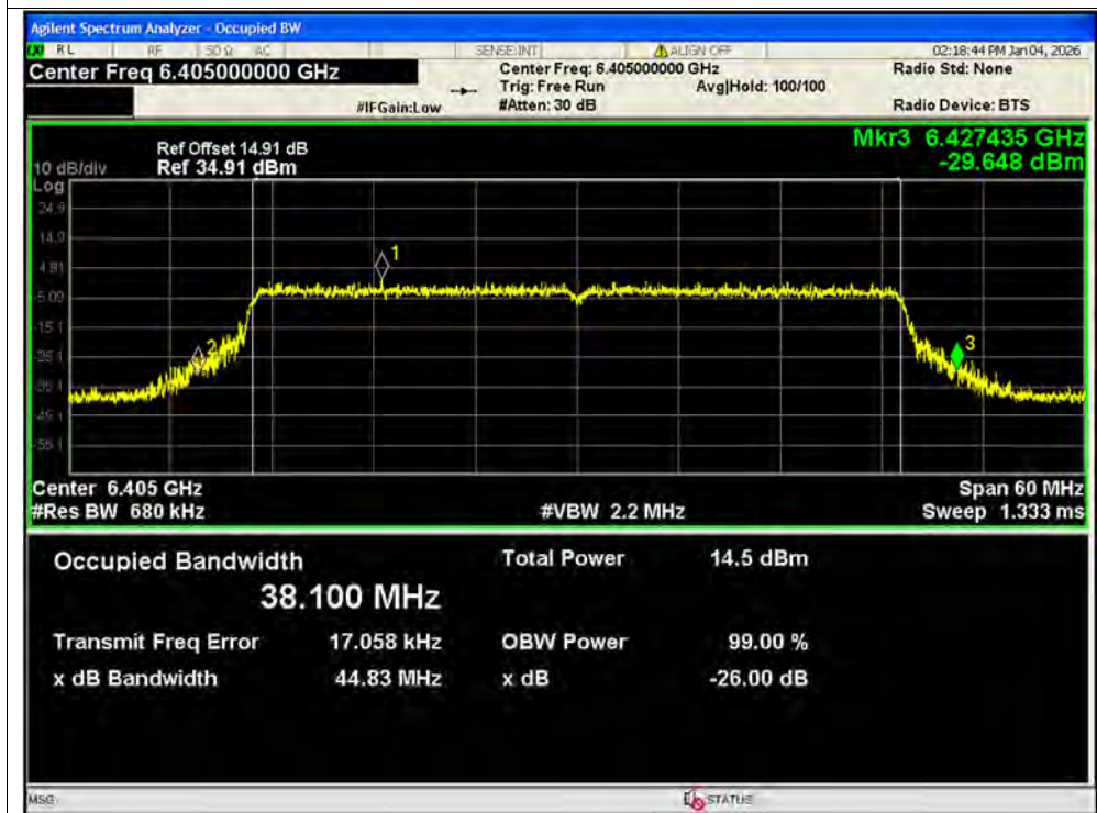
-26dB Bandwidth NVNT ax40 6405MHz Ant2 SISO
