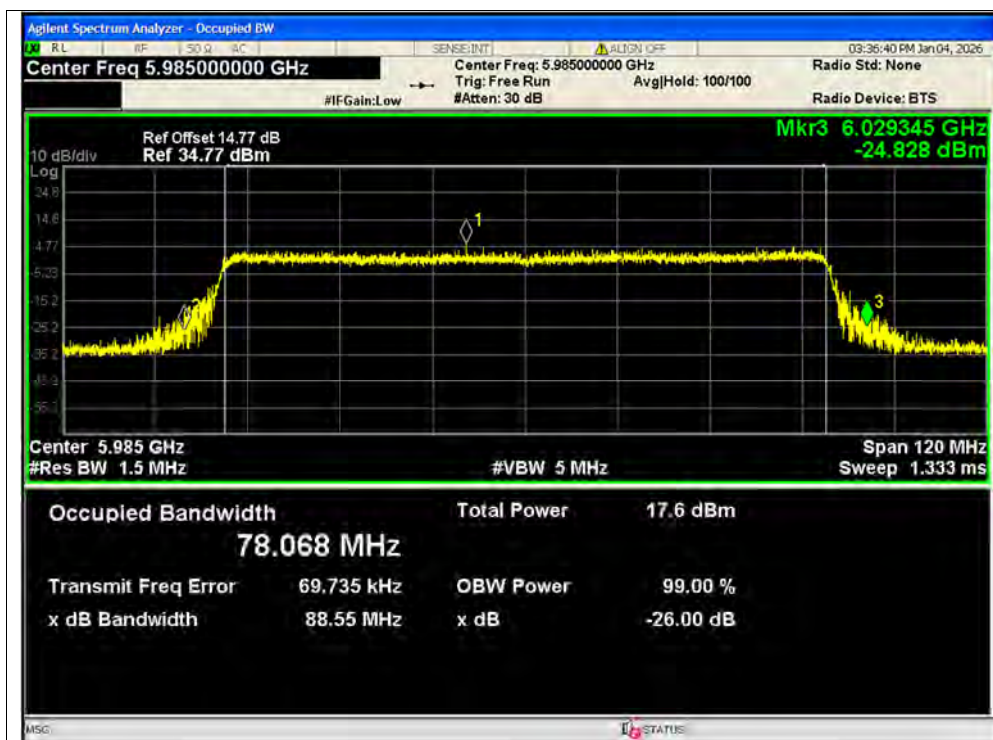
-26dB Bandwidth NVNT ax80 5985MHz Ant1 SISO
