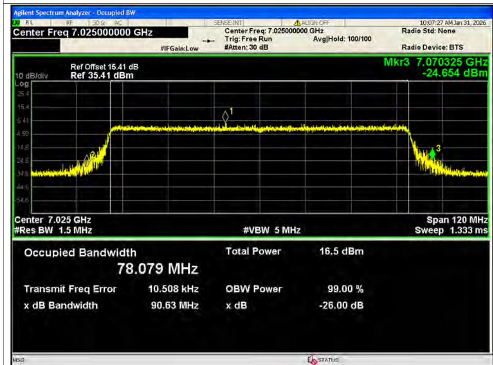
-26dB Bandwidth NVNT ax80 7025MHz Ant2 SISO
