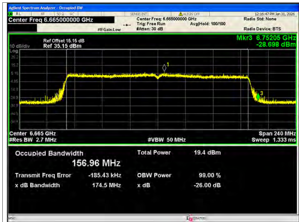
-26dB Bandwidth NVNT ax160 6665MHz Ant2 SISO
