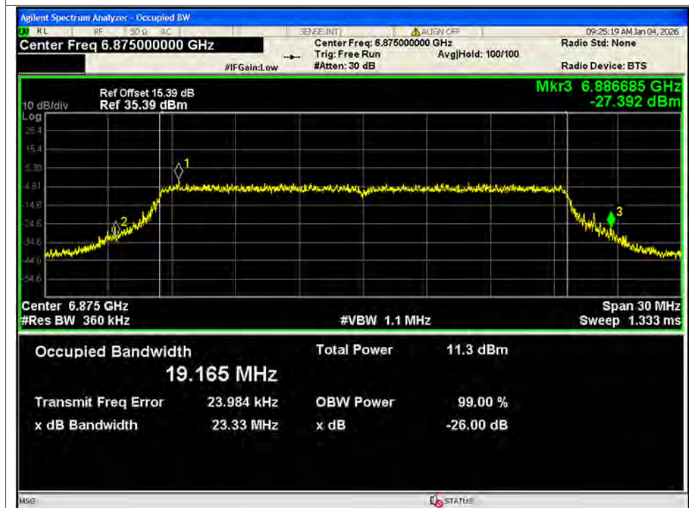
-26dB Bandwidth NVNT ax20 6875MHz Ant1 SISO
