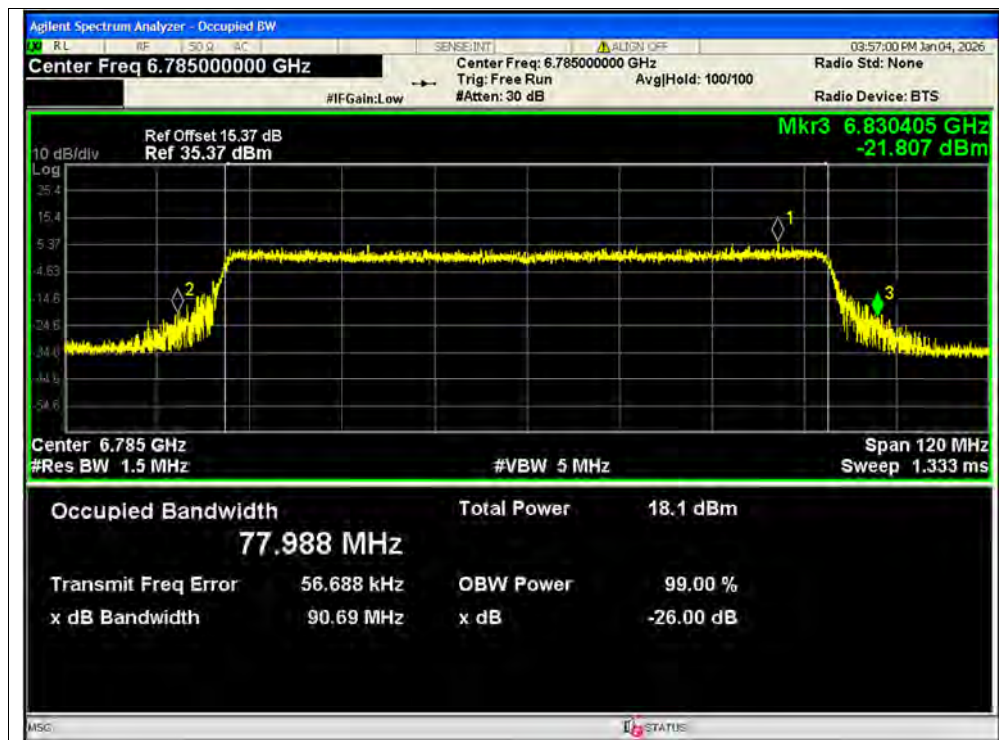
-26dB Bandwidth NVNT ax80 6785MHz Ant1 SISO
