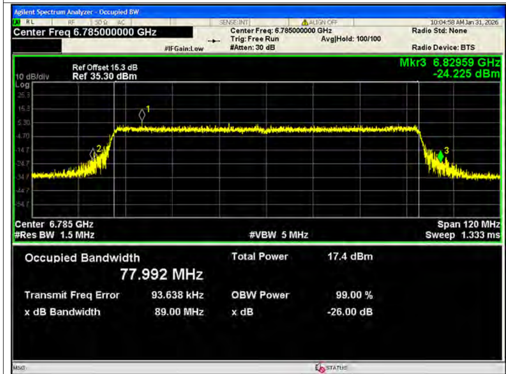
-26dB Bandwidth NVNT ax80 6785MHz Ant2 SISO
