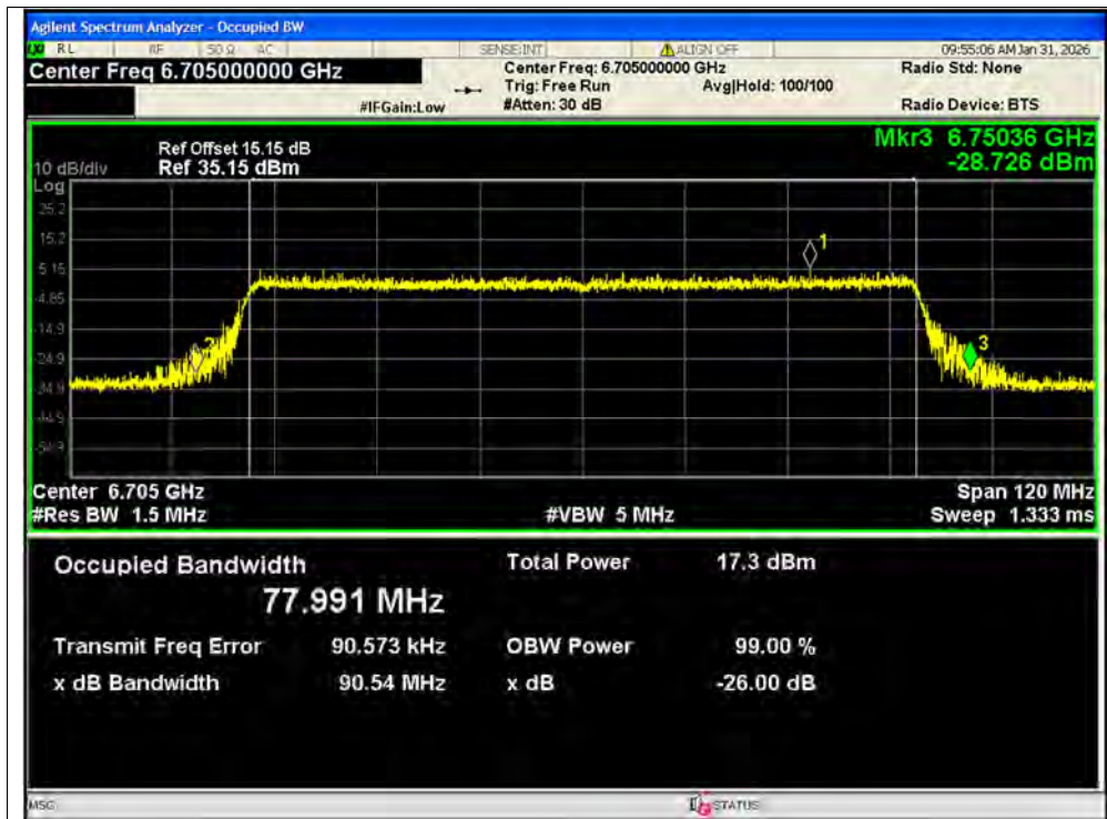
-26dB Bandwidth NVNT ax80 6705MHz Ant2 SISO
