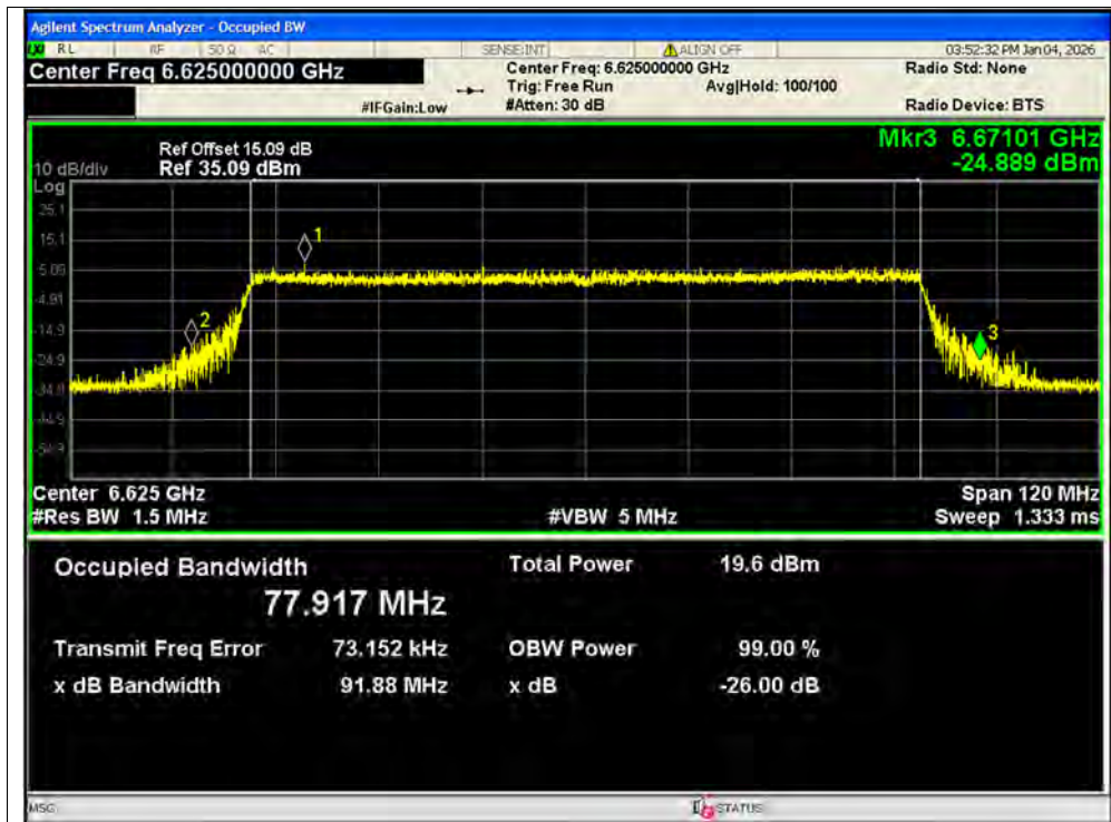
-26dB Bandwidth NVNT ax80 6625MHz Ant1 SISO
