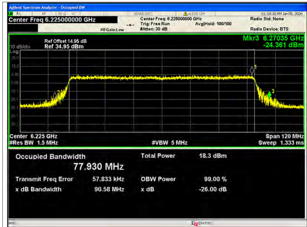
-26dB Bandwidth NVNT ax80 6225MHz Ant2 SISO
