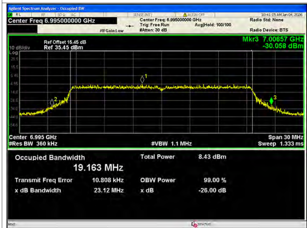
-26dB Bandwidth NVNT ax20 6995MHz Ant2 MIMO
