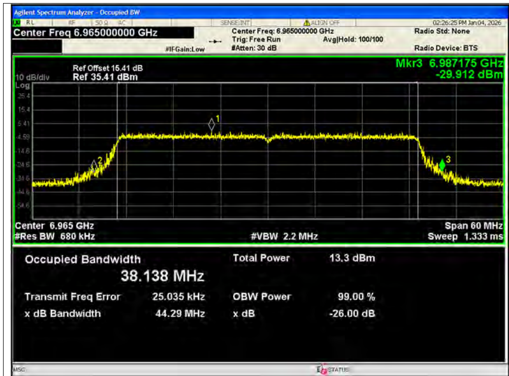
-26dB Bandwidth NVNT ax40 6965MHz Ant2 SISO
