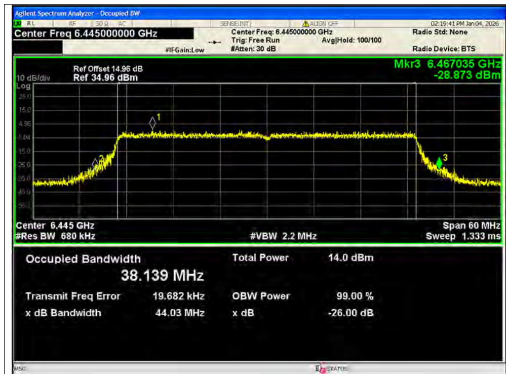
-26dB Bandwidth NVNT ax40 6445MHz Ant2 SISO
