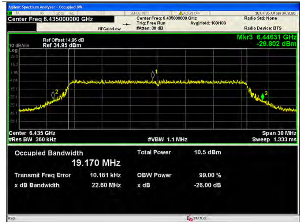
-26dB Bandwidth NVNT ax20 6435MHz Ant2 SISO
