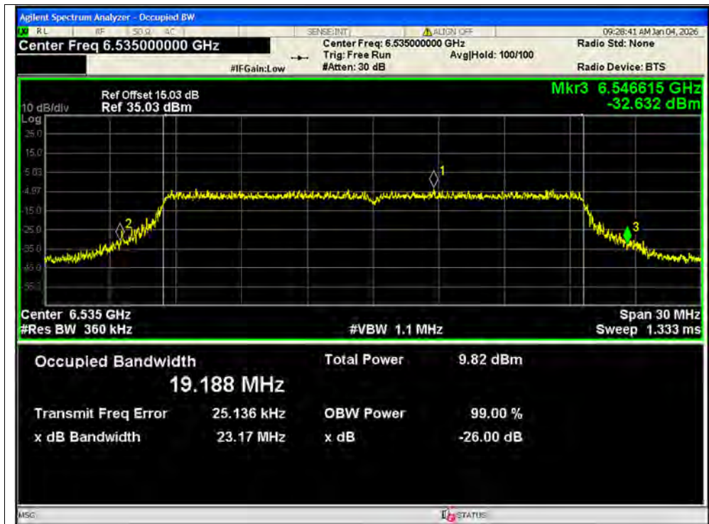
-26dB Bandwidth NVNT ax20 6535MHz Ant1 SISO
