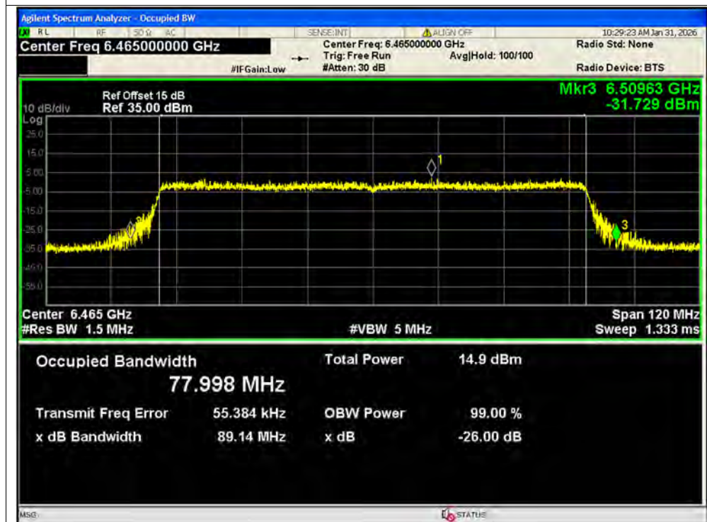
-26dB Bandwidth NVNT ax80 6465MHz Ant2 MIMO
