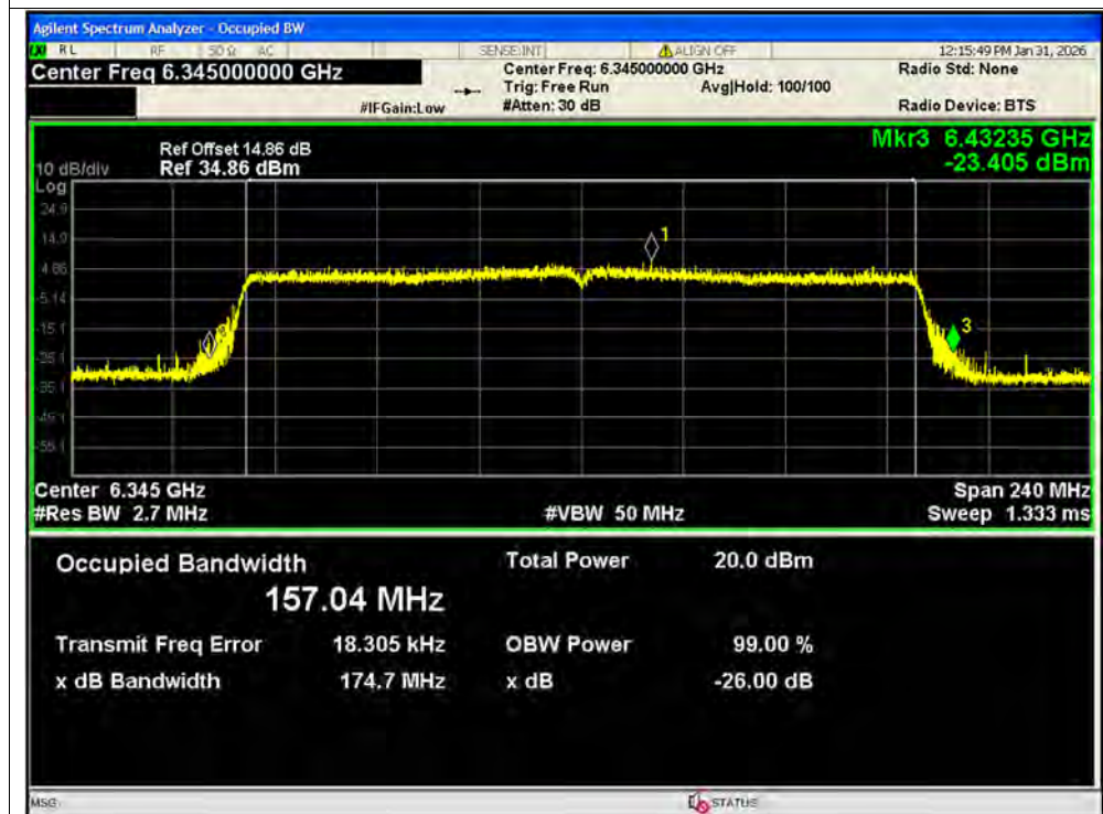
-26dB Bandwidth NVNT ax160 6345MHz Ant2 SISO
