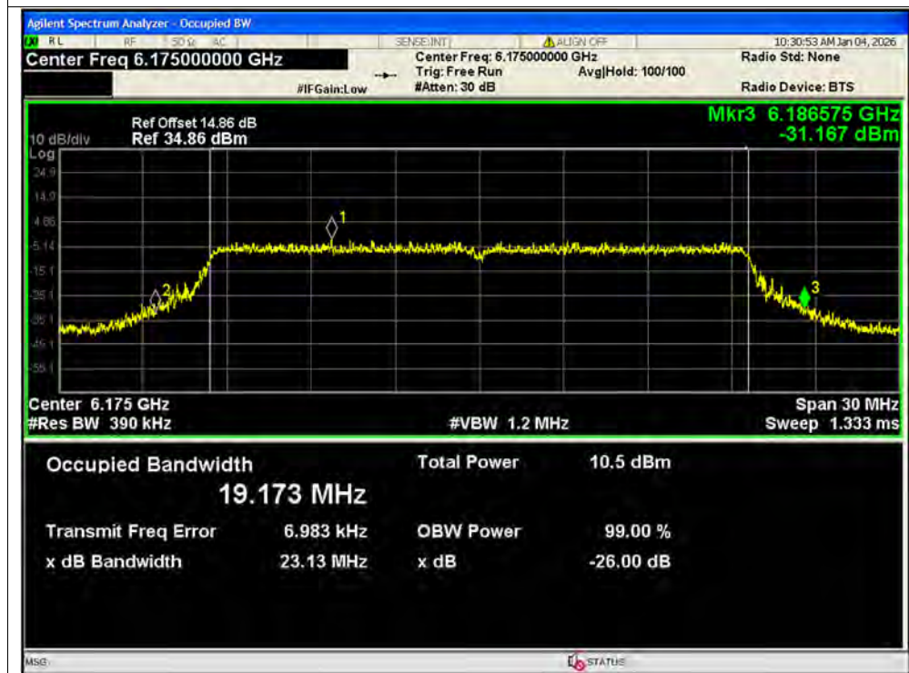
-26dB Bandwidth NVNT ax20 6175MHz Ant2 MIMO
