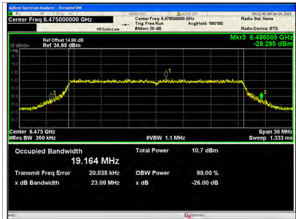
-26dB Bandwidth NVNT ax20 6475MHz Ant1 SISO
