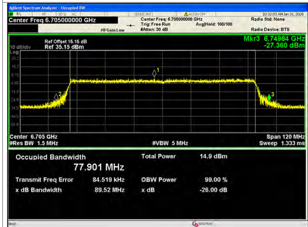
-26dB Bandwidth NVNT ax80 6705MHz Ant2 MIMO
