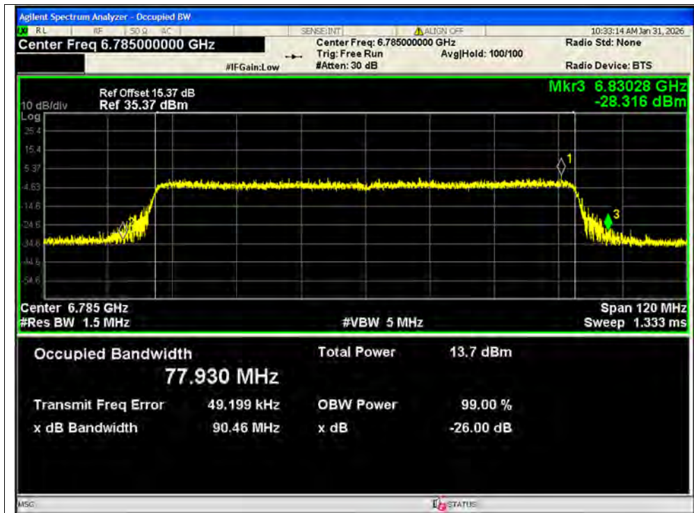
-26dB Bandwidth NVNT ax80 6785MHz Ant1 MIMO
