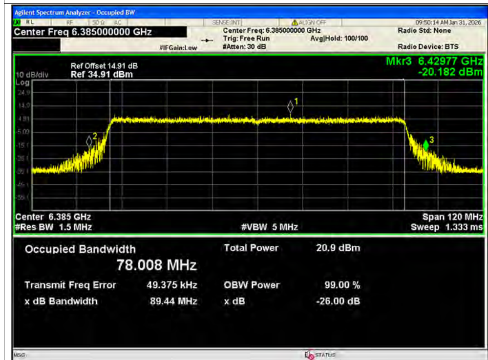
-26dB Bandwidth NVNT ax80 6385MHz Ant2 SISO
