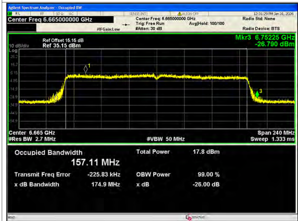
-26dB Bandwidth NVNT ax160 6665MHz Ant2 MIMO
