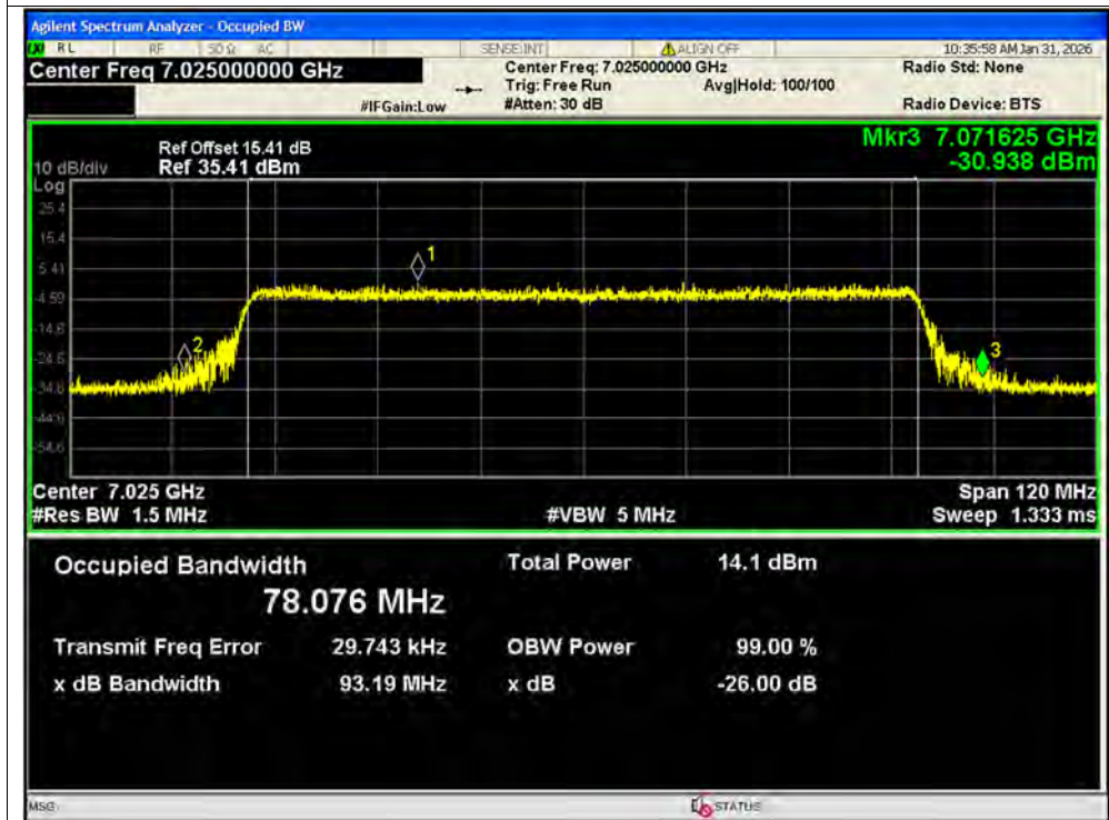
-26dB Bandwidth NVNT ax80 7025MHz Ant2 MIMO
