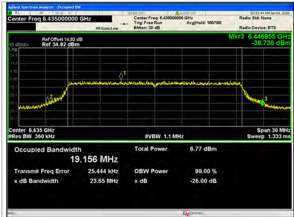
-26dB Bandwidth NVNT ax20 6435MHz Ant1 MIMO
