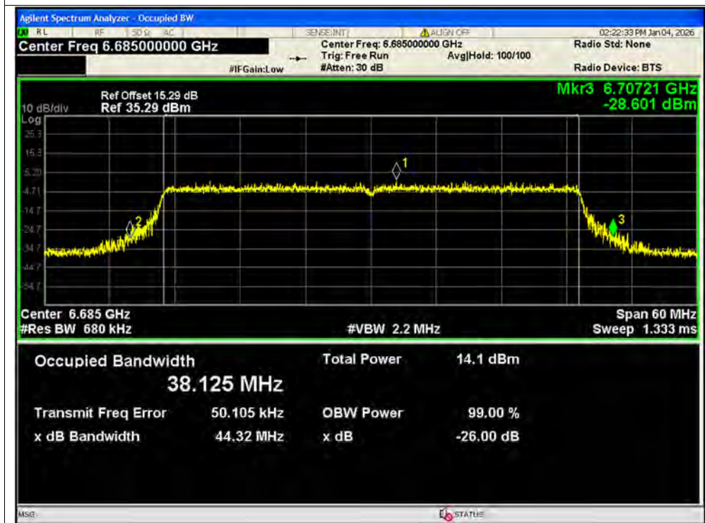
-26dB Bandwidth NVNT ax40 6685MHz Ant2 SISO
