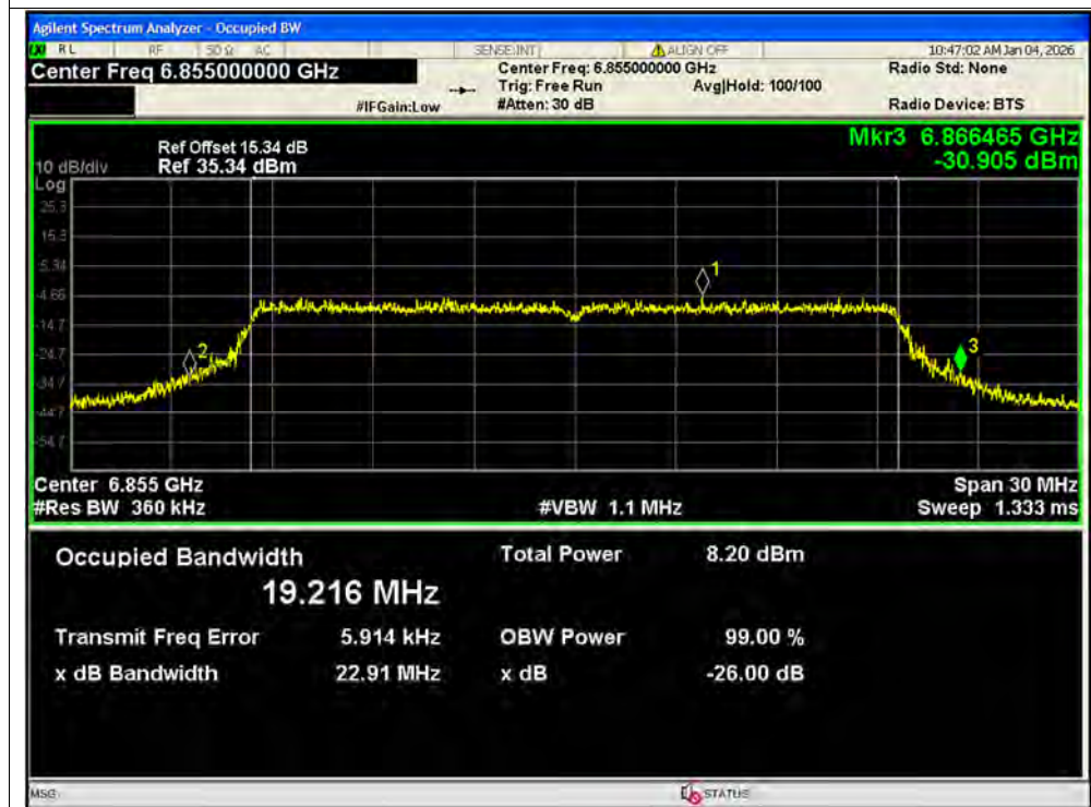
-26dB Bandwidth NVNT ax20 6855MHz Ant2 MIMO
