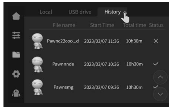
⑤ History
