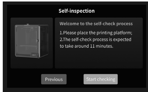
④ Self-inspection
