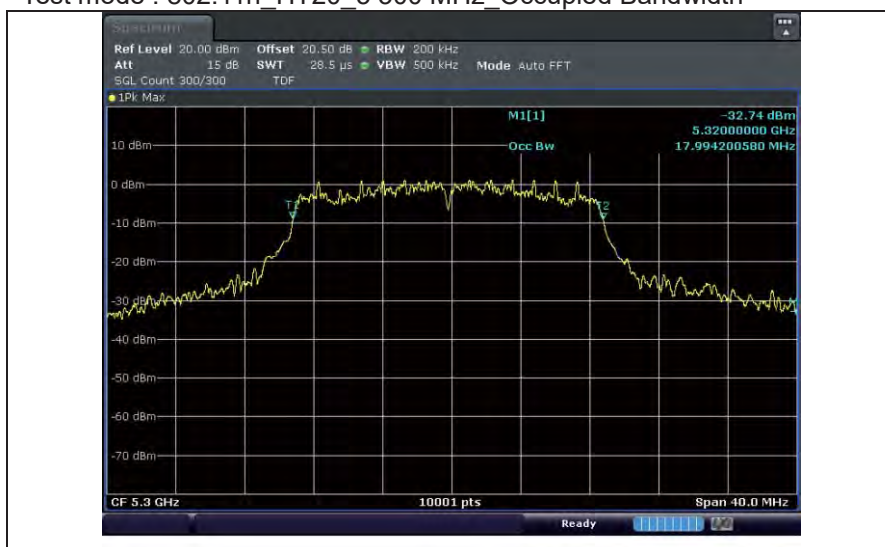
Test mode : 802.11n HT20 5 320 MHz Occupied Bandwidth
