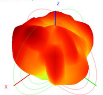
5750.0MHz H+V, Eff: 47.4%
