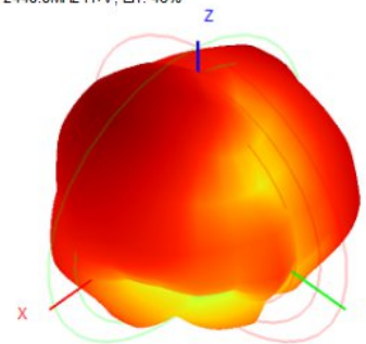
2440.0MHz H+V, Eff: 46%
