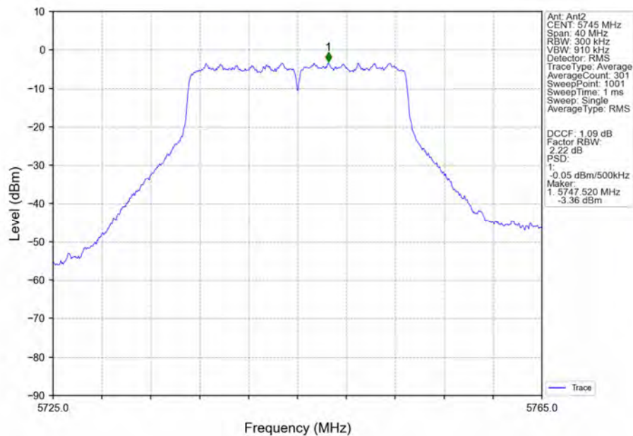
802.11ac(VHT20)_LCH_5745MHz_Ant2_NTNV
