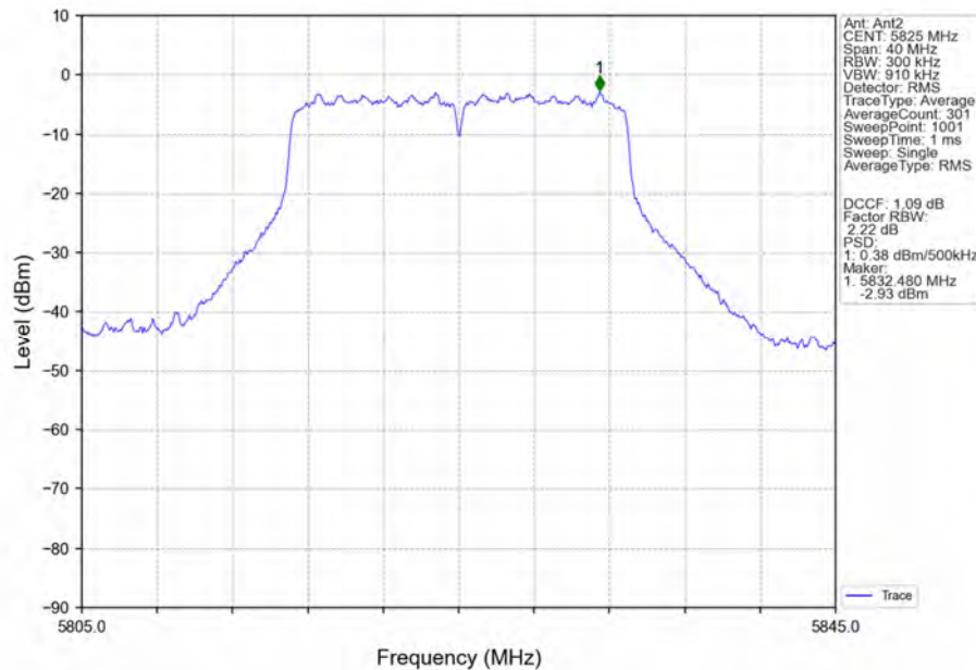
802.11ac(VHT20)_HCH_5825MHz_Ant2_NTNV
