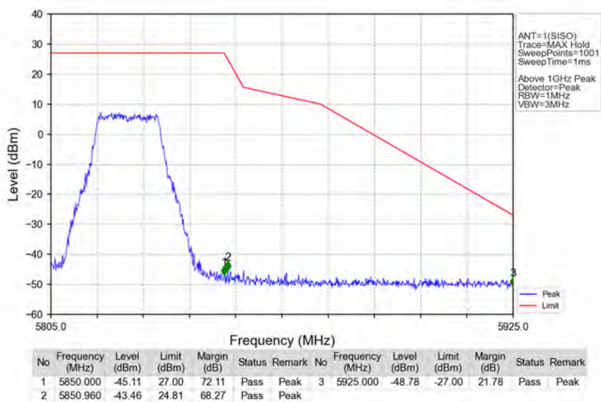
802.11a_HCH_5825MHz_Ant1_NTNV
