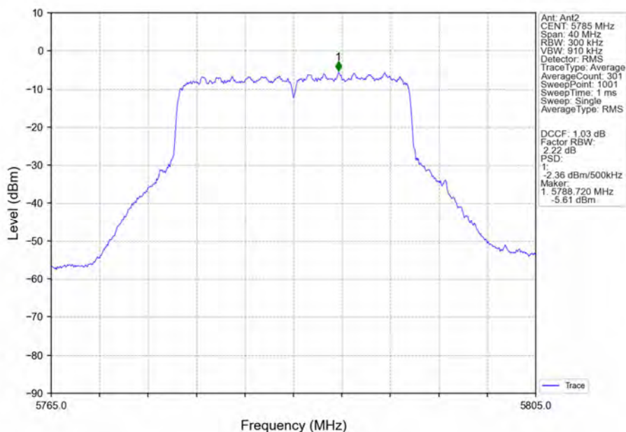
802.11ax(HEW20)_MCH_5785MHz_SU_ / _Ant2_NTNV
