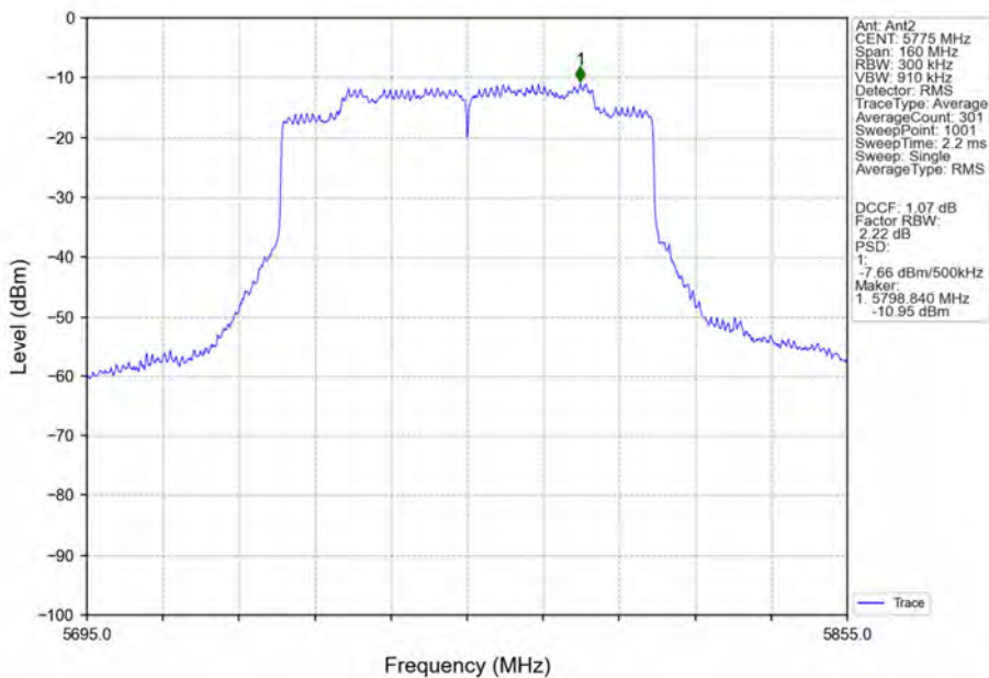
802.11ax(HEW80)_MCH_5775MHz_SU_ / Ant2_NTNV
