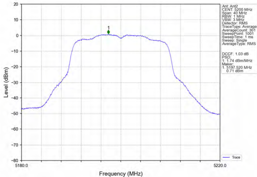
802.11ax(HEW20)_MCH_5200MHz_SU_ / Ant2_NTNV
