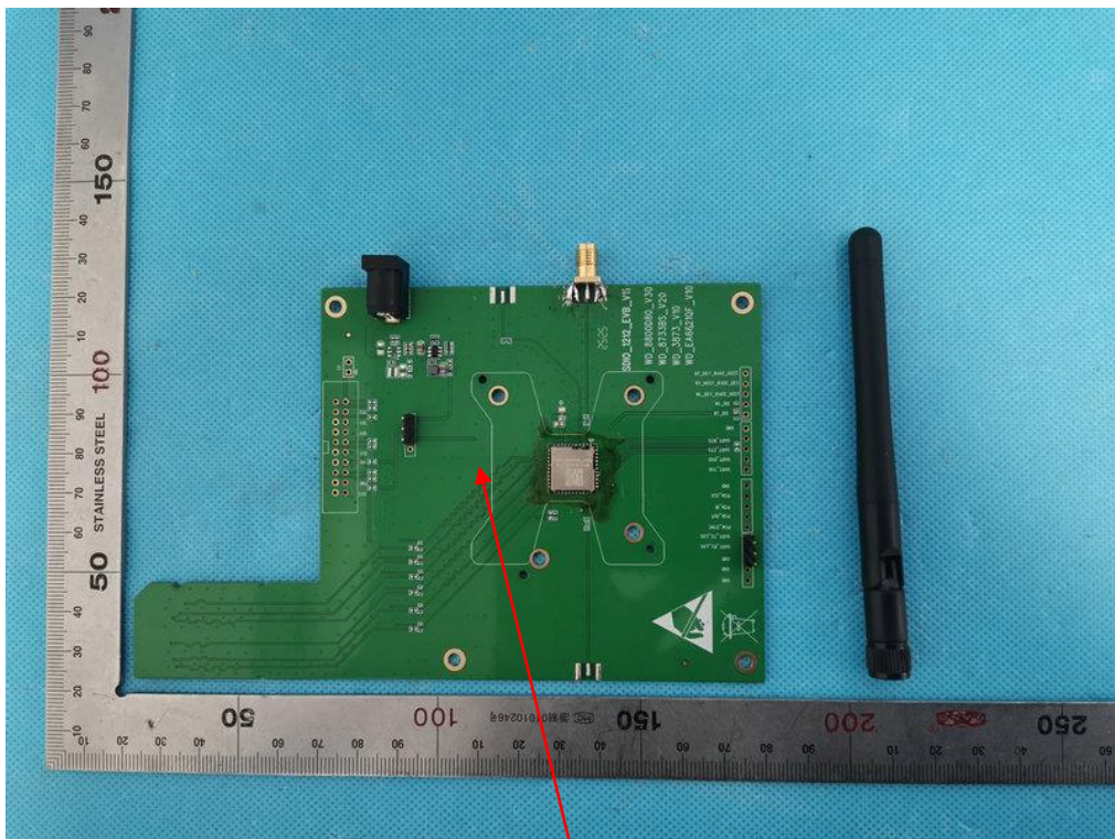
Test base plate
