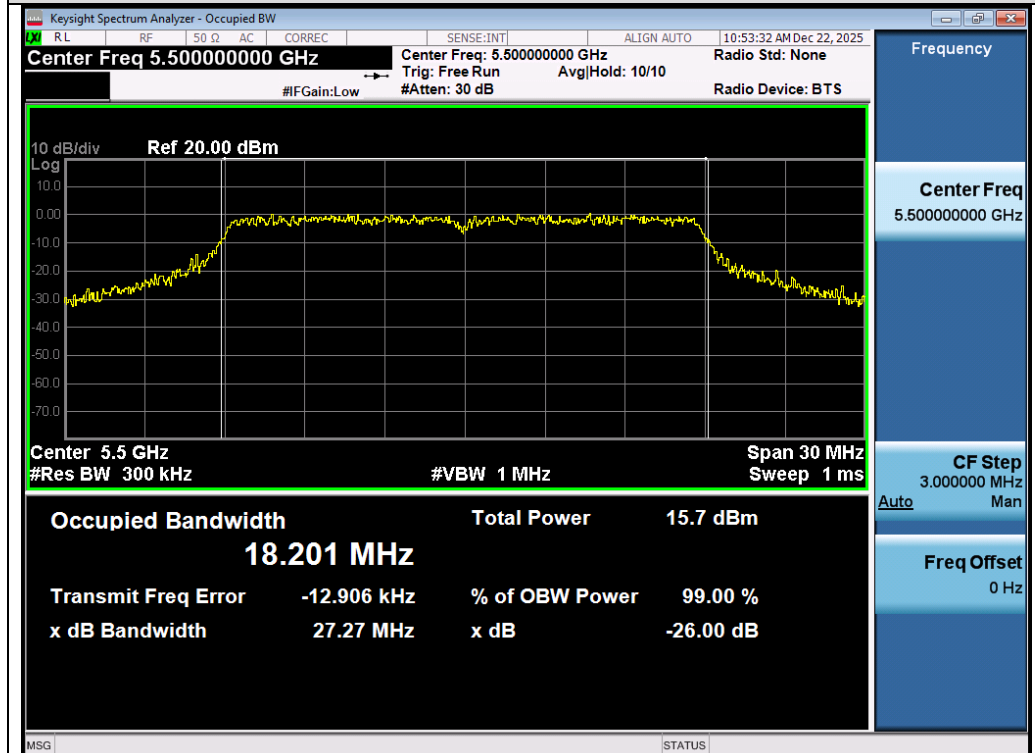
Test_Graph_802.11n20_ANT1_5500_MCS0_OBW
