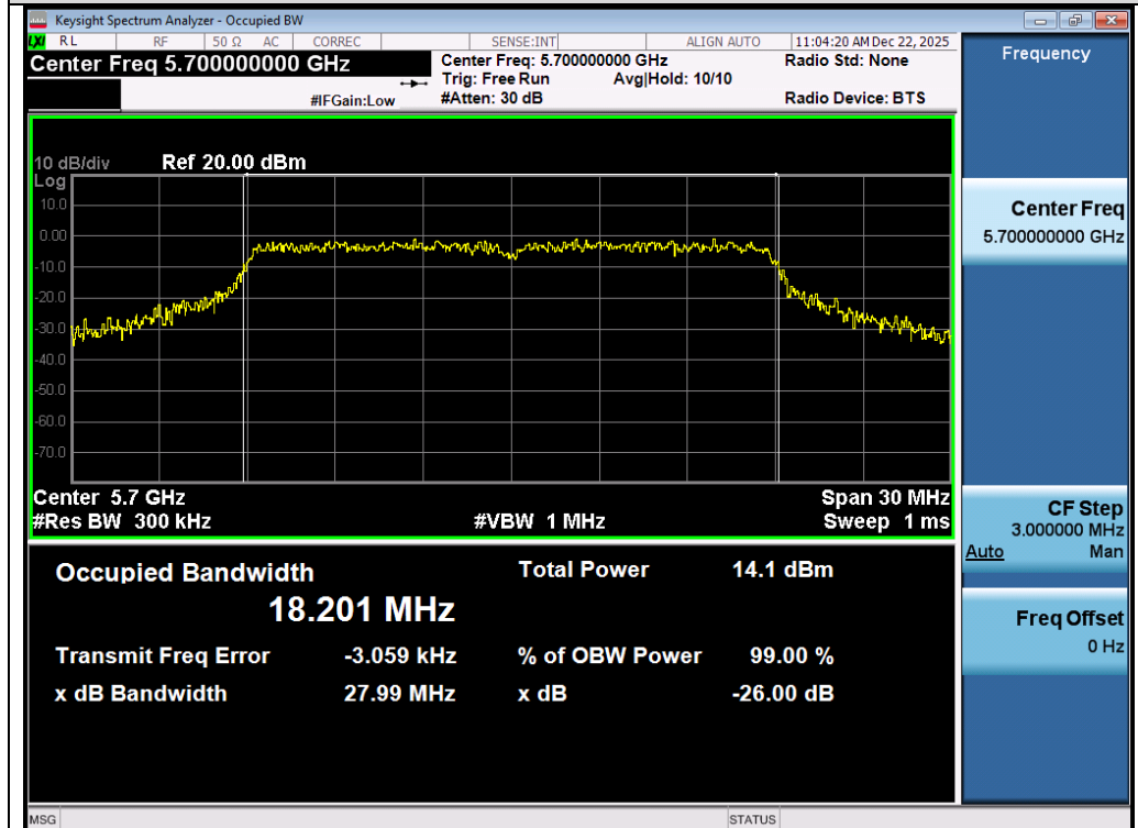
Test_Graph_802.11ac20_ANT1_5700_MCS0_OBW
