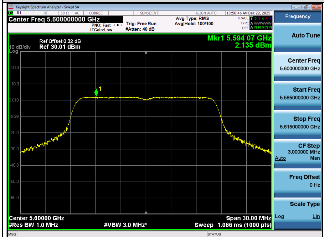
Test_Graph_802.11a_ANT1_5600_6Mbps_PSD
