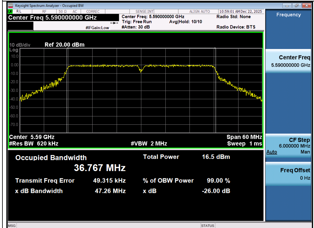
Test_Graph_802.11n40_ANT1_5590_MCS0_OBW
