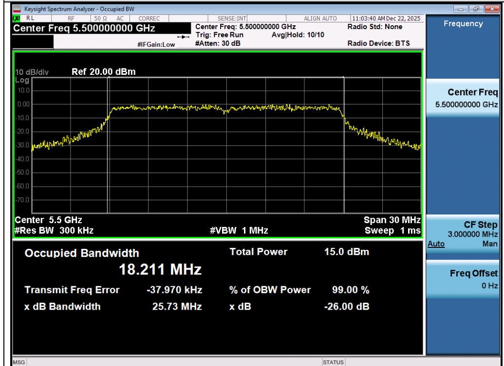
Test_Graph_802.11ac20_ANT1_5500_MCS0_OBW
