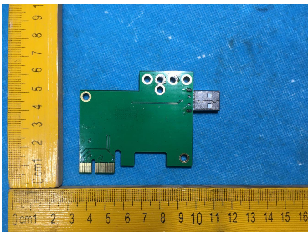
Eut in Test Fixture
