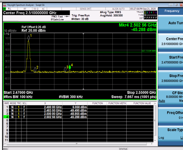
BLE_BT4.2_Ant1_High_2480
