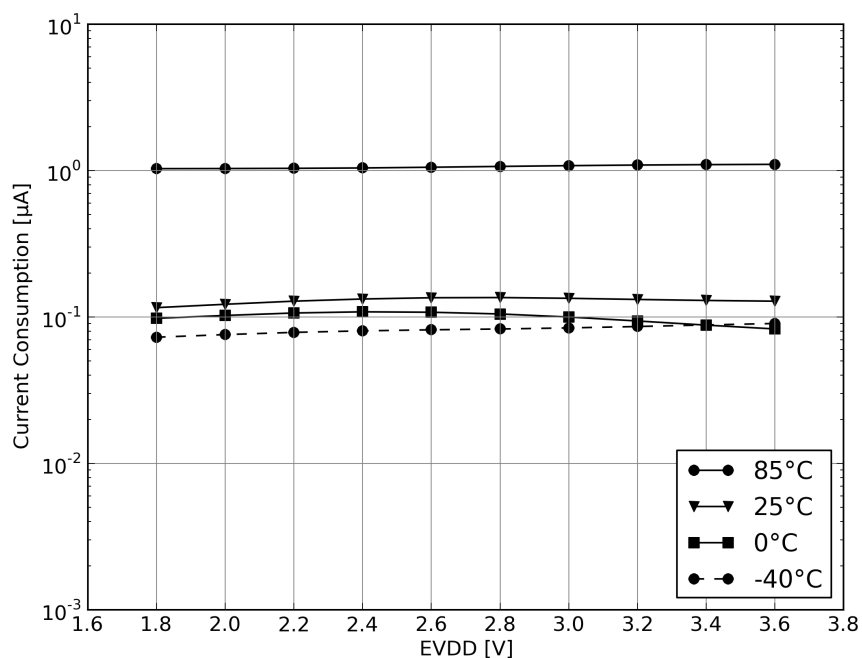
Figure 13-11. Current Consumption in SLEEP.
