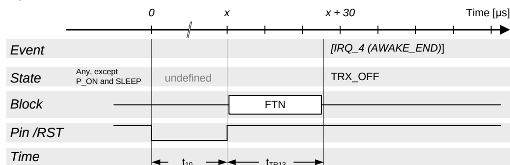
Figure 7-7. Reset Procedure.
