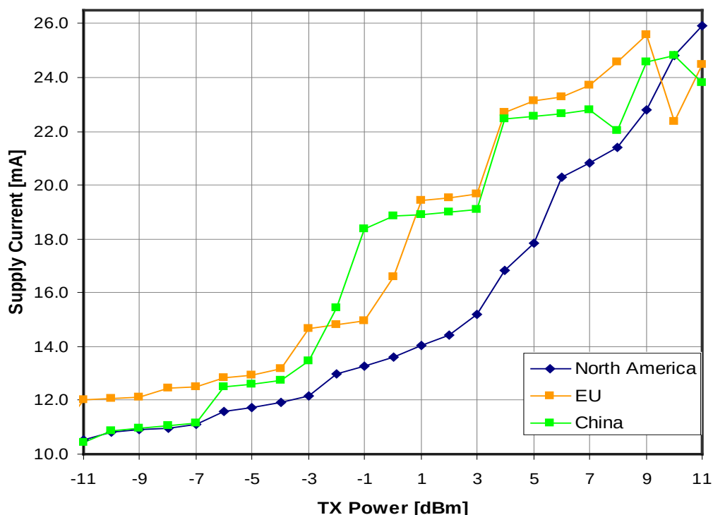
Figure 9-16. Supply Currents for O-QPSK Modulation depending on TX Power Setting (according to Table 9-15).
