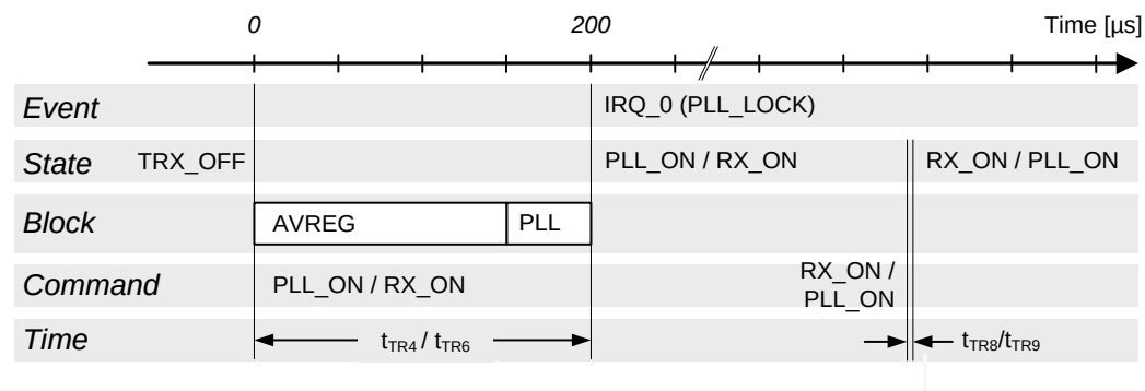
Figure 7-5. Transition from TRX_OFF to PLL_ON/RX_ON State and further to RX_ON/PLL_ON.
