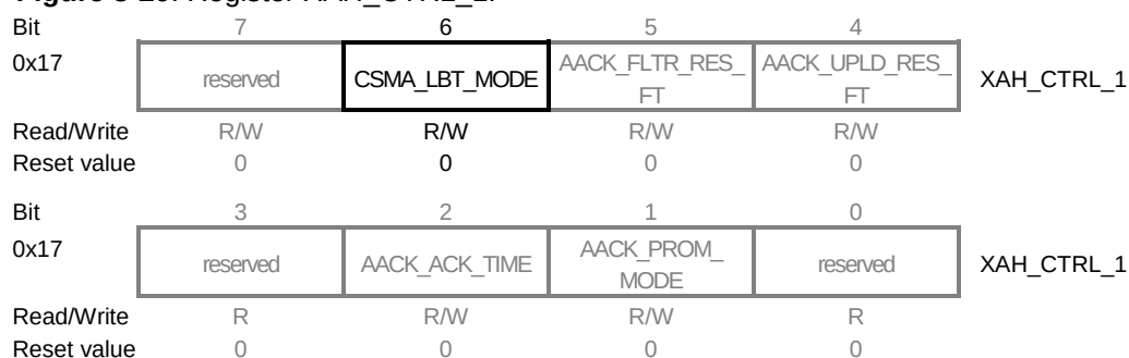
Figure 8-29. Register XAH_CTRL_1.
