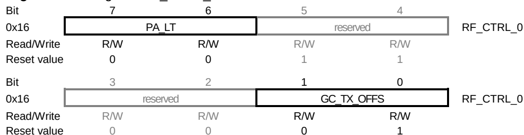
Figure 9-15. Register RF_CTRL_0.
