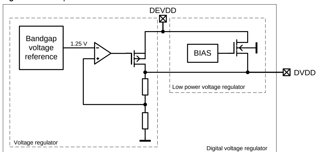
Figure 9-19. Simplified Schematic of DVREG.
