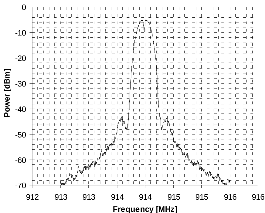
Figure 9-6. Spectrum of BPSK-20.
