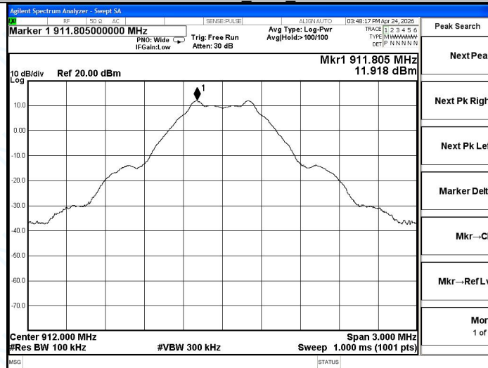
Z-Wave Ant1 912
