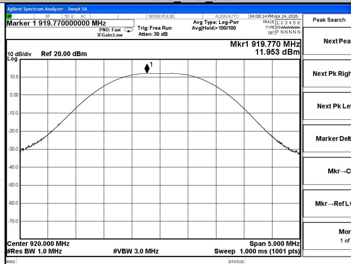
Z-Wave Ant1_920
