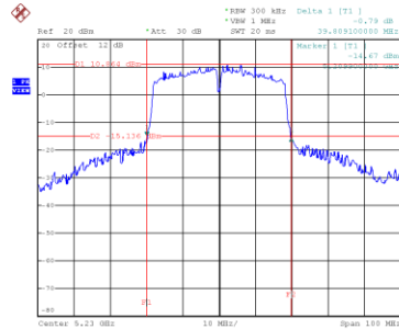
26 dB Bandwidth
