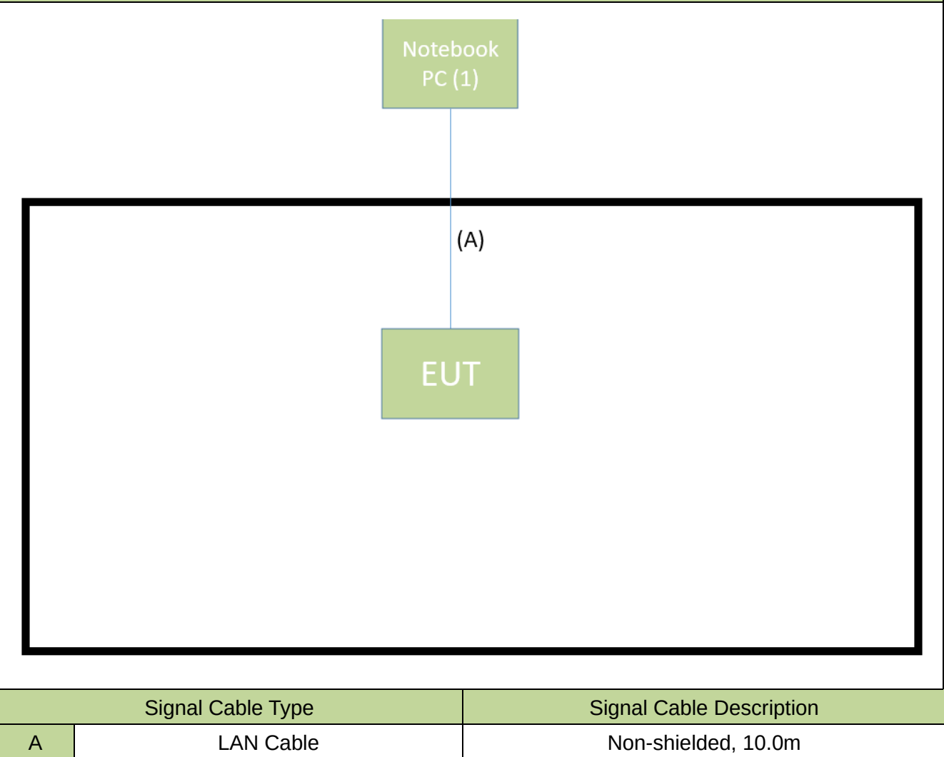
Connection Diagram
