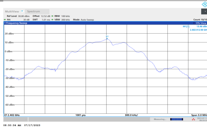
BLE_125 kbps_Ant1_2402_0~Reference
