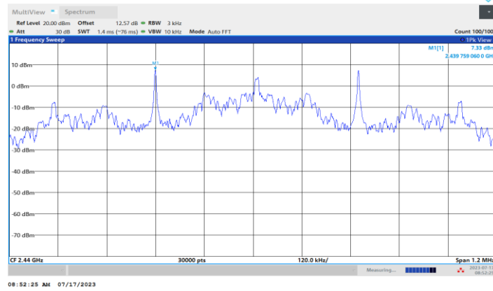
BLE_125 kbps_Ant1_2440
