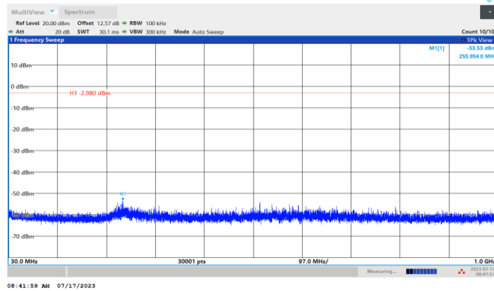
BLE_1 Mbps_Ant1_2440_30~1000
