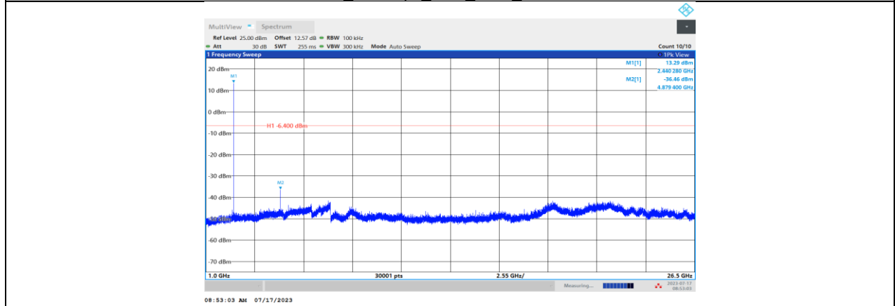
BLE_125 kbps_Ant1_2440_1000~26500
