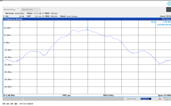
BLE_1 Mbps_Ant1_2480_0~Reference
