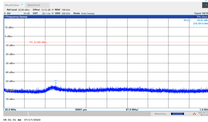
BLE_125 kbps_Ant1_2402_30~1000
