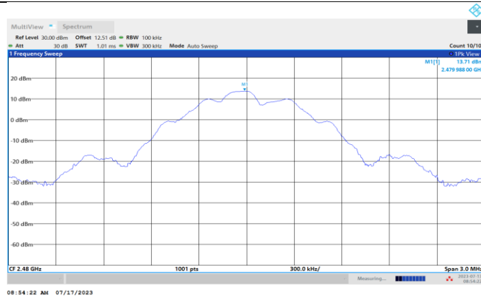
BLE_125 kbps_Ant1_2480_0~Reference
