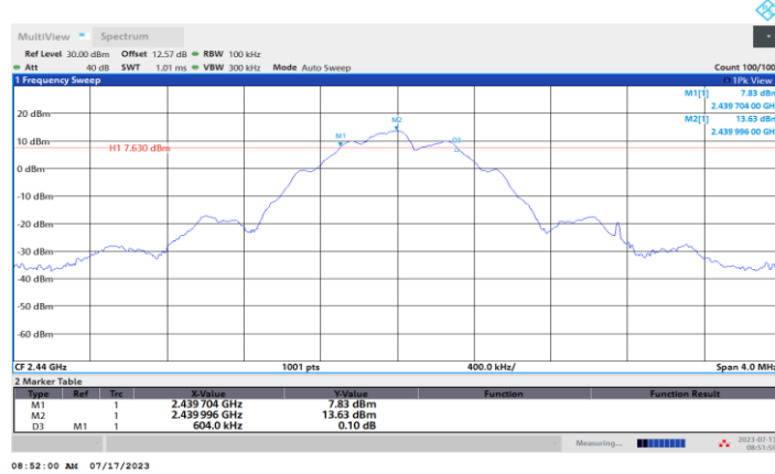
BLE_125 kbps_Ant1_2440
