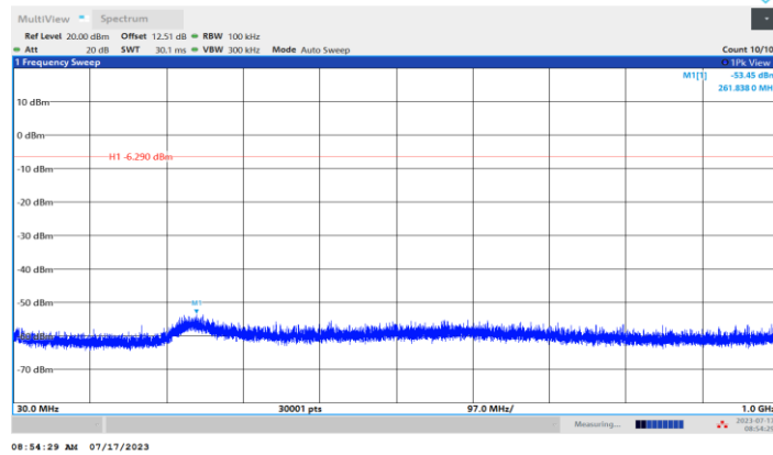
BLE_125 kbps_Ant1_2480_30~1000
