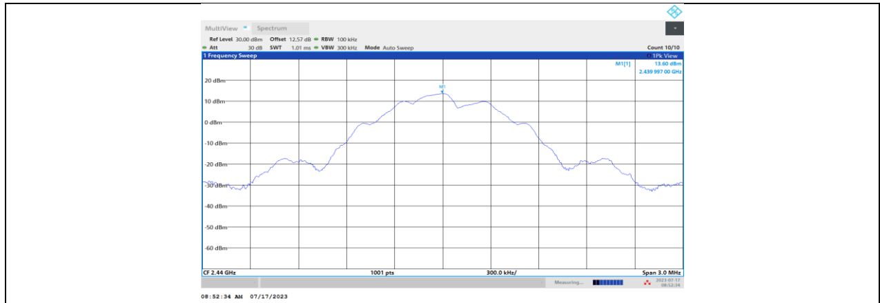
BLE_125 kbps_Ant1_2440_0~Reference
