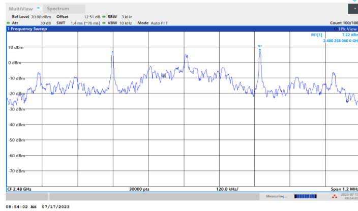
BLE_125 kbps_Ant1_2480
