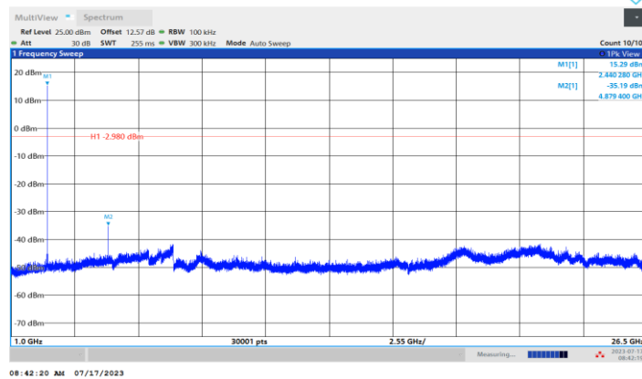
BLE_1 Mbps_Ant1_2440_1000~26500
