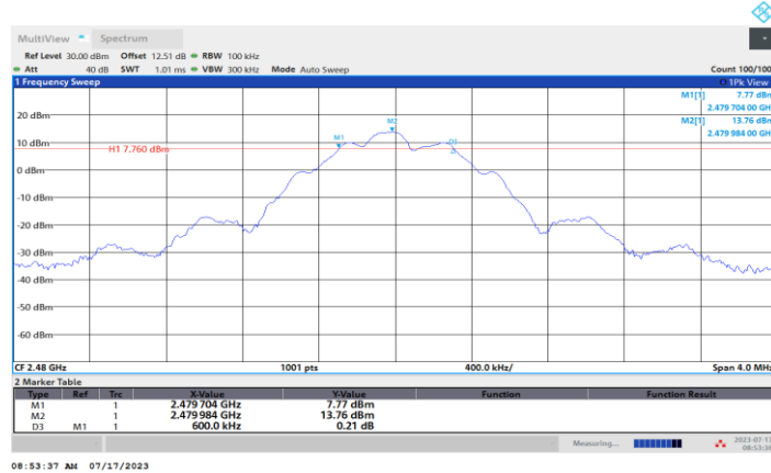
BLE_125 kbps_Ant1_2480
