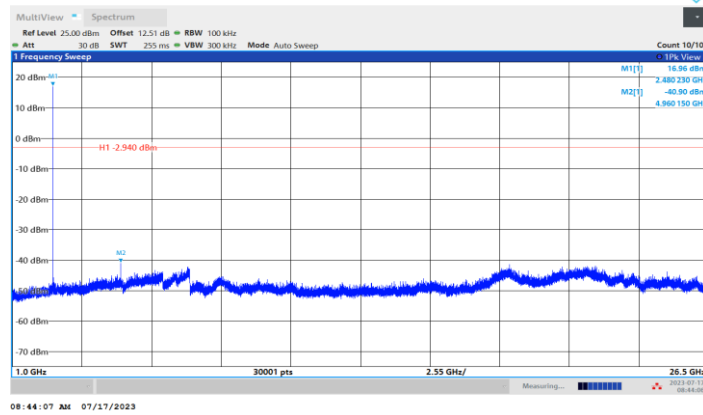
BLE_1 Mbps_Ant1_2480_1000~26500
