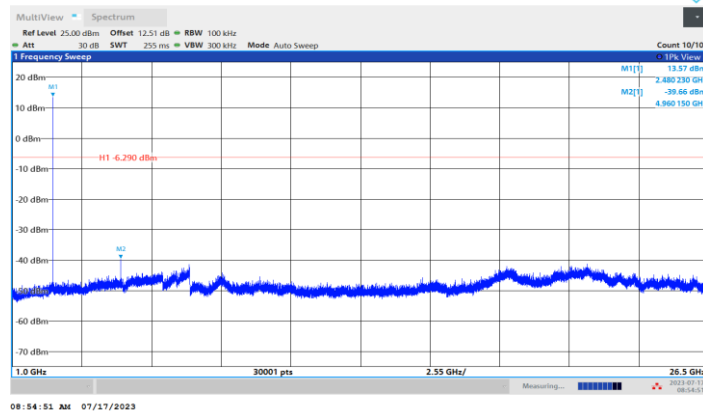
BLE_125 kbps_Ant1_2480_1000~26500
