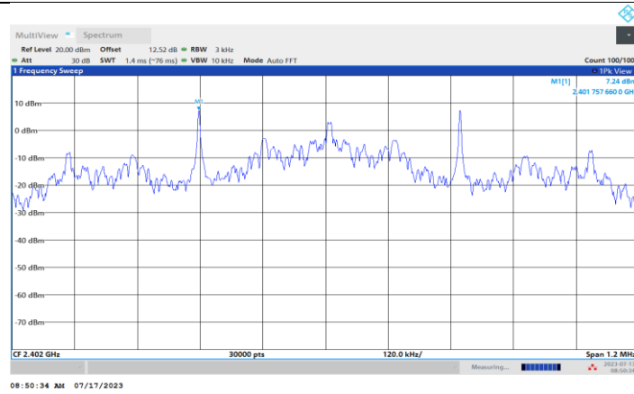
BLE_125 kbps_Ant1_2402
