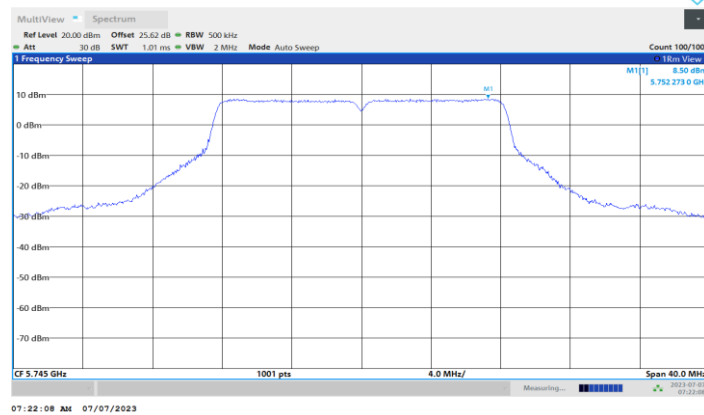
11A-CDD_Ant4_5745
