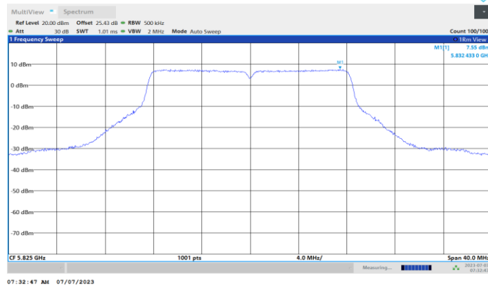
11A-CDD_Ant4_5825
