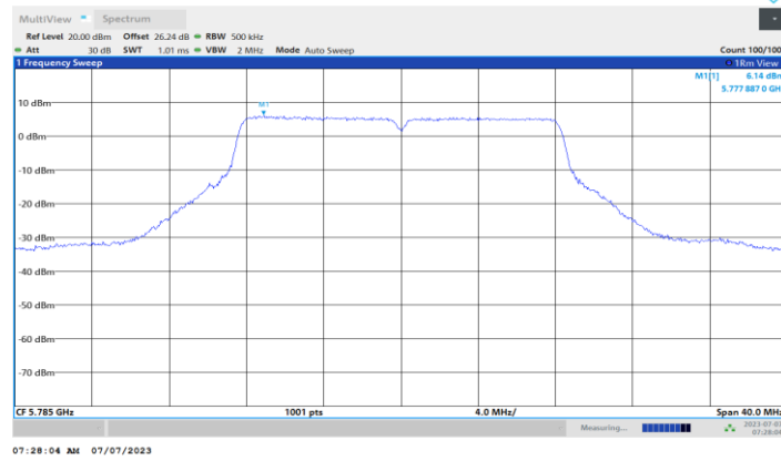
11A-CDD_Ant2_5785
