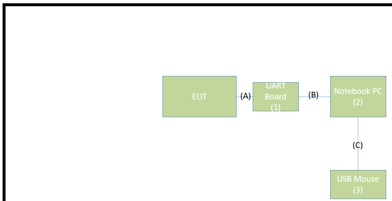
Connection Diagram – Mode1~13
