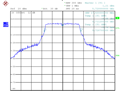
CH144 99 % Occupied Bandwidth
