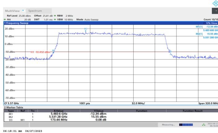
11AX160-CDD_Ant5_5570
