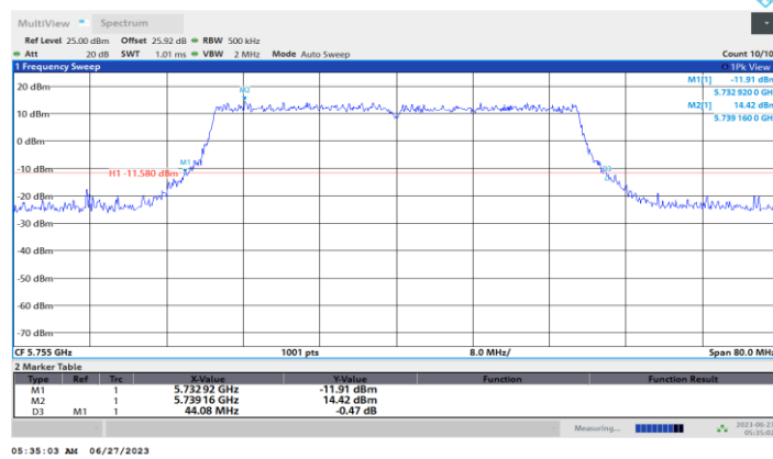
11AX40-CDD_Ant5_5755
