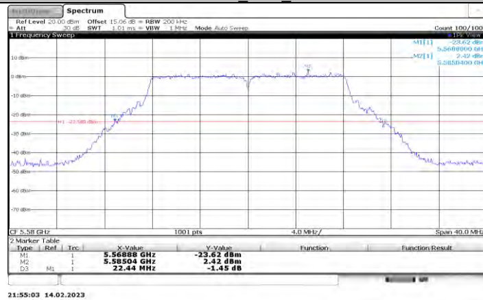
11A-CDD_Ant4_5580
