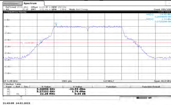
11A-CDD_Ant4_5280
