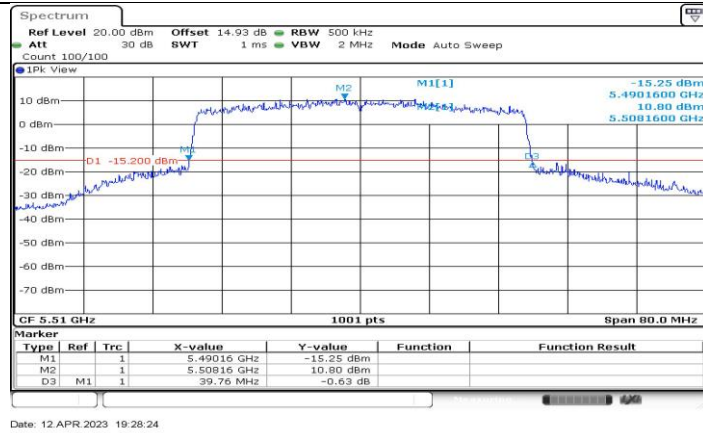
11AX40-CDD_Ant3_5510
