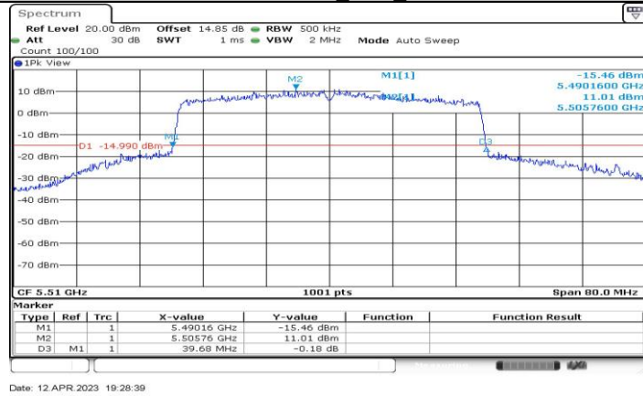
11AX40-CDD_Ant4_5510
