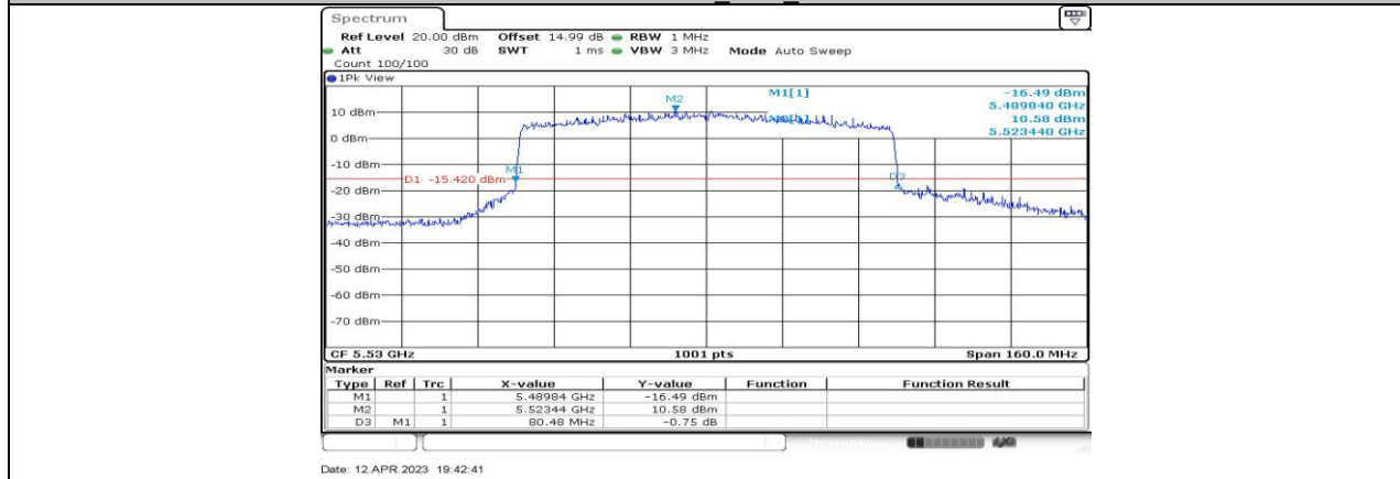
11AX80-CDD_Ant3_5530
