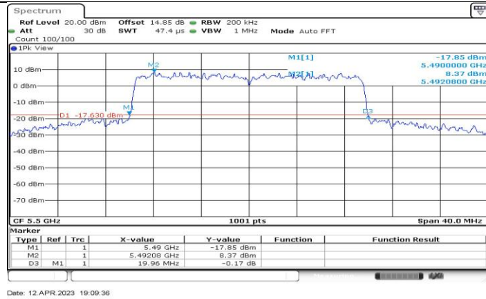
11AX20-CDD_Ant4_5500
