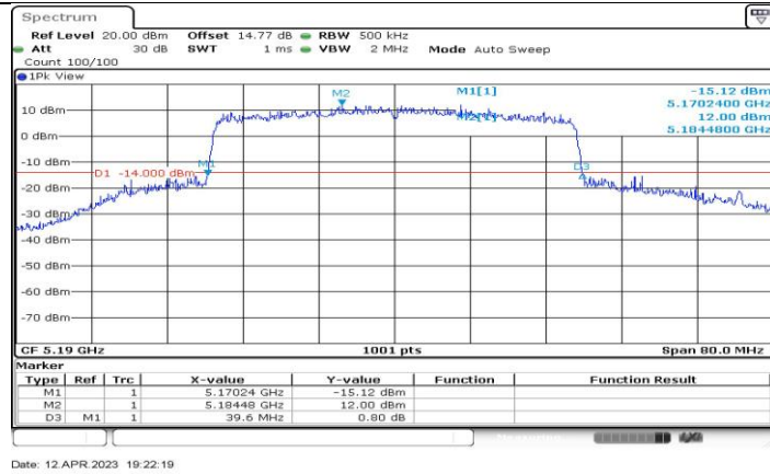
11AX40-CDD_Ant4_5190
