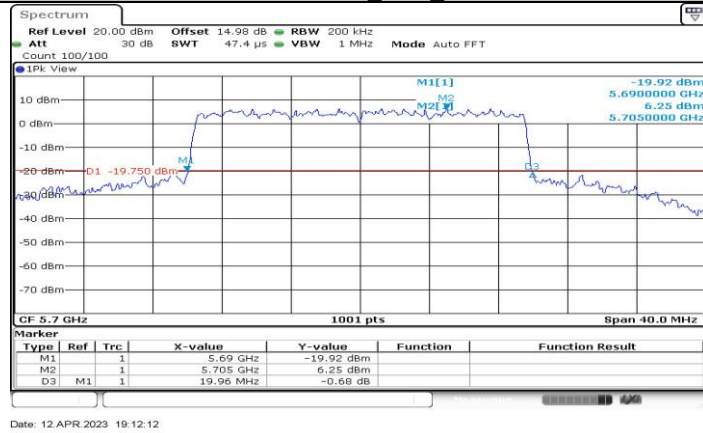
11AX20-CDD_Ant3_5700
