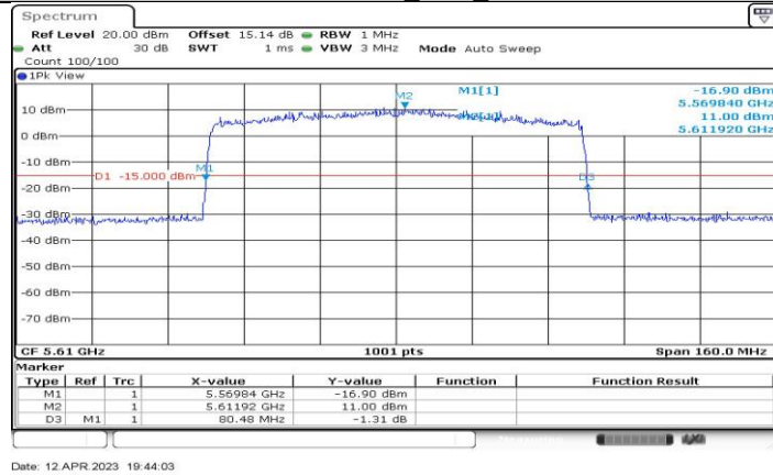
11AX80-CDD_Ant3_5610
