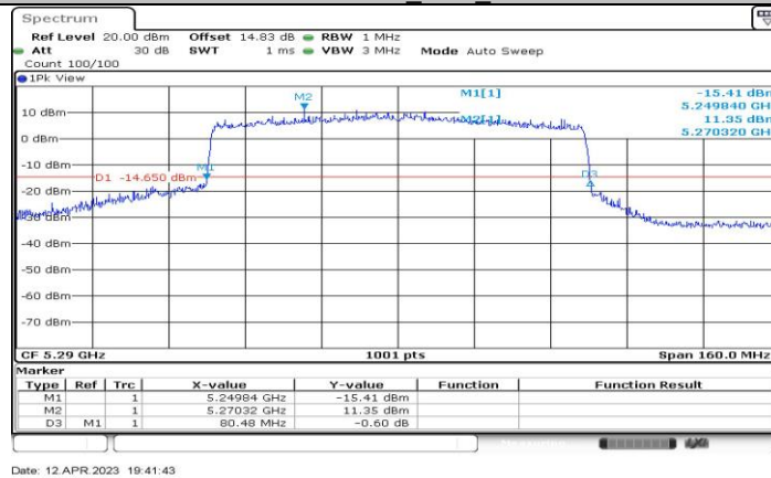
11AX80-CDD_Ant4_5290
