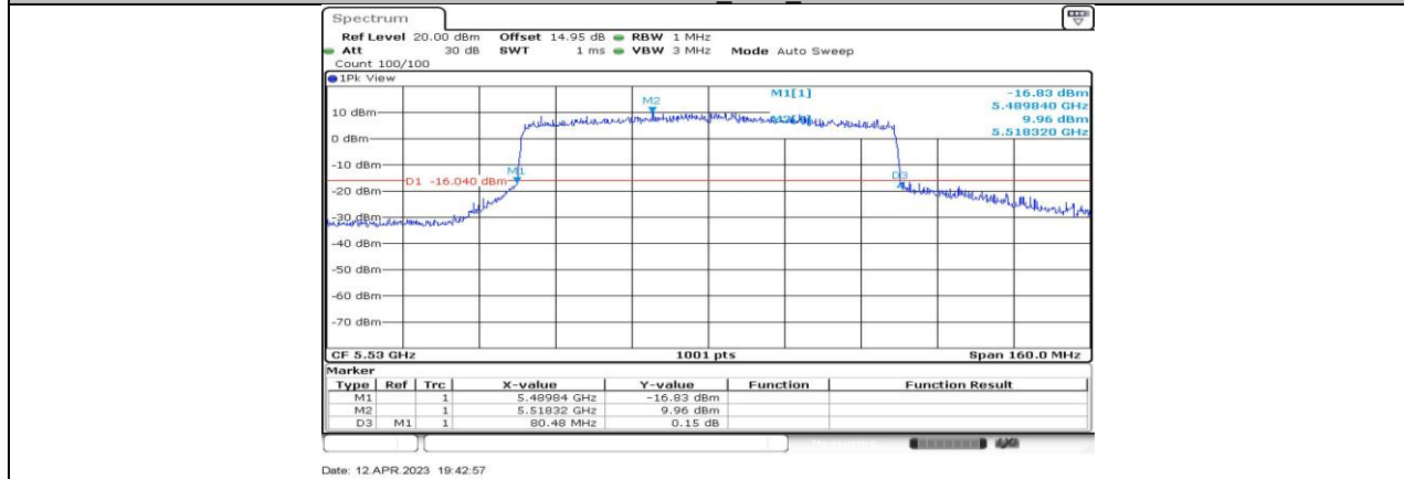
11AX80-CDD_Ant4_5530
