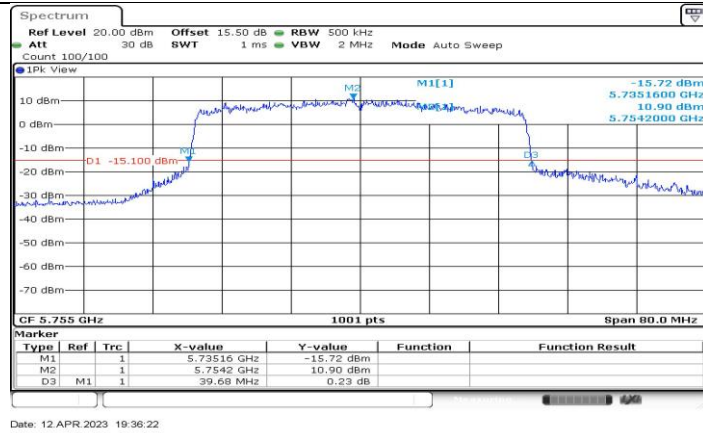
11AX40-CDD_Ant3_5755
