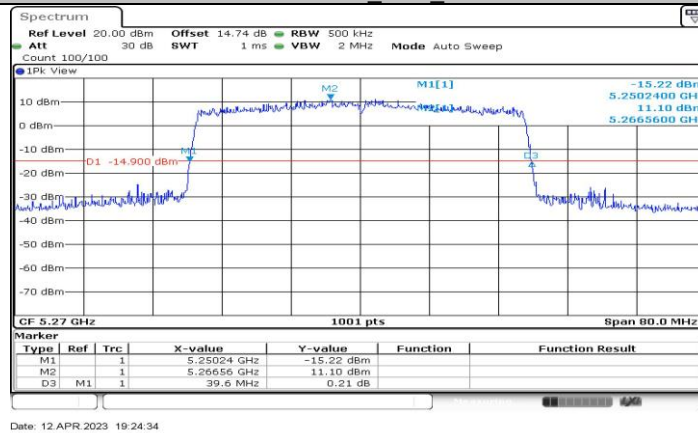
11AX40-CDD_Ant3_5270
