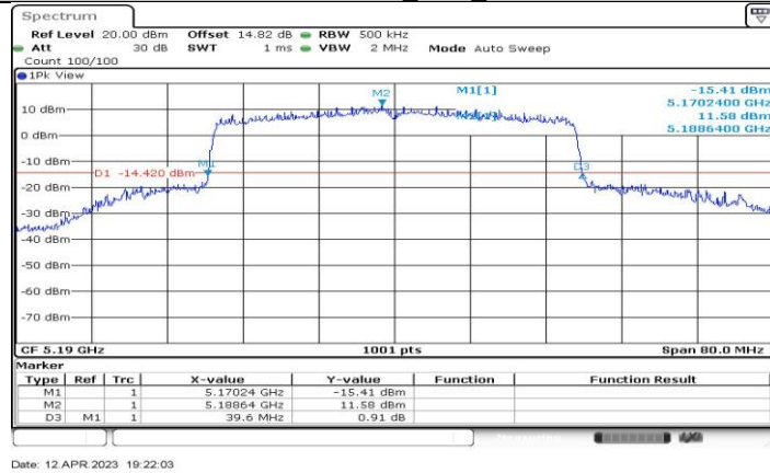
11AX40-CDD_Ant3_5190
