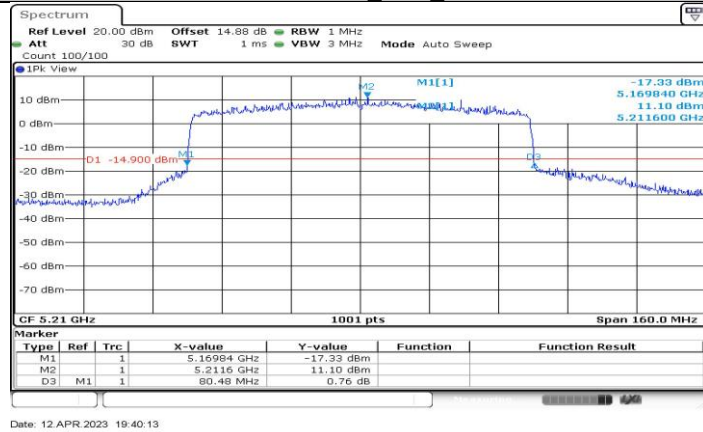
11AX80-CDD_Ant3_5210
