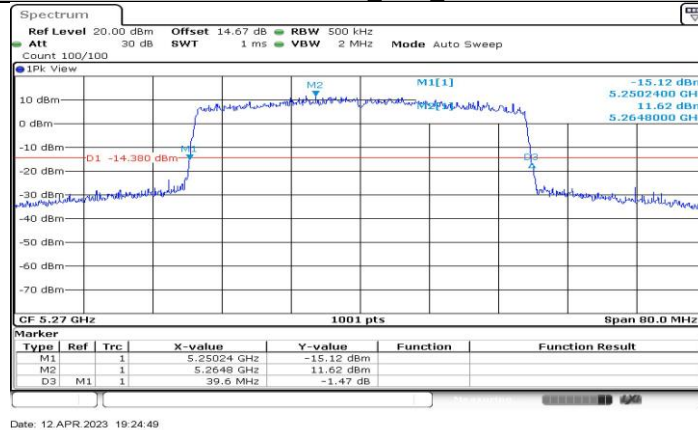
11AX40-CDD_Ant4_5270
