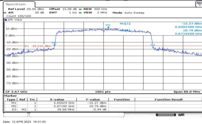
11AX40-CDD_Ant3_5670
