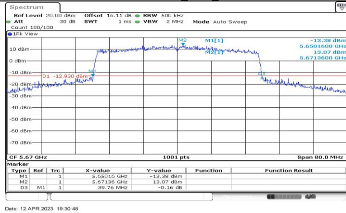
11AX40-CDD_Ant2_5670
