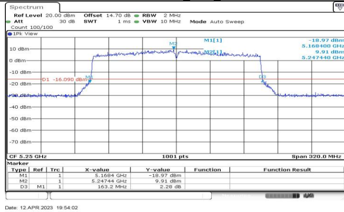
11AX160-CDD_Ant3_5250
