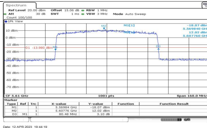
11AX80-CDD_Ant4_5610
