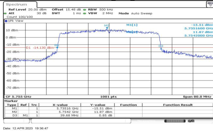
11AX40-CDD_Ant4_5755
