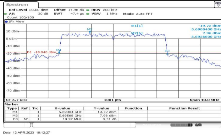
11AX20-CDD_Ant4_5700
