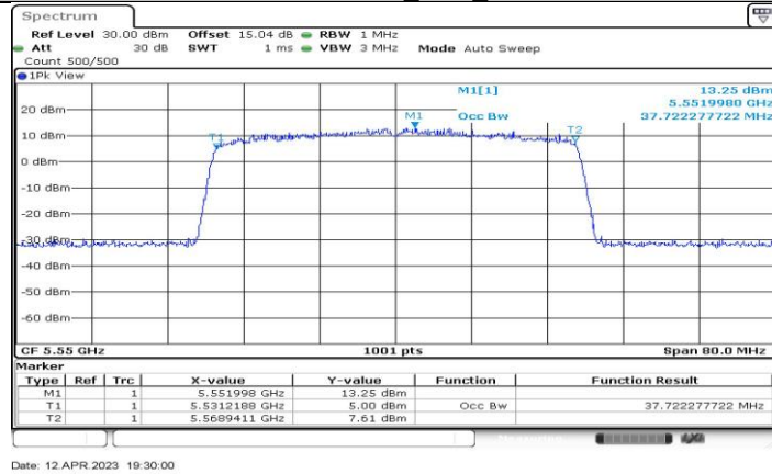
11AX40-CDD_Ant4_5550
