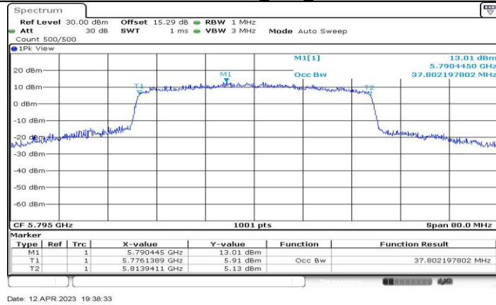
11AX40-CDD_Ant3_5795
