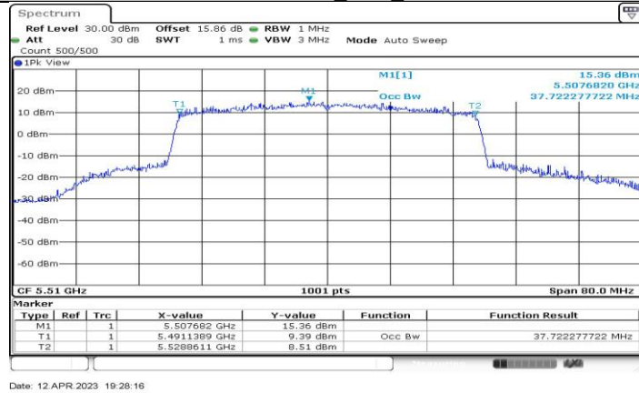
11AX40-CDD_Ant2_5510
