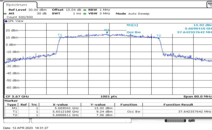
11AX40-CDD_Ant4_5670
