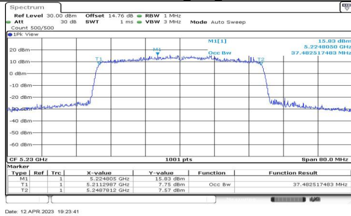
11AX40-CDD_Ant4_5230
