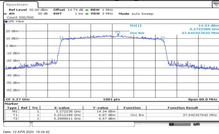
11AX40-CDD_Ant3_5270
