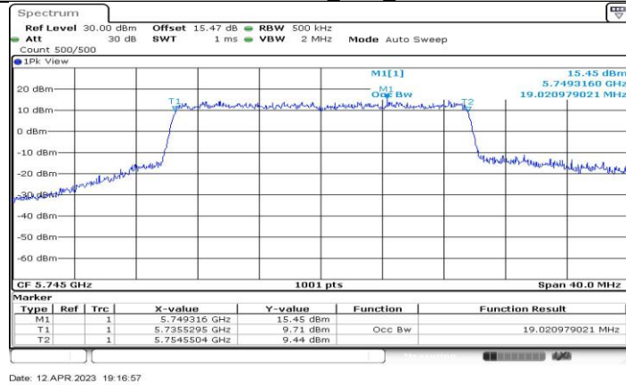
11AX20-CDD_Ant3_5745
