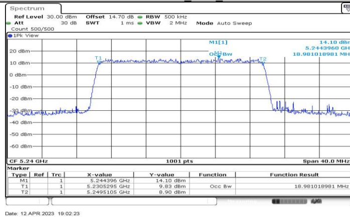
11AX20-CDD_Ant3_5240
