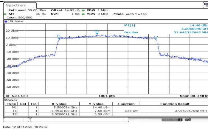
11AX40-CDD_Ant3_5510
