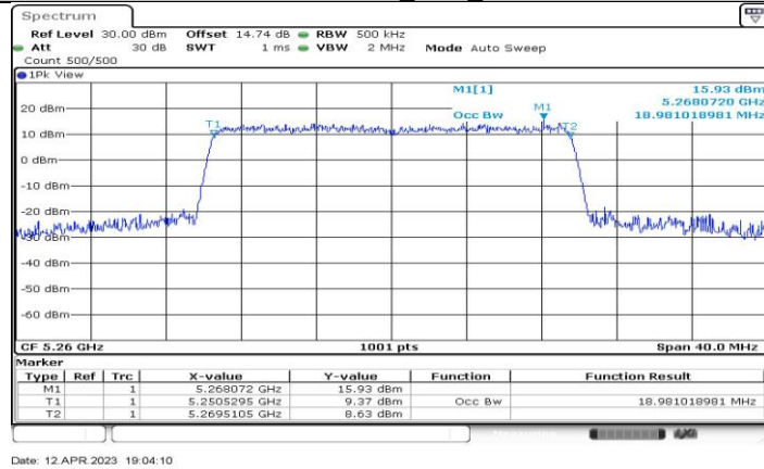
11AX20-CDD_Ant3_5260
