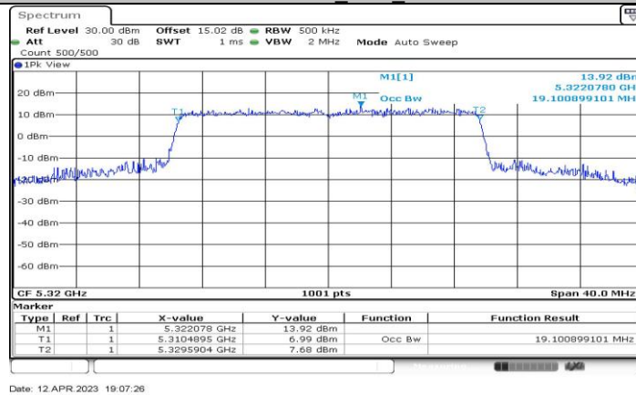
11AX20-CDD_Ant3_5320
