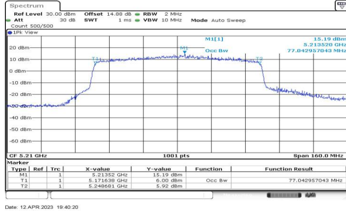
11AX80-CDD_Ant3_5210
