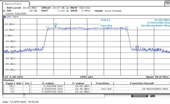
11AX20-CDD_Ant4_5260
