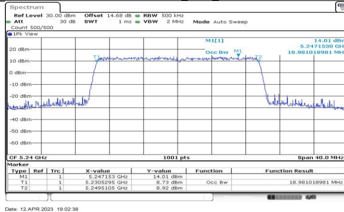
11AX20-CDD_Ant4_5240
