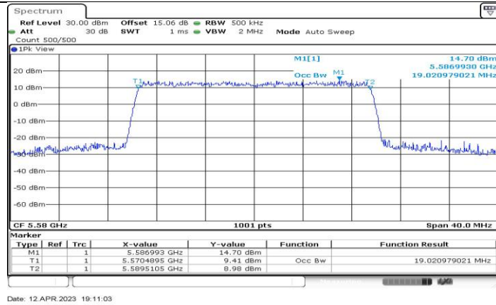
11AX20-CDD_Ant3_5580
