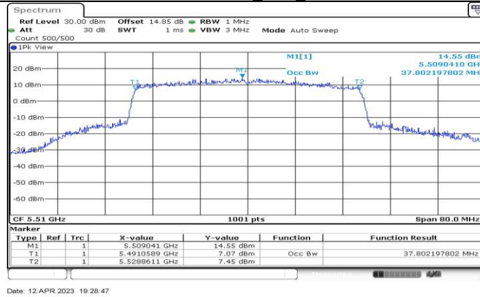
11AX40-CDD_Ant4_5510
