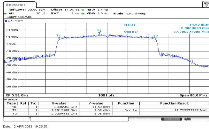
11AX40-CDD_Ant4_5310
