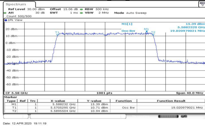
11AX20-CDD_Ant4_5580
