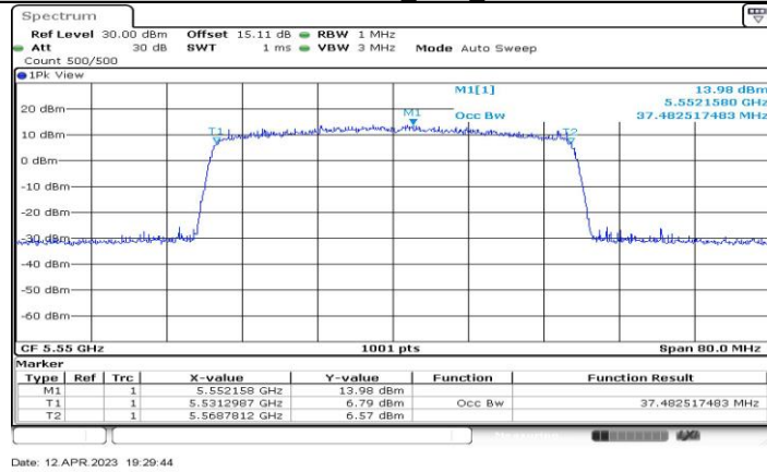
11AX40-CDD_Ant3_5550
