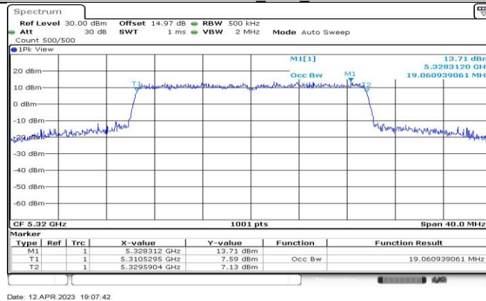
11AX20-CDD_Ant4_5320
