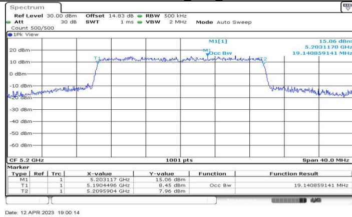
11AX20-CDD_Ant4_5200
