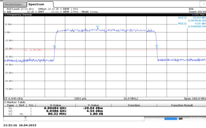
11BE80-CDD_Ant3_6945
