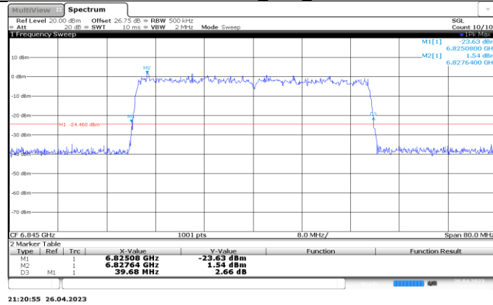
11BE40-CDD_Ant4_6845
