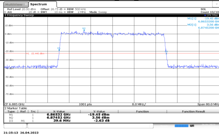
11BE40-CDD_Ant2_6885
