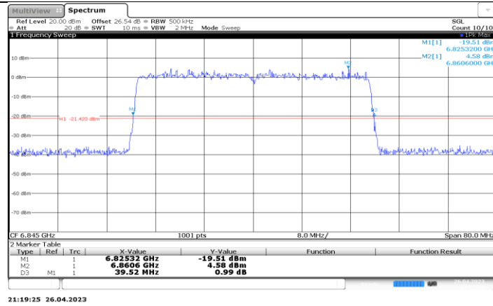
11BE40-CDD_Ant2_6845
