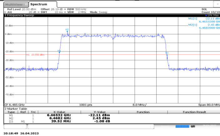
11BE40-CDD_Ant4_6485
