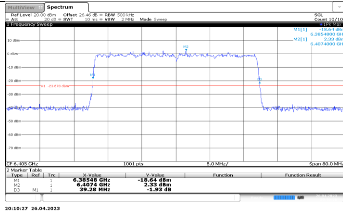
11BE40-CDD_Ant4_6405
