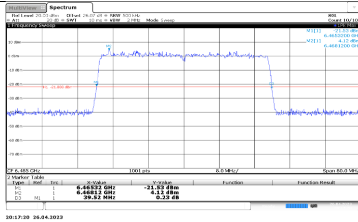
11BE40-CDD_Ant2_6485
