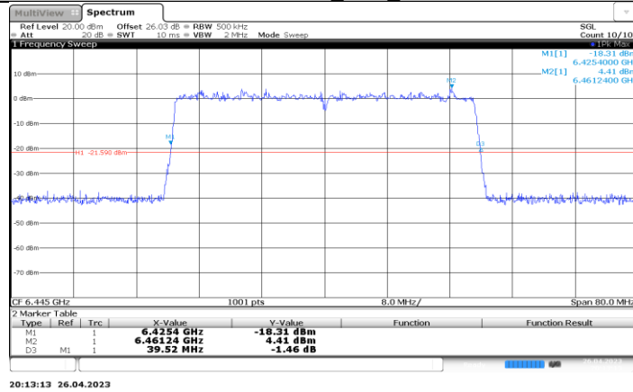
11BE40-CDD_Ant2_6445
