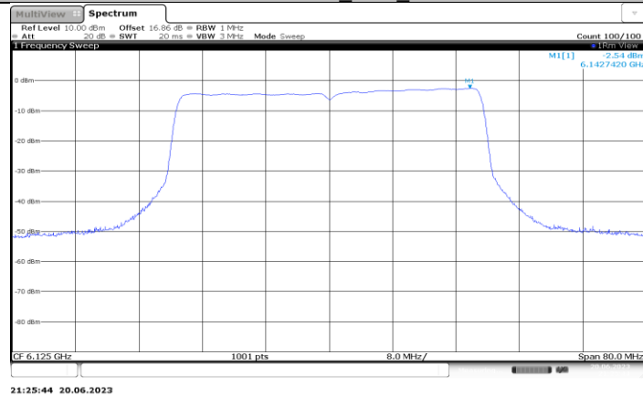
11BE40MIMO_Ant5_6125
