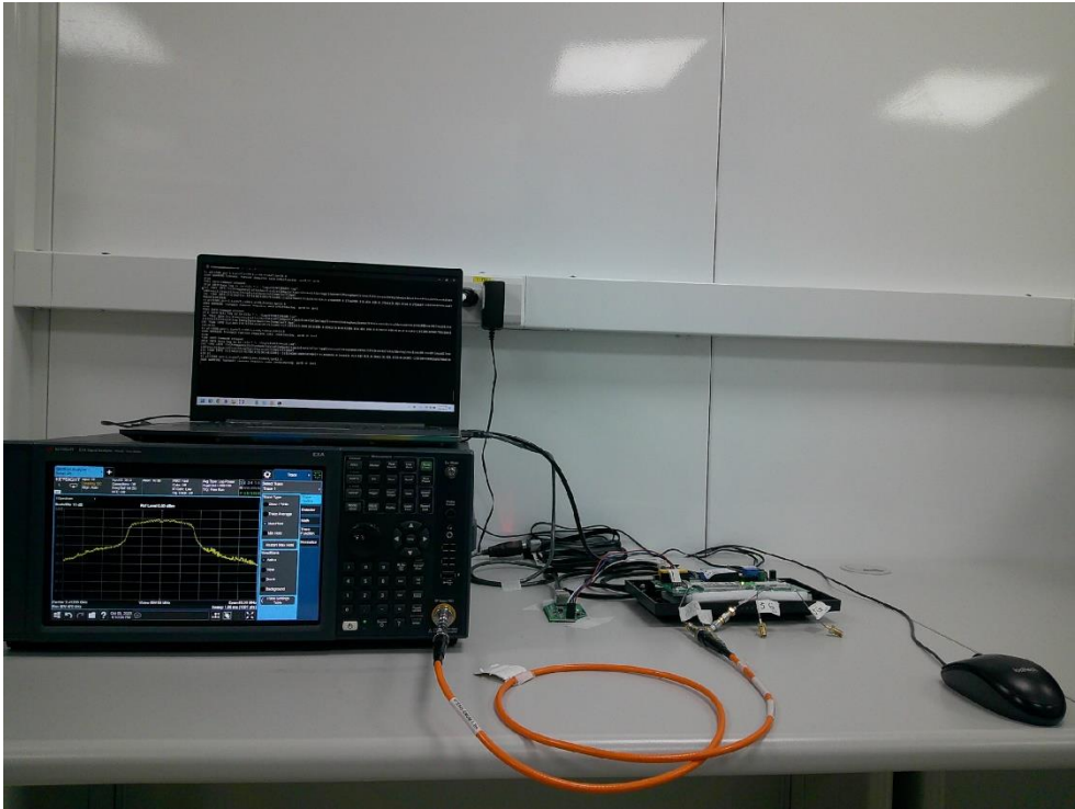
Description: Conducted Test Setup – 5G
